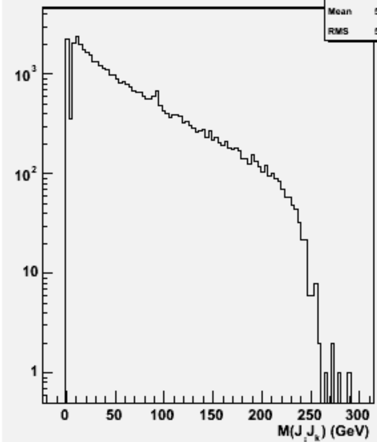
2jets mass(All comb)w103804 ae1_e1n3n3e1e1_o
