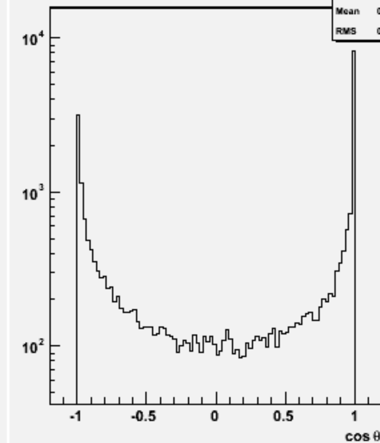
Jet cos \theta (All jets)w103804 ae1_e1n3n3e1e1_o
