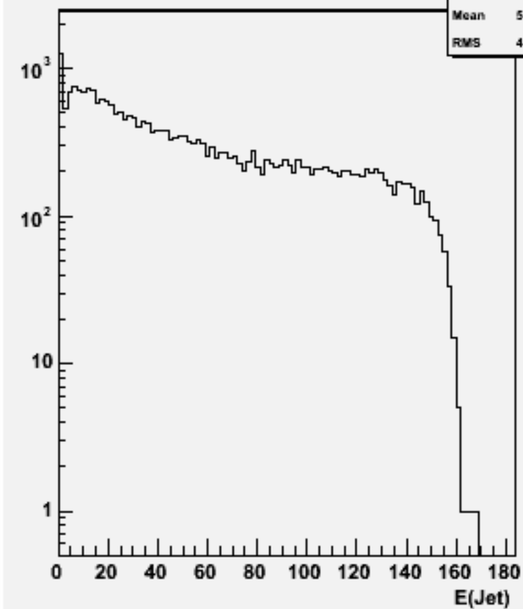
Jet energies(All jets)w103804 ae1_e1n3n3e1e1_o
