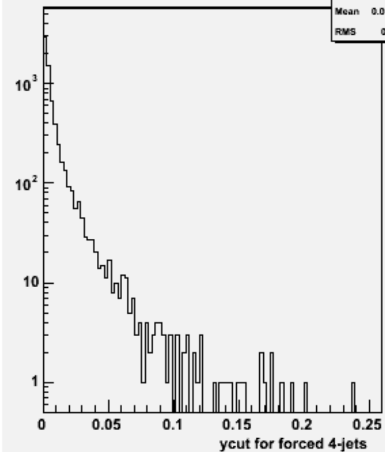
Ycut for 4-jets :w103804 ae1_e1n3n3e1e1_o
