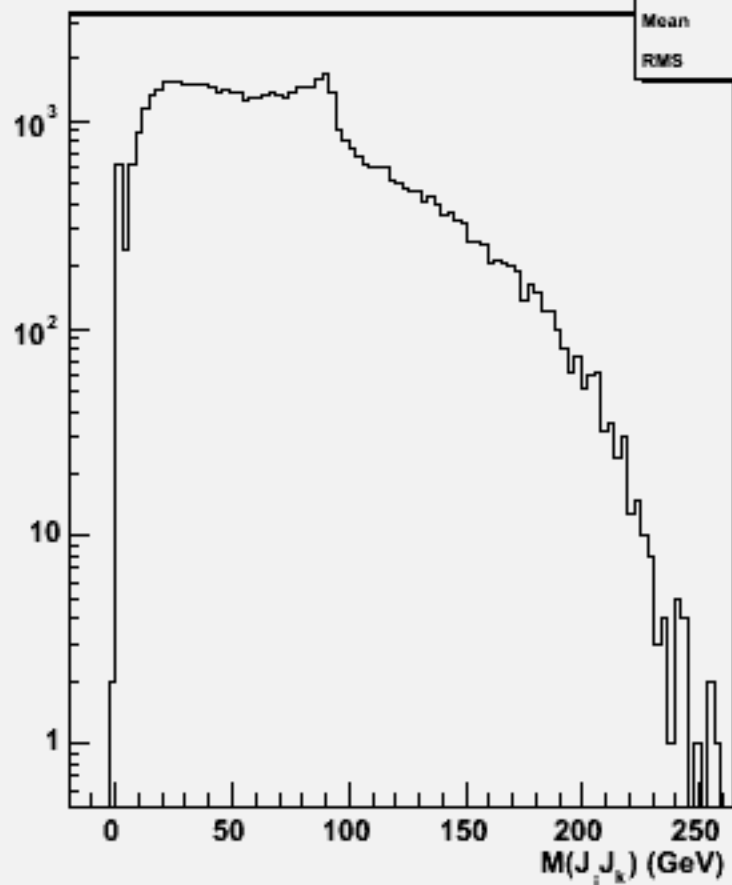
2jets mass(All comb)w103802 ae1_e1n2n2bb_o
