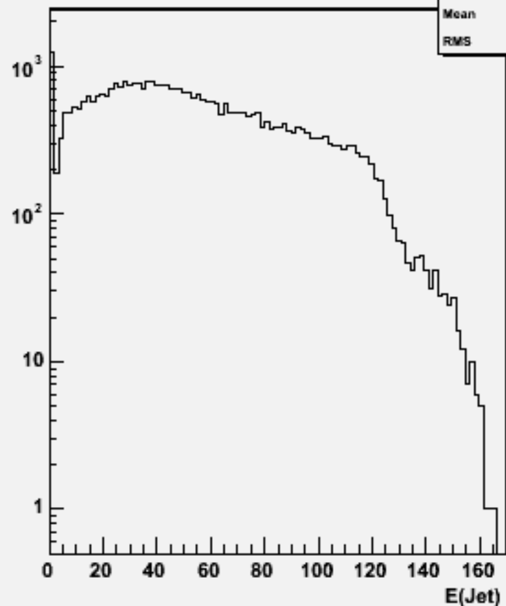
Jet energies(All jets)w103802 ae1_e1n2n2bb_o
