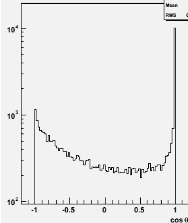
Jet cos \theta (All jets)w103802 ae1_e1n2n2bb_o
