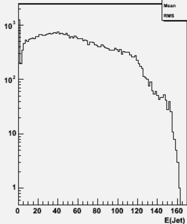
Jet energies(All jets)w103798 ae1_e1n2n2ss_o
