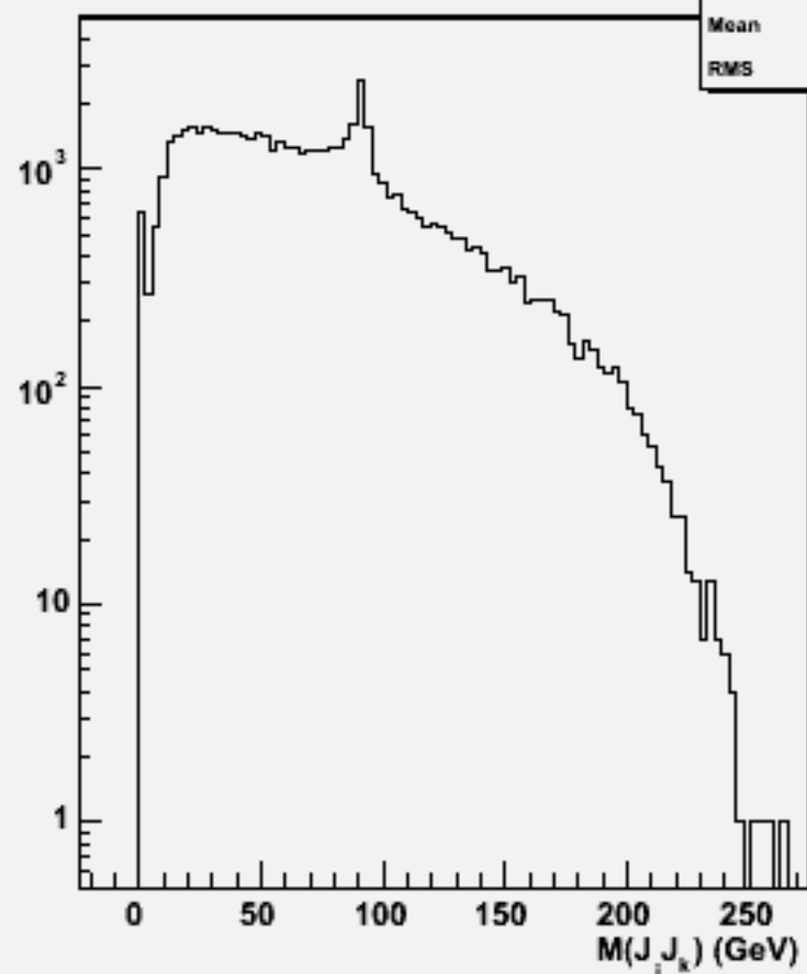
2jets mass(All comb)w103798 ae1_e1n2n2ss_o
