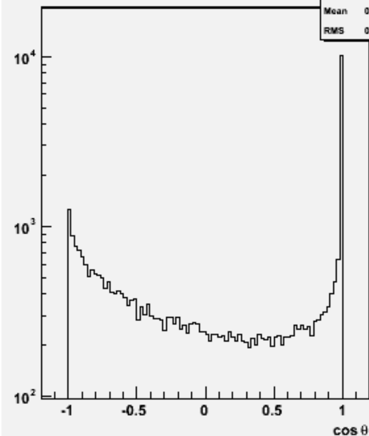
Jet cos \theta (All jets)w103798 ae1_e1n2n2ss_o
