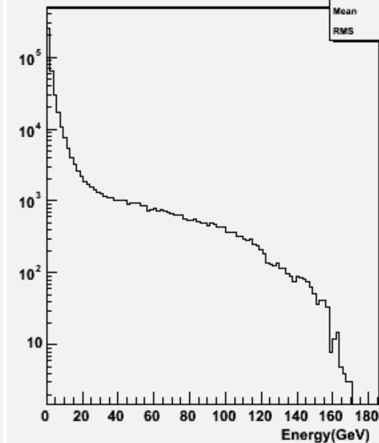
Particle Energy : w103794 ae1_e1n2n2dd_o
