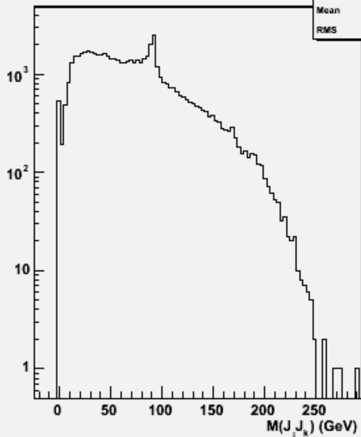
2jets mass(All comb)w103794 ae1_e1n2n2dd_o
