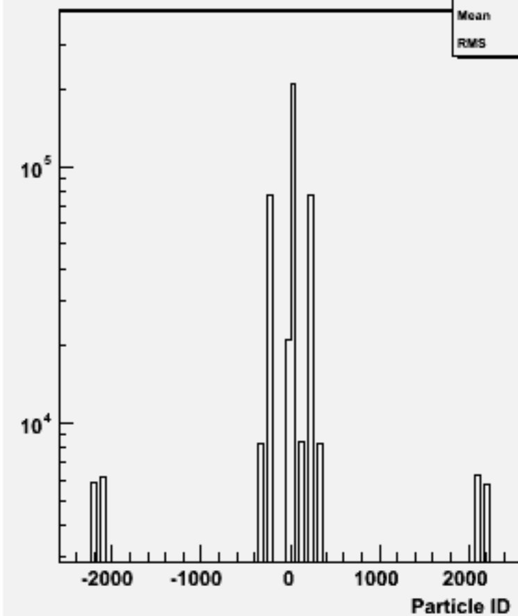
Particle ID : w103794 ae1_e1n2n2dd_o
