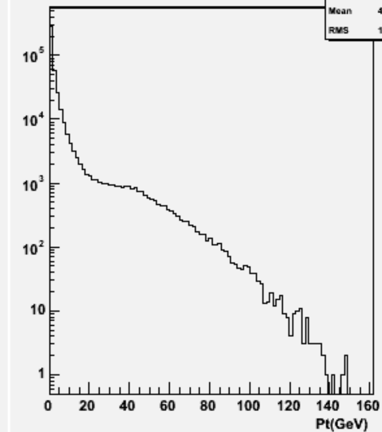
Particle Pt : w103794 ae1_e1n2n2dd_o
