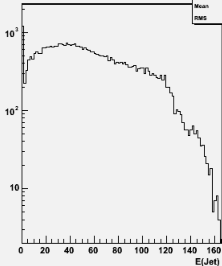
Jet energies(All jets)w103794 ae1_e1n2n2dd_o
