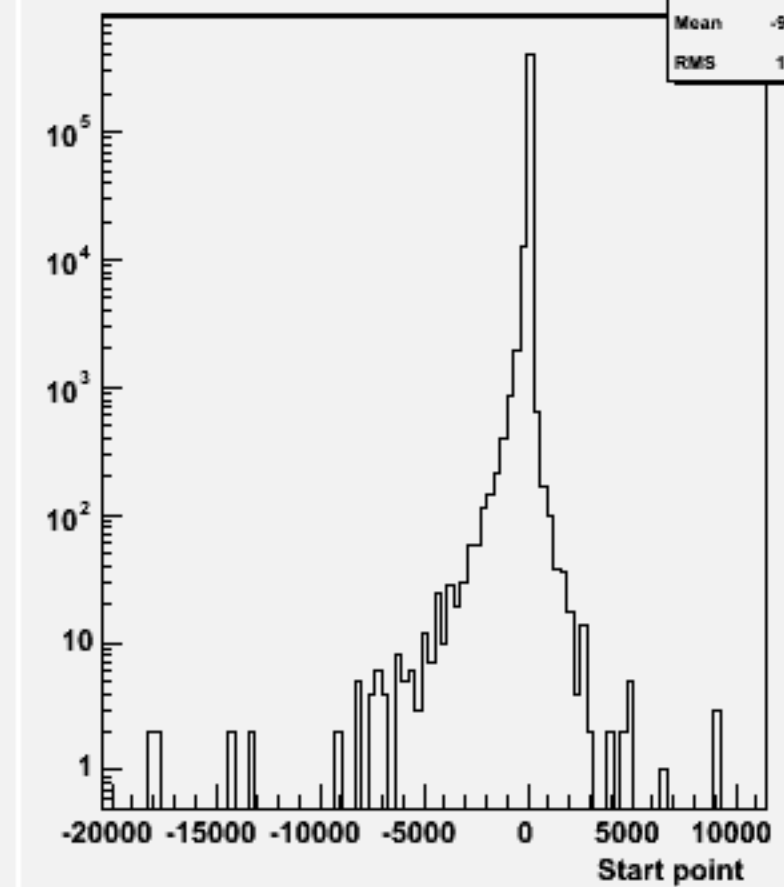
Start point Z : w103794 ae1_e1n2n2dd_o
