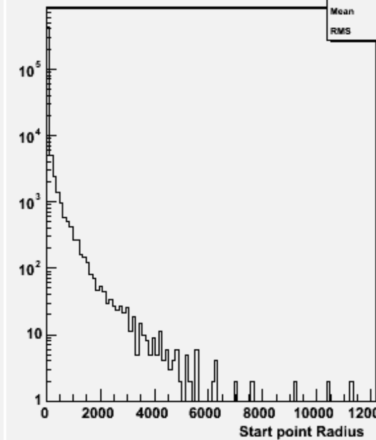
Start point R : w103794 ae1_e1n2n2dd_o
