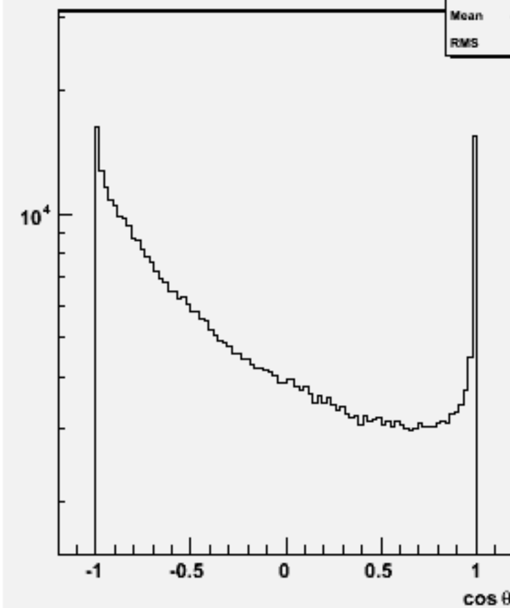
Particle cos \theta : w103794 ae1_e1n2n2dd_o
