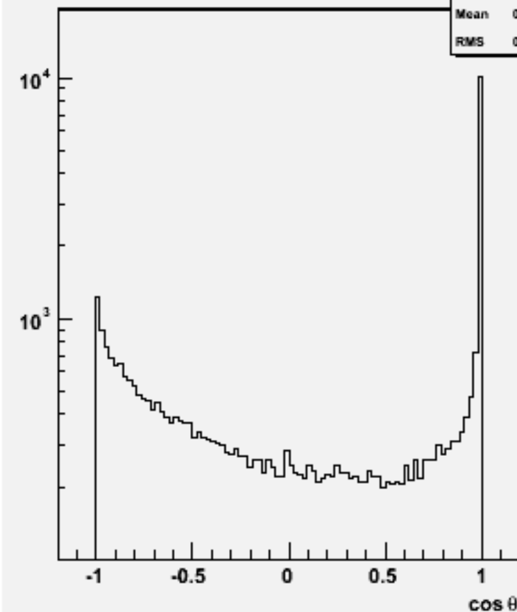
Jet cos \theta (All jets)w103794 ae1_e1n2n2dd_o
