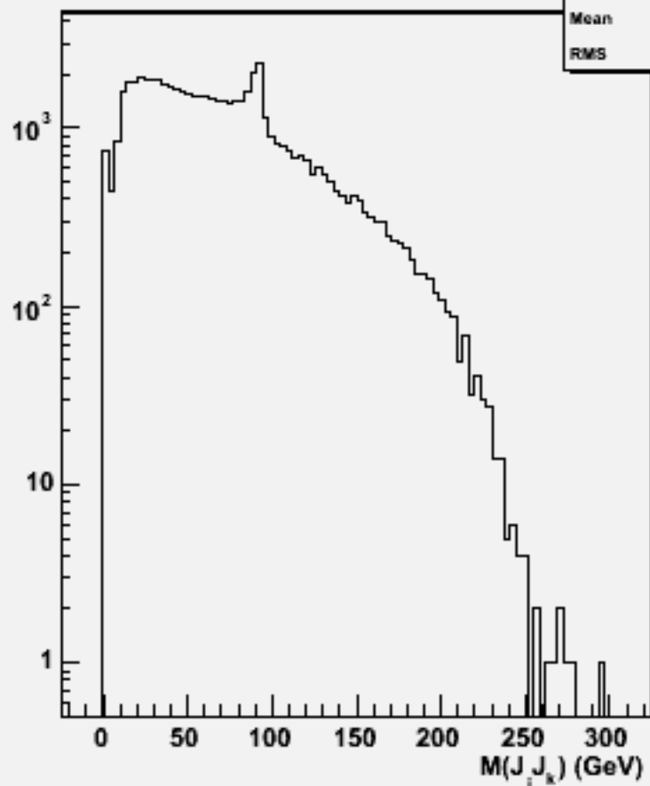
2jets mass(All comb)w103792 ae1_e1n2n2dd_o
