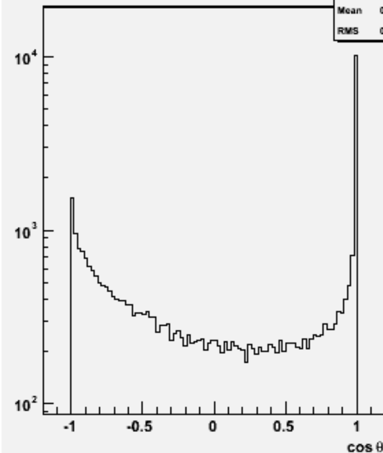
Jet cos \theta (All jets)w103792 ae1_e1n2n2dd_o
