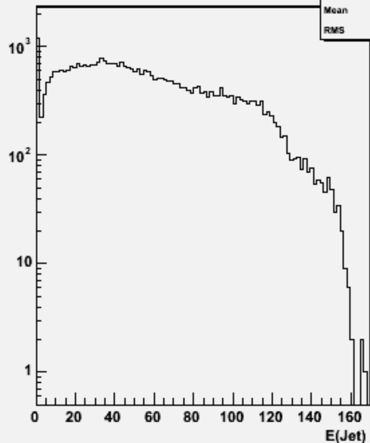
Jet energies(All jets)w103792 ae1_e1n2n2dd_o
