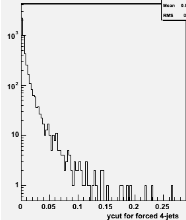
Ycut for 4-jets :w103790 ae1_e1n2n2e3e3_o
