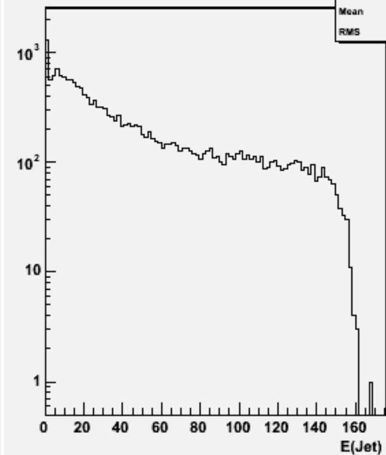
Jet energies(All jets)w103790 ae1_e1n2n2e3e3_o
