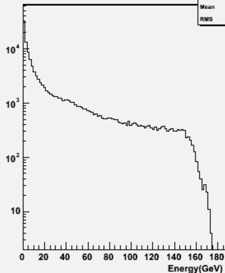
Start point R : w103790 ae1_e1n2n2e3e3_o
