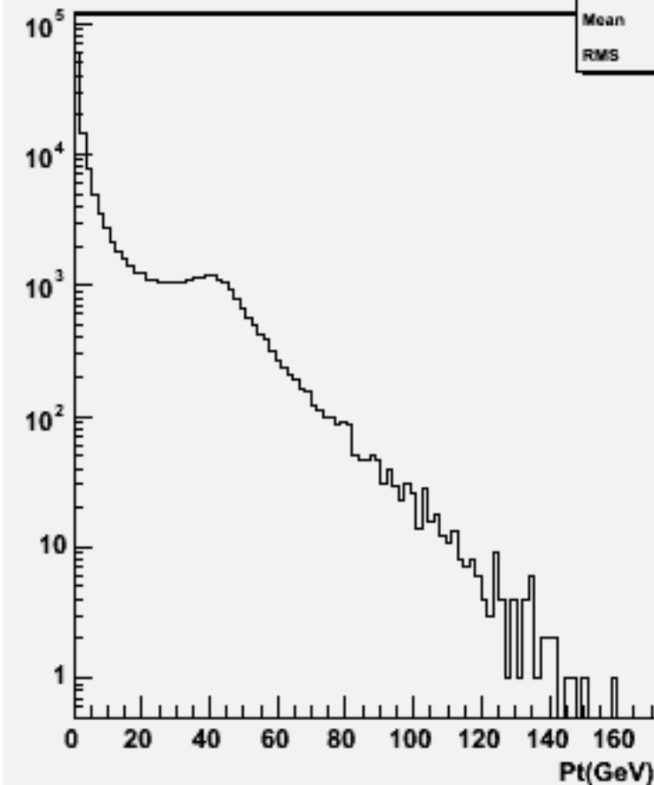
Start point Z : w103790 ae1_e1n2n2e3e3_o
