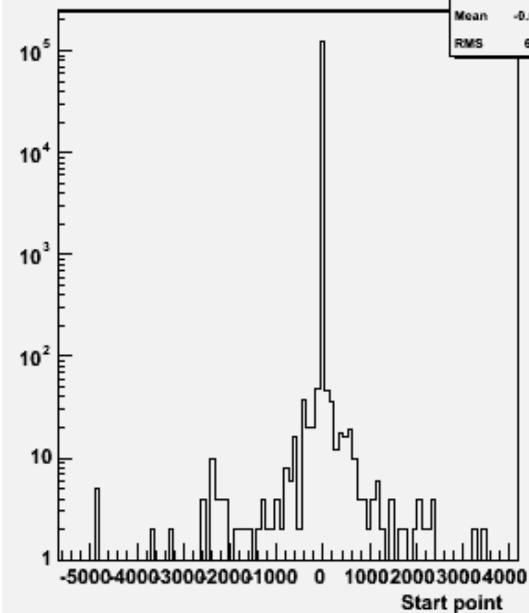
Start point Z : w103790 ae1_e1n2n2e3e3_o
