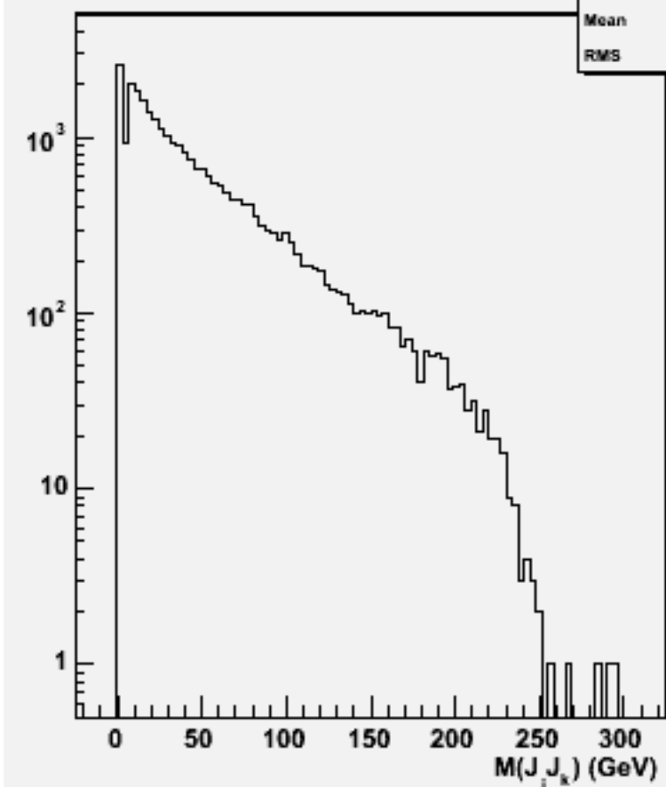
2jets mass(All comb)w103790 ae1_e1n2n2e3e3_o
