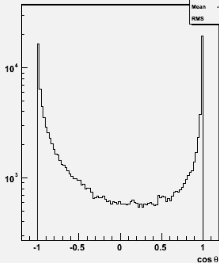
Particle cos \theta : w103790 ae1_e1n2n2e3e3_o
