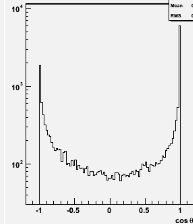
Jet cos \theta (All jets)w103790 ae1_e1n2n2e3e3_o
