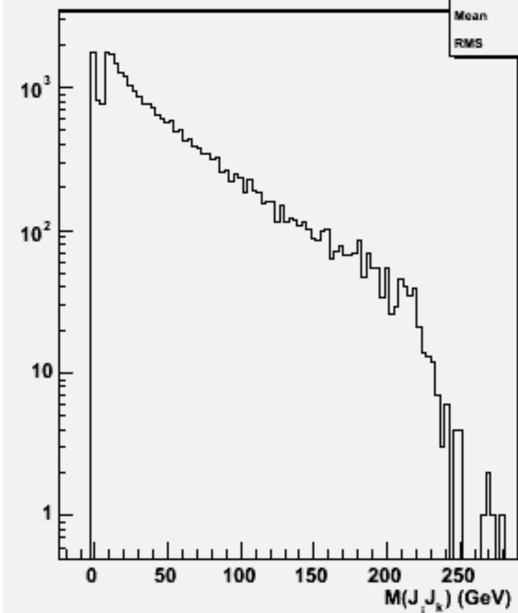
2jets mass(All comb)w103788 ae1_e1n2n2e3e3_o
