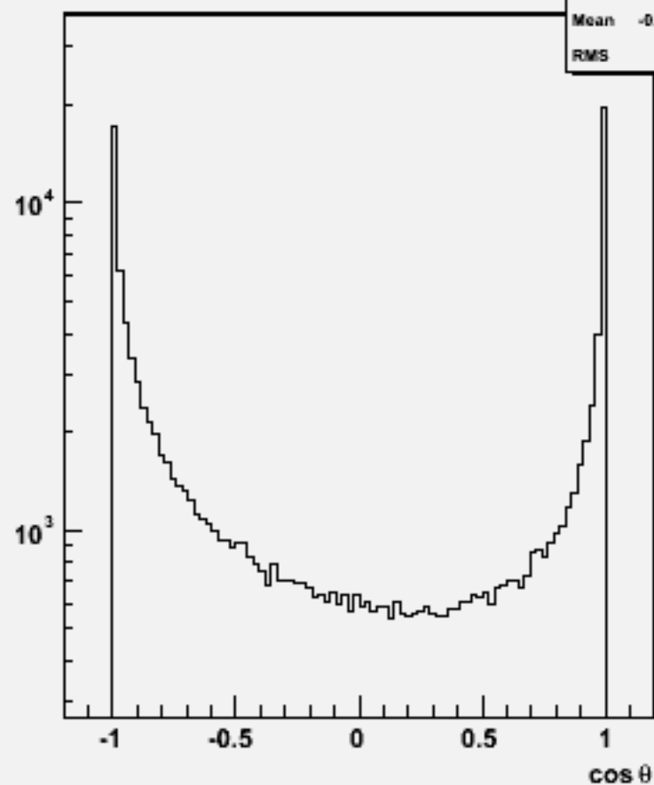
Particle cos \theta : w103788 ae1_e1n2n2e3e3_o
