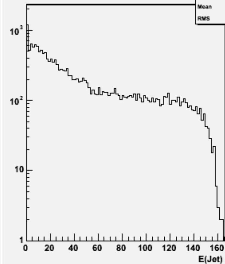
Jet energies(All jets)w103788 ae1_e1n2n2e3e3_o
