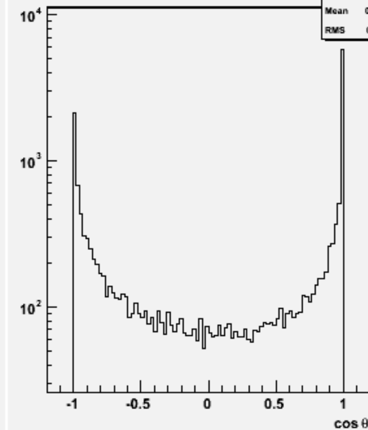
Jet cos \theta (All jets)w103788 ae1_e1n2n2e3e3_o
