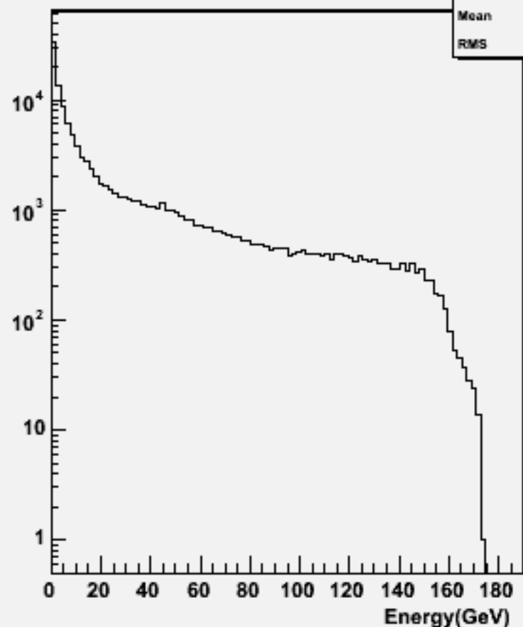
Particle Energy : w103788 ae1_e1n2n2e3e3_o
