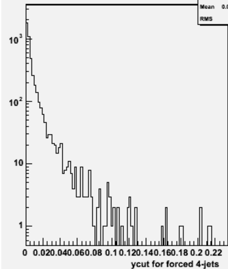
Ycut for 4-jets :w103788 ae1_e1n2n2e3e3_o
