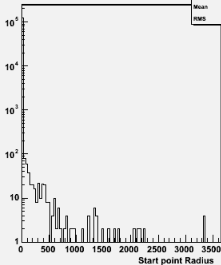
Start point R : w103788 ae1_e1n2n2e3e3_o
