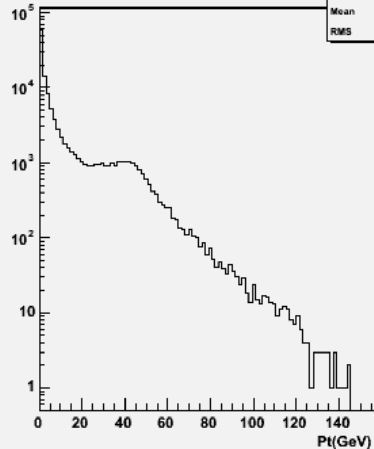
Particle Pt : w103788 ae1_e1n2n2e3e3_o
