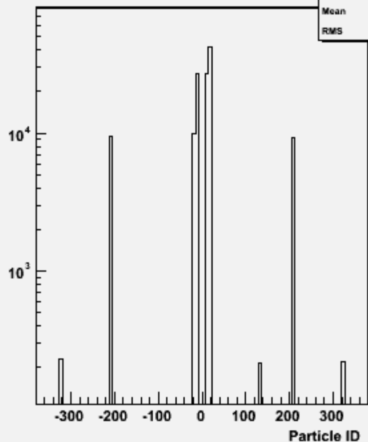
Particle ID : w103788 ae1_e1n2n2e3e3_o
