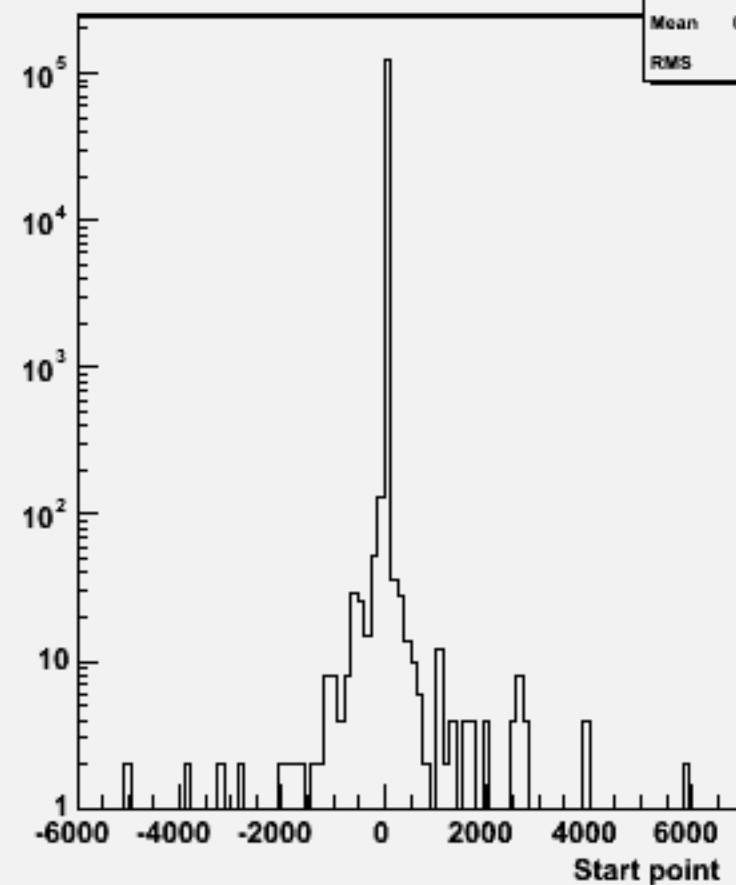
Start point Z : w103788 ae1_e1n2n2e3e3_o
