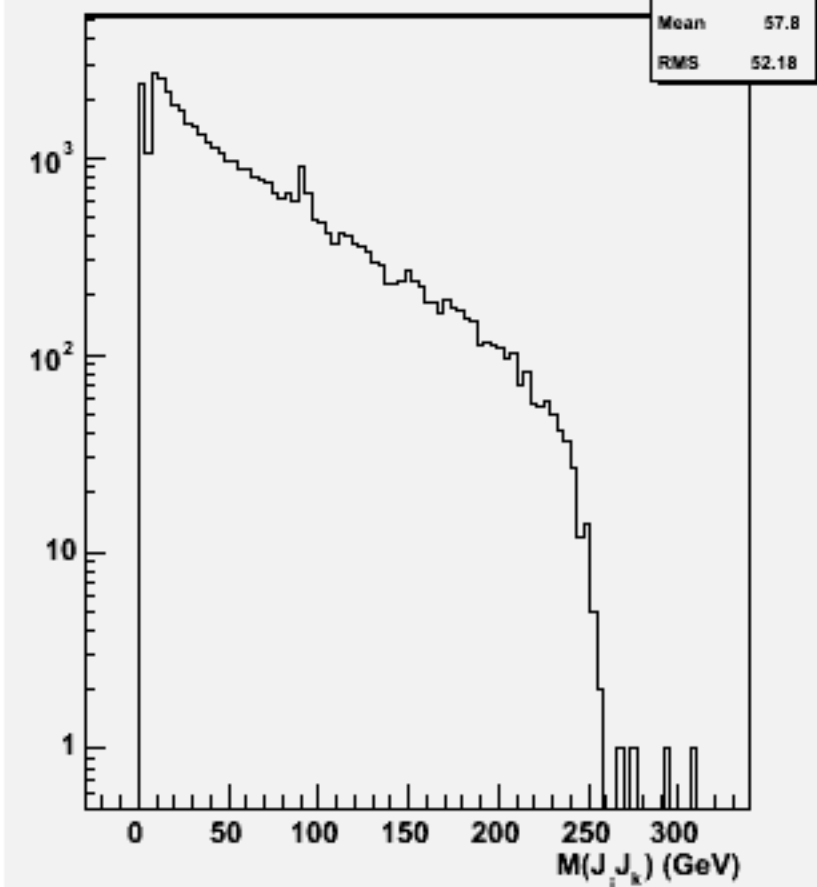
2jets mass(All comb)w103786 ae1_e1n2n2e1e1_o
