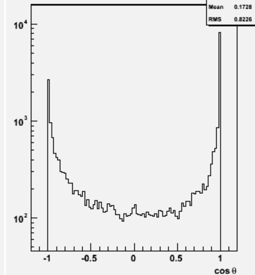
Jet cos \theta (All jets)w103786 ae1_e1n2n2e1e1_o
