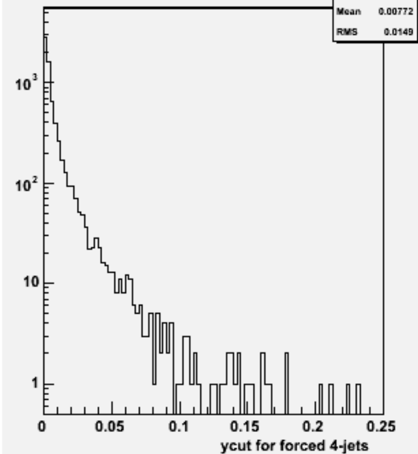
Ycut for 4-jets :w103786 ae1_e1n2n2e1e1_o
