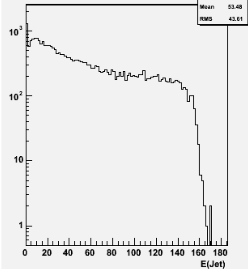
Jet energies(All jets)w103786 ae1_e1n2n2e1e1_o
