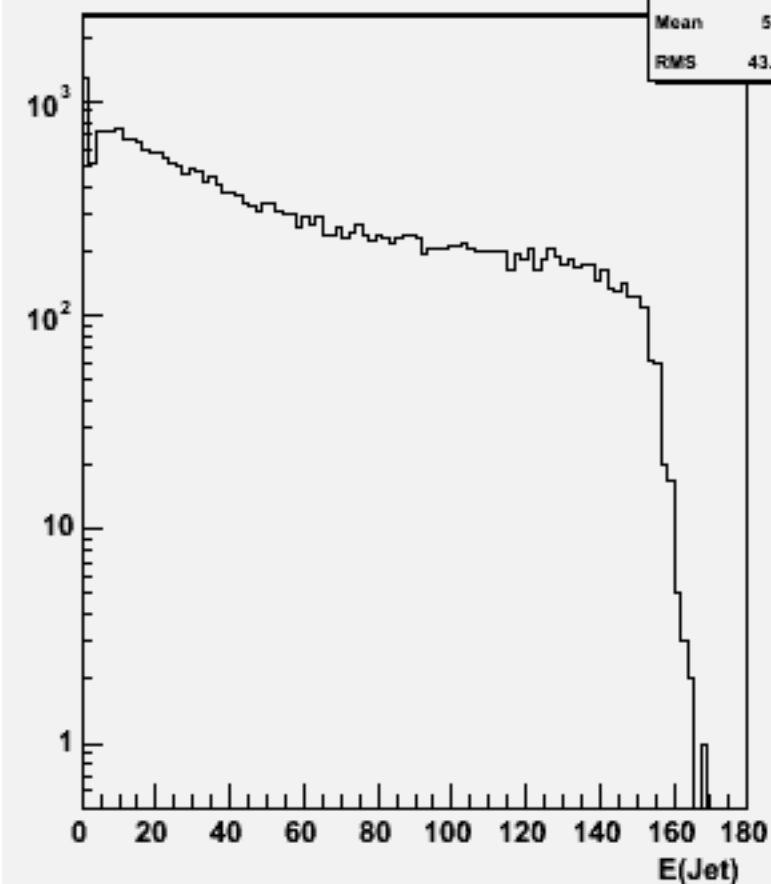
Jet energies(All jets)w103784 ae1_e1n2n2e1e1_o
