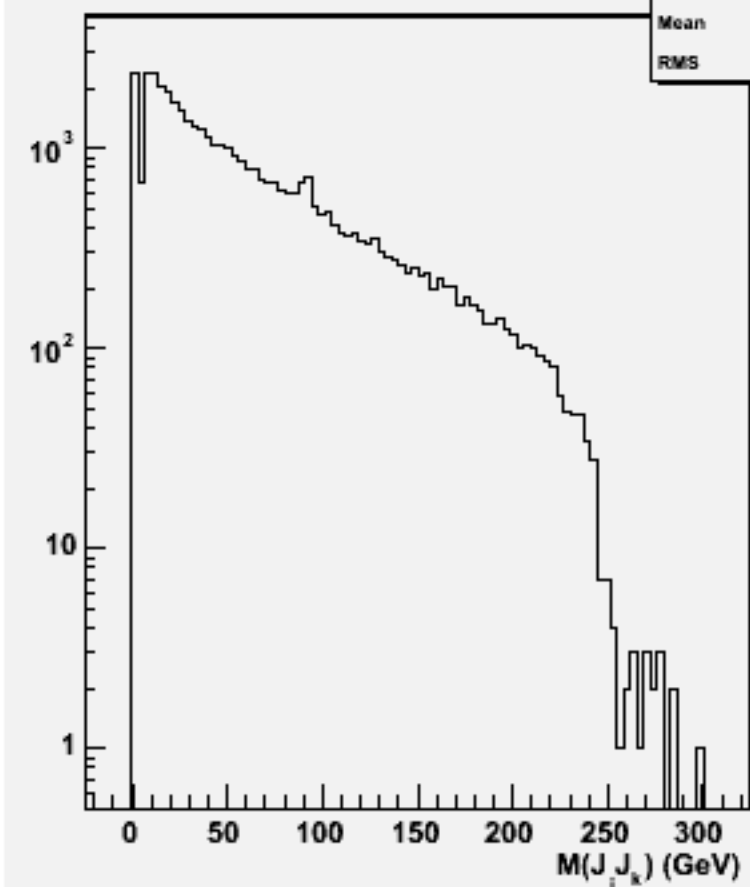
2jets mass(All comb)w103784 ae1_e1n2n2e1e1_o
