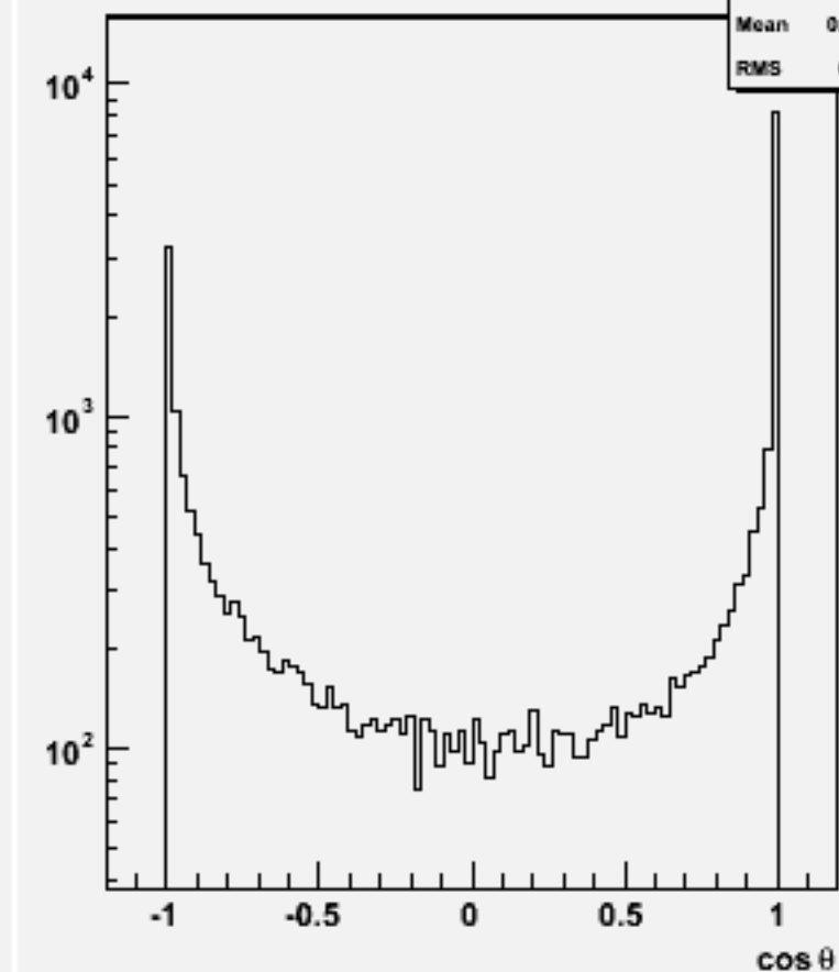
Jet cos \theta (All jets)w103784 ae1_e1n2n2e1e1_o
