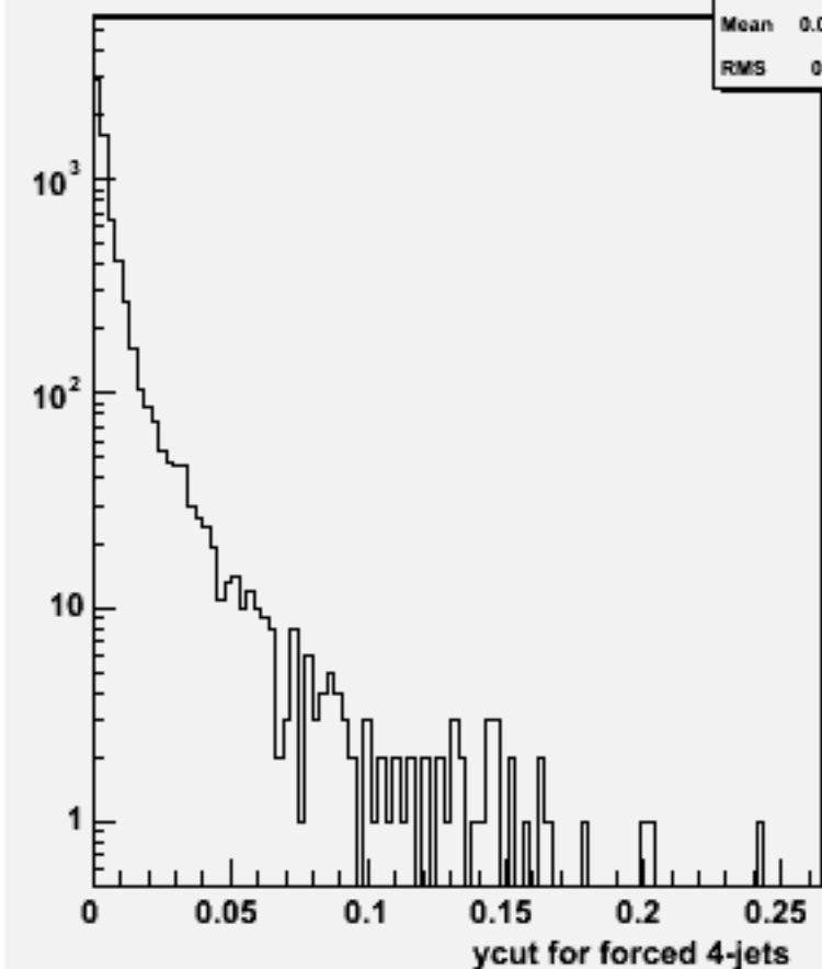
Ycut for 4-jets :w103784 ae1_e1n2n2e1e1_o
