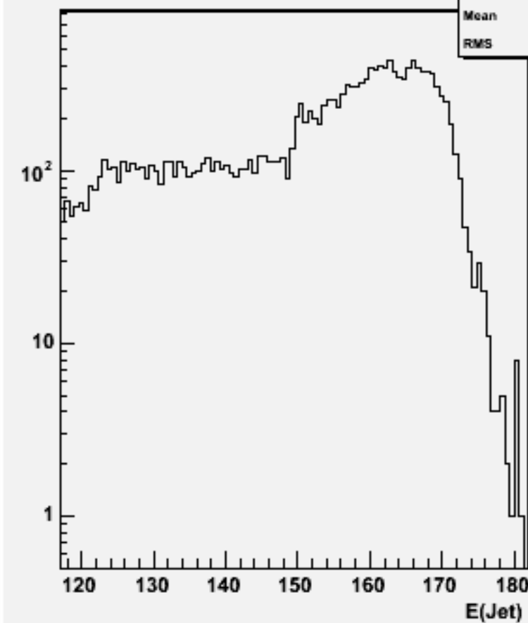
Jet energies(All jets)w103783 ae1_e1cccc_o
