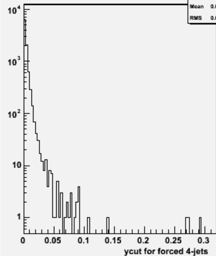
Ycut for 4-jets :w103783 ae1_e1cccc_o
