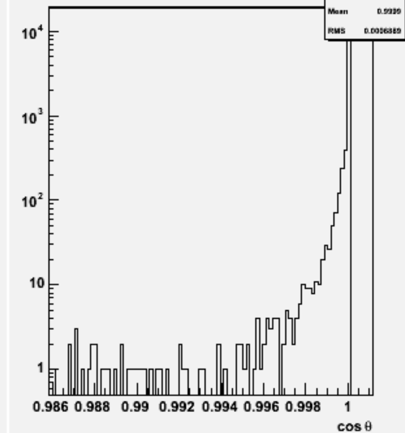
Jet cos \theta (All jets)w103783 ae1_e1cccc_o
