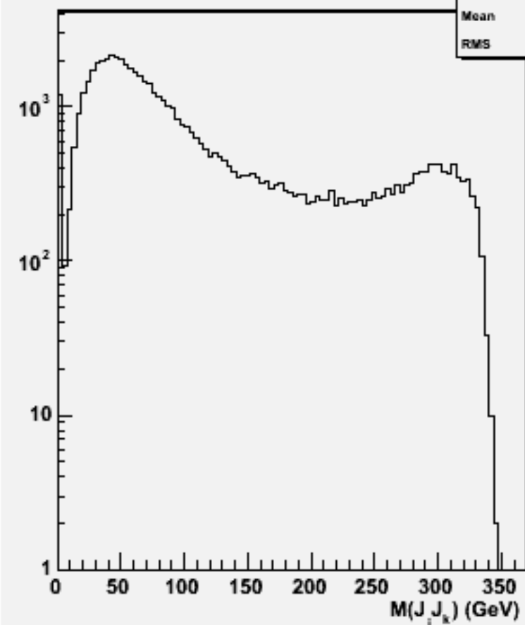
2jets mass(All comb)w103783 ae1_e1cccc_o
