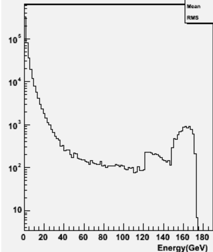
Particle Energy : w103781 ae1_e1cccc_o
