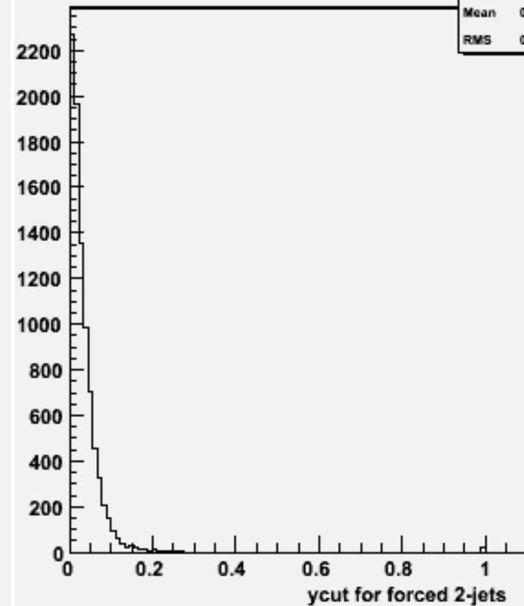
Ycut for 2-jets :w103781 ae1_e1cccc_o
