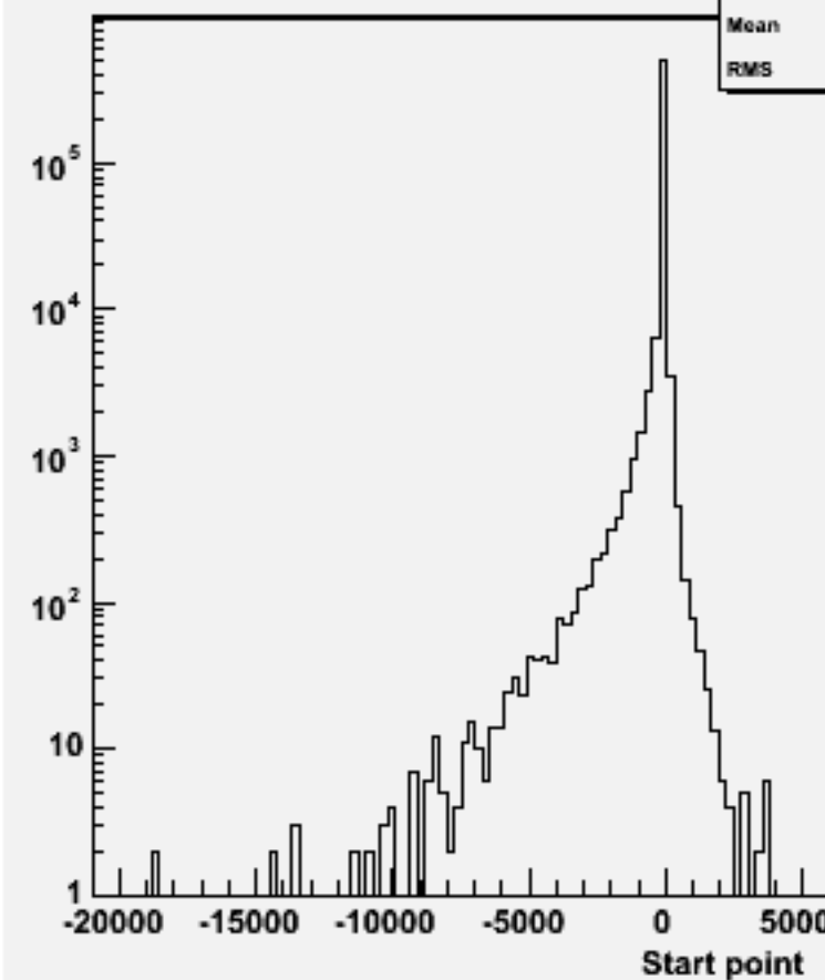
Start point Z : w103781 ae1_e1cccc_o
