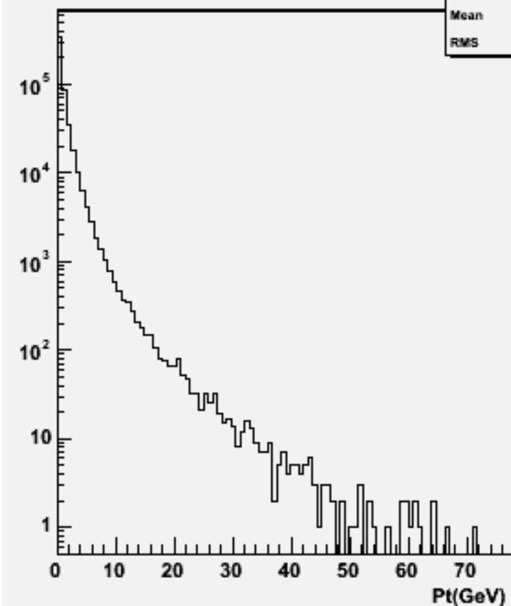
Particle Pt : w103781 ae1_e1cccc_o
