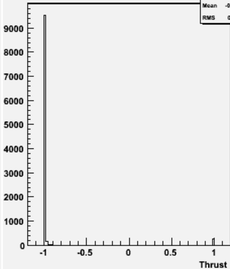
cos \Theta (thrust) w103781 ae1_e1cccc_o
