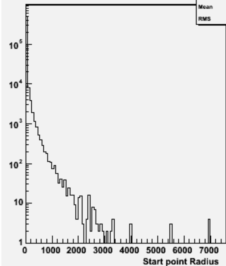
Start point R : w103781 ae1_e1cccc_o
