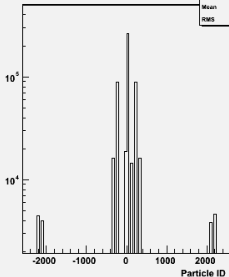
Particle ID : w103781 ae1_e1cccc_o
