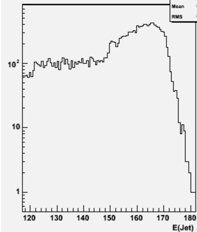
Jet energies(All jets)w103781 ae1_e1cccc_o
