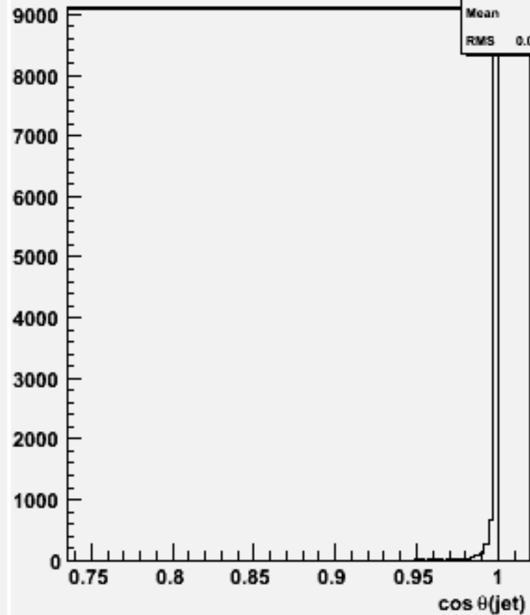
cos \theta for 2-jets :w103781 ae1_e1cccc_o
