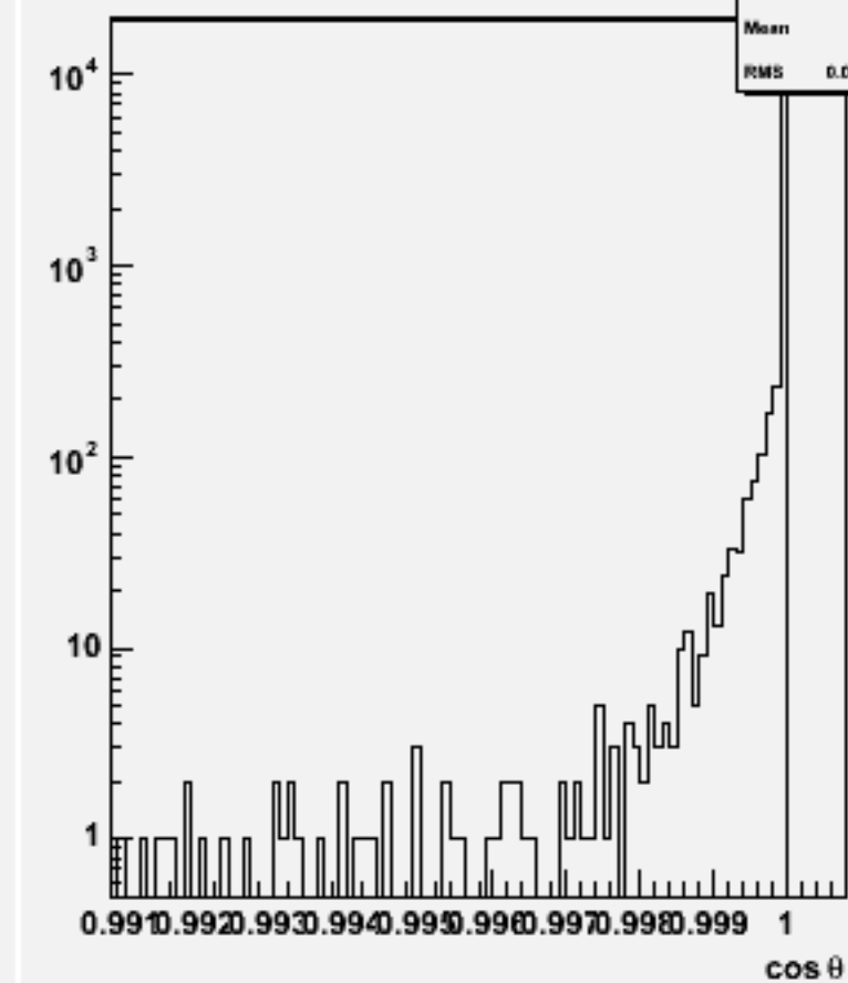
Jet cos \theta (All jets)w103781 ae1_e1cccc_o
