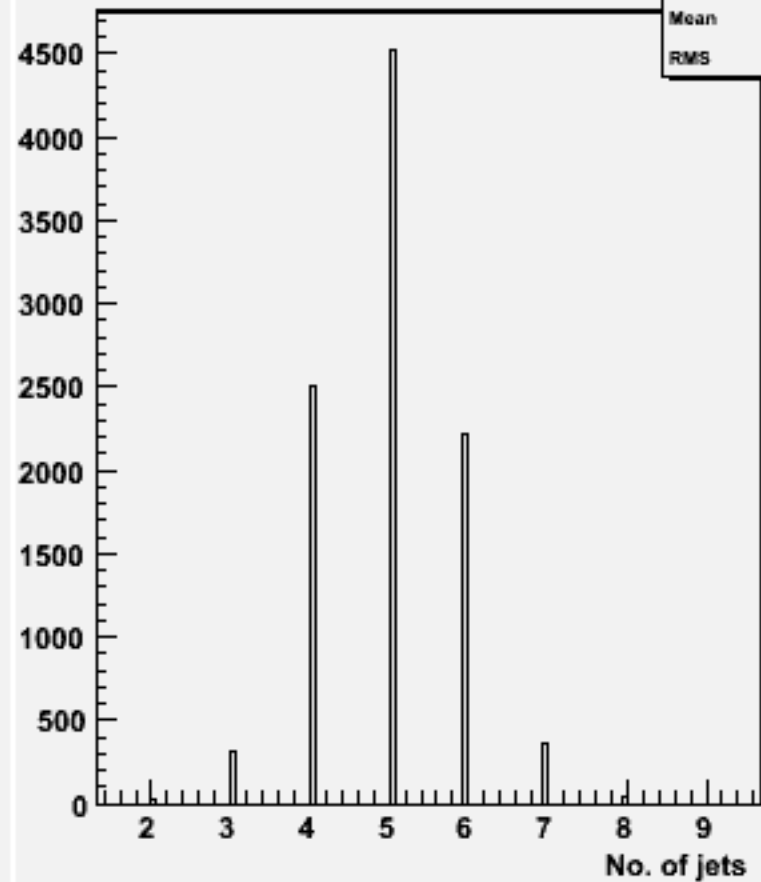
No. jets (ycut=0.001) : w103781 ae1_e1cccc_o
