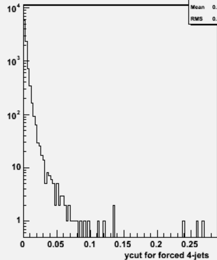
Ycut for 4-jets :w103781 ae1_e1cccc_o
