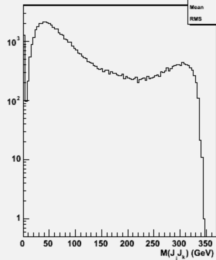
2jets mass(All comb)w103781 ae1_e1cccc_o
