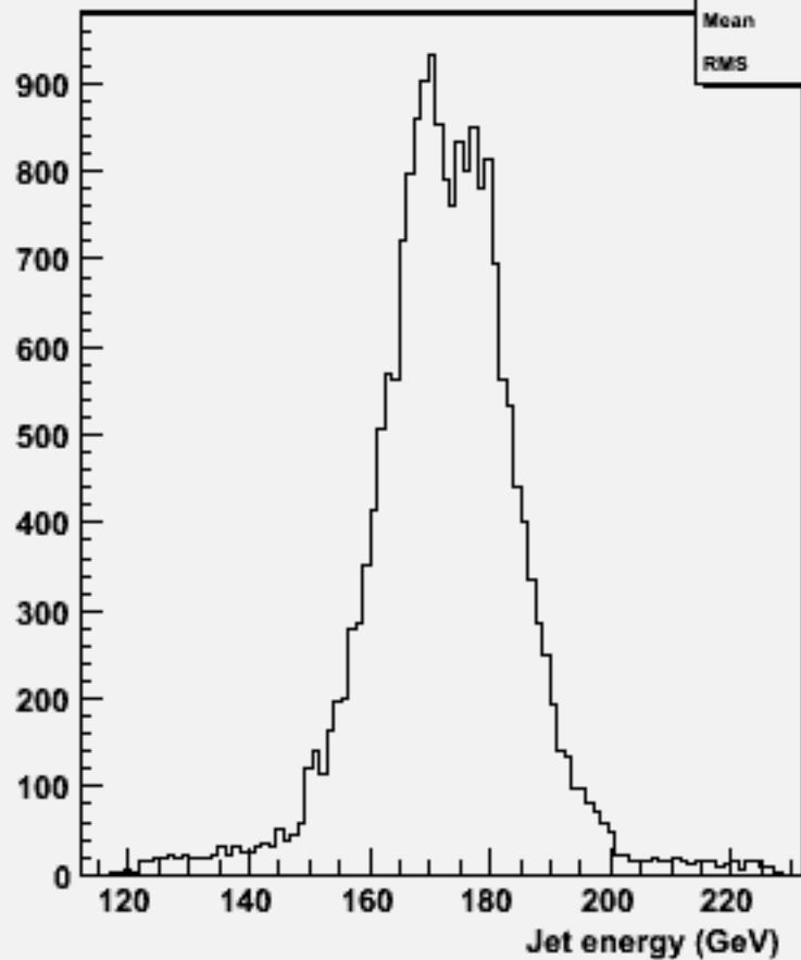
energy for 2-jets :w103781 ae1_e1cccc_o
