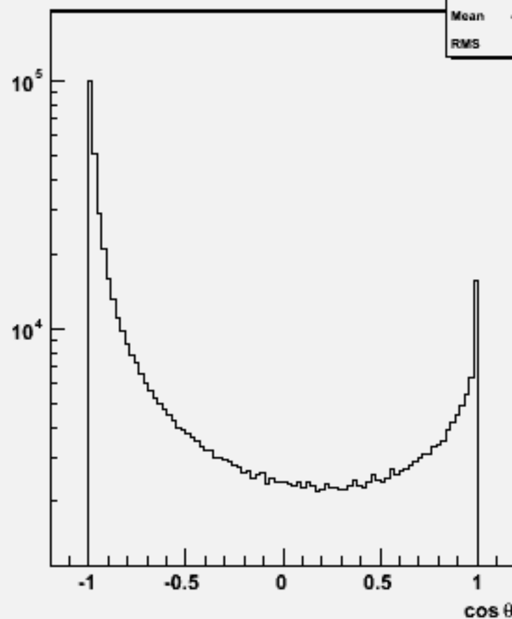
Particle cos \theta : w103781 ae1_e1cccc_o
