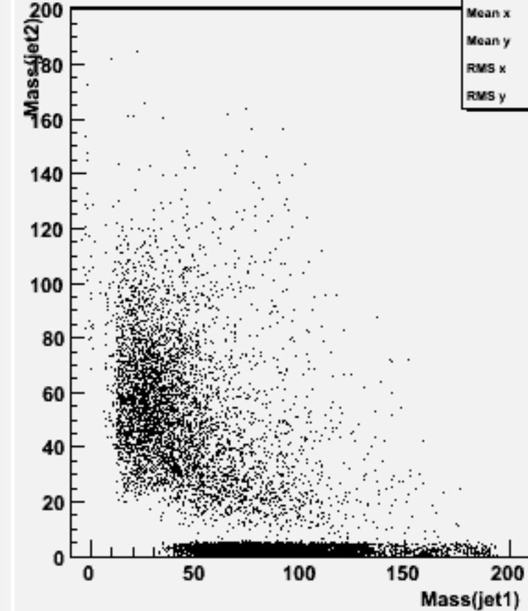
Jet mass for forced 2-jets : w103781 ae1_e1cccc_o
