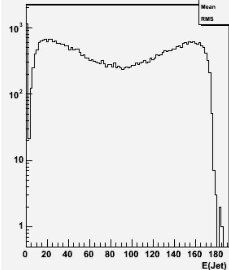
Jet energies(All jets)w103780 ae1_e1cccc_o
