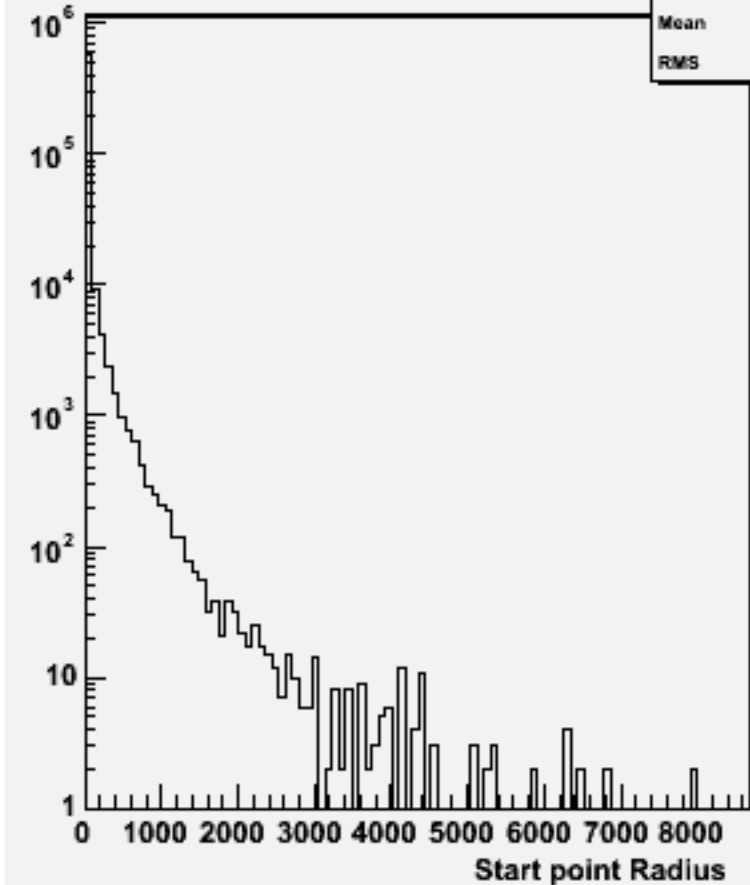
Start point R : w103780 ae1_e1cccc_o
