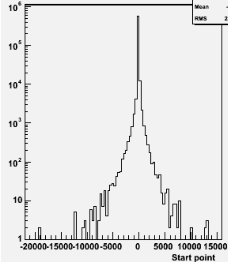
Start point Z : w103780 ae1_e1cccc_o
