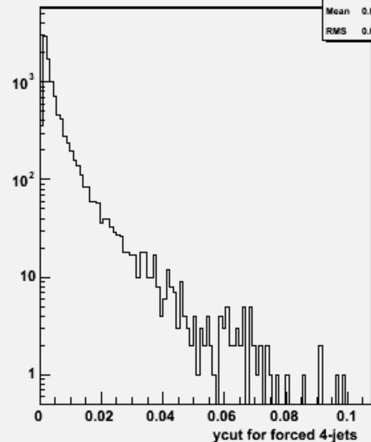
Ycut for 4-jets :w103780 ae1_e1cccc_o
