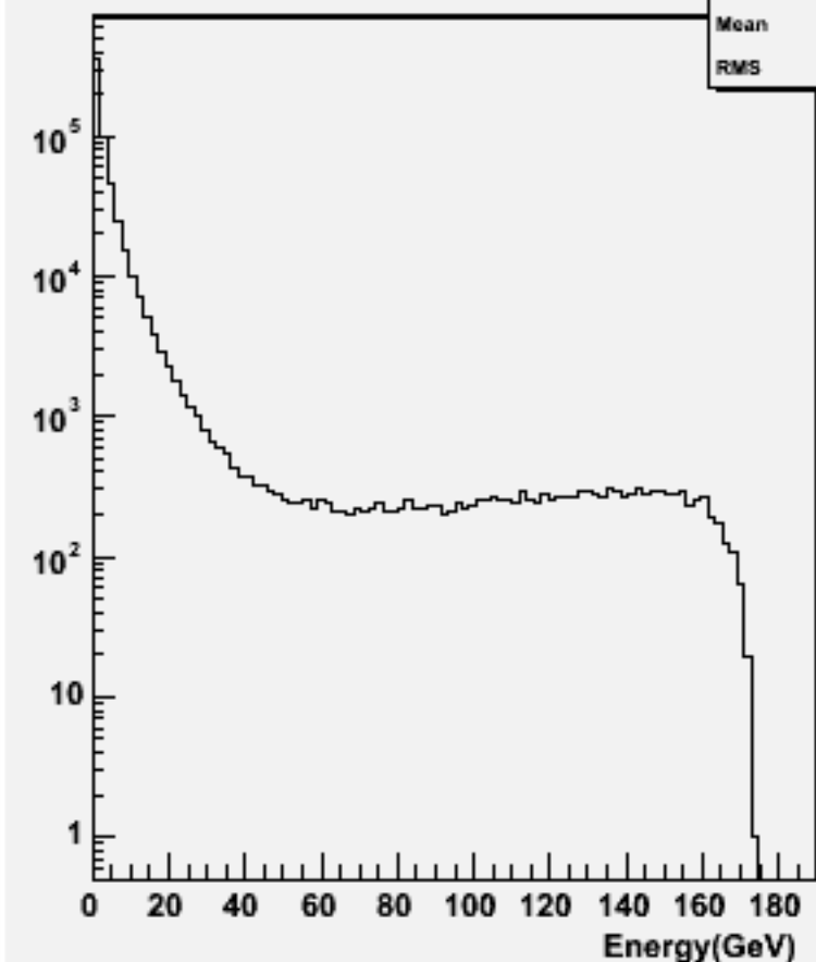
Particle Energy : w103780 ae1_e1cccc_o
