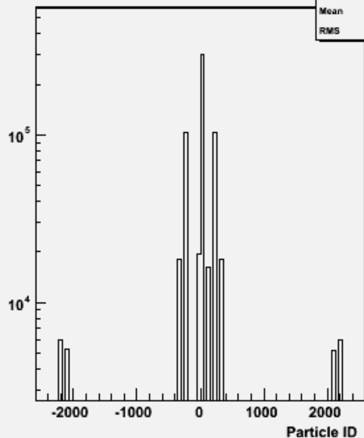
Particle ID : w103780 ae1_e1cccc_o
