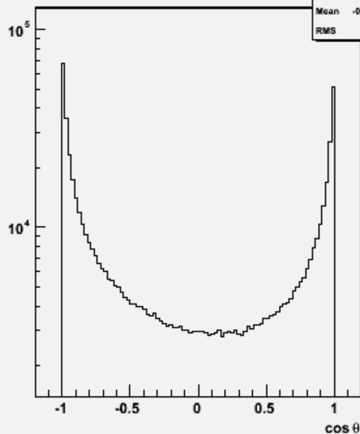
Particle cos \theta : w103780 ae1_e1cccc_o
