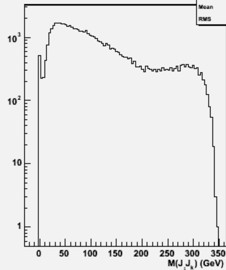
2jets mass(All comb)w103780 ae1_e1cccc_o
