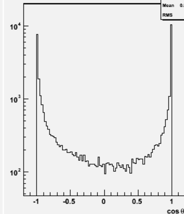
Jet cos \theta (All jets)w103780 ae1_e1cccc_o
