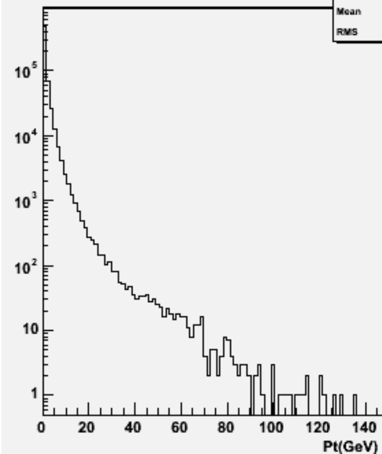
Particle Pt : w103780 ae1_e1cccc_o
