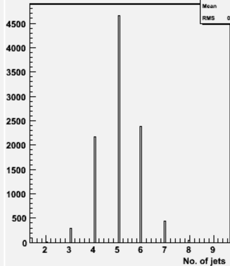
No. jets (ycut=0.001) : w103779 ae1_e1uucc_o
