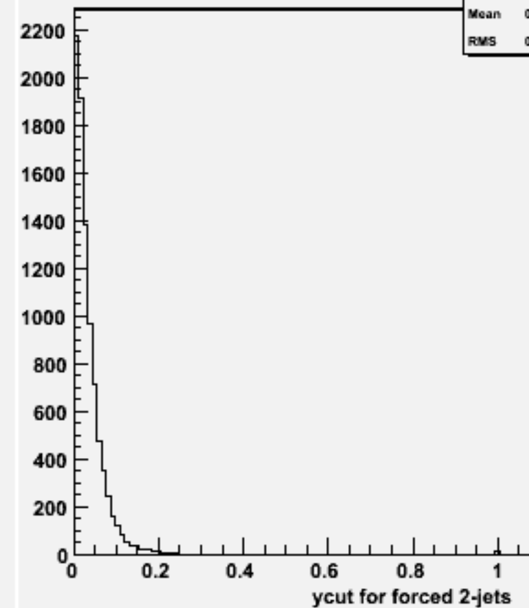
Ycut for 2-jets :w103779 ae1_e1uucc_o
