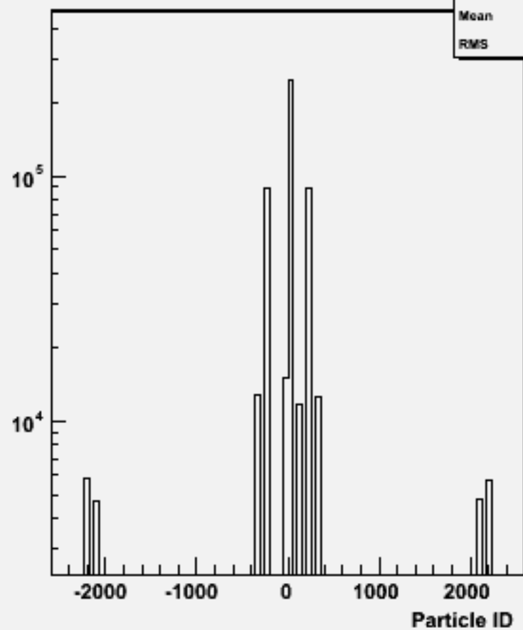
Particle ID : w103779 ae1_e1uucc_o
