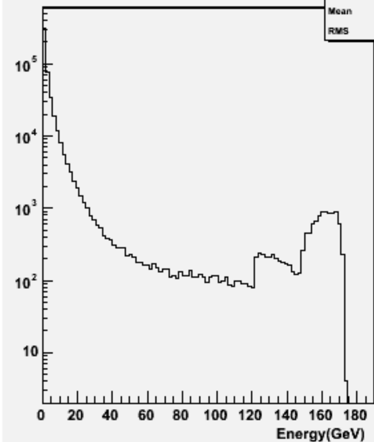
Particle Energy : w103779 ae1_e1uucc_o
