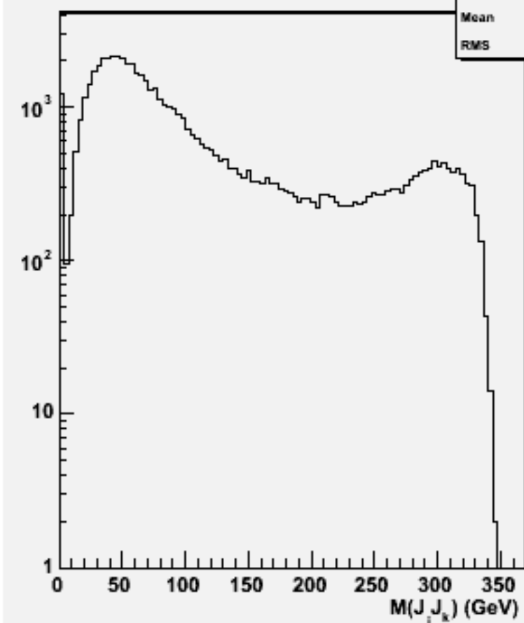
2jets mass(All comb)w103779 ae1_e1uucc_o
