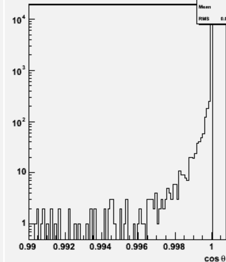
Jet cos \theta (All jets)w103779 ae1_e1uucc_o
