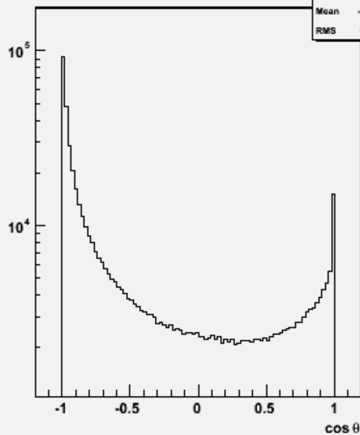
Particle cosθ : w103779 ae1_e1uucc_o
