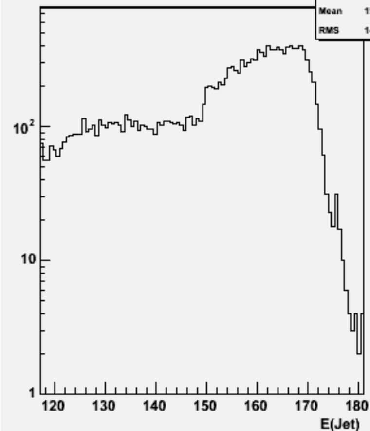
Jet energies(All jets)w103779 ae1_e1uucc_o
