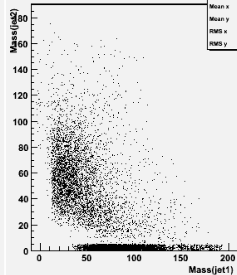
Jet mass for forced 2-jets : w103779 ae1_e1uucc_o
