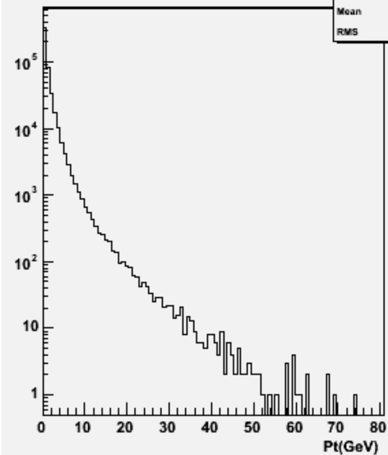
Particle Pt : w103779 ae1_e1uucc_o
