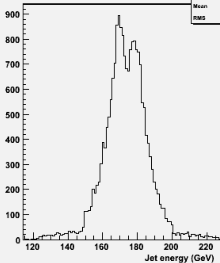
energy for 2-jets :w103779 ae1_e1uucc_o
