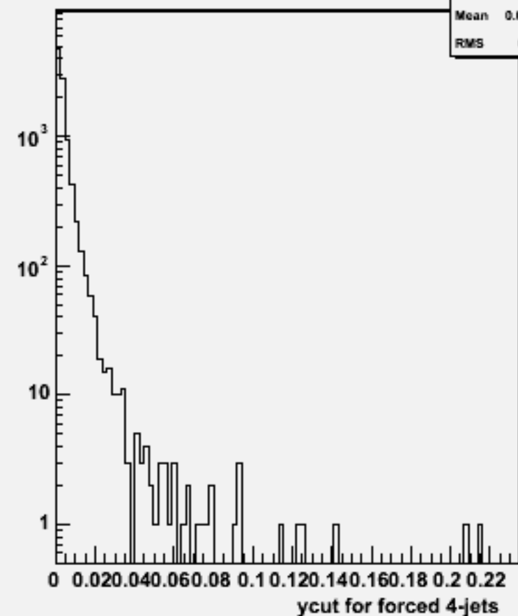
Ycut for 4-jets :w103779 ae1_e1uucc_o
