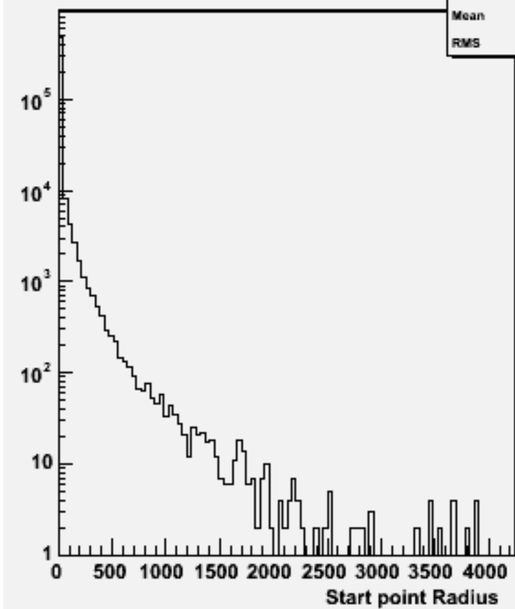
Start point R : w103779 ae1_e1uucc_o
