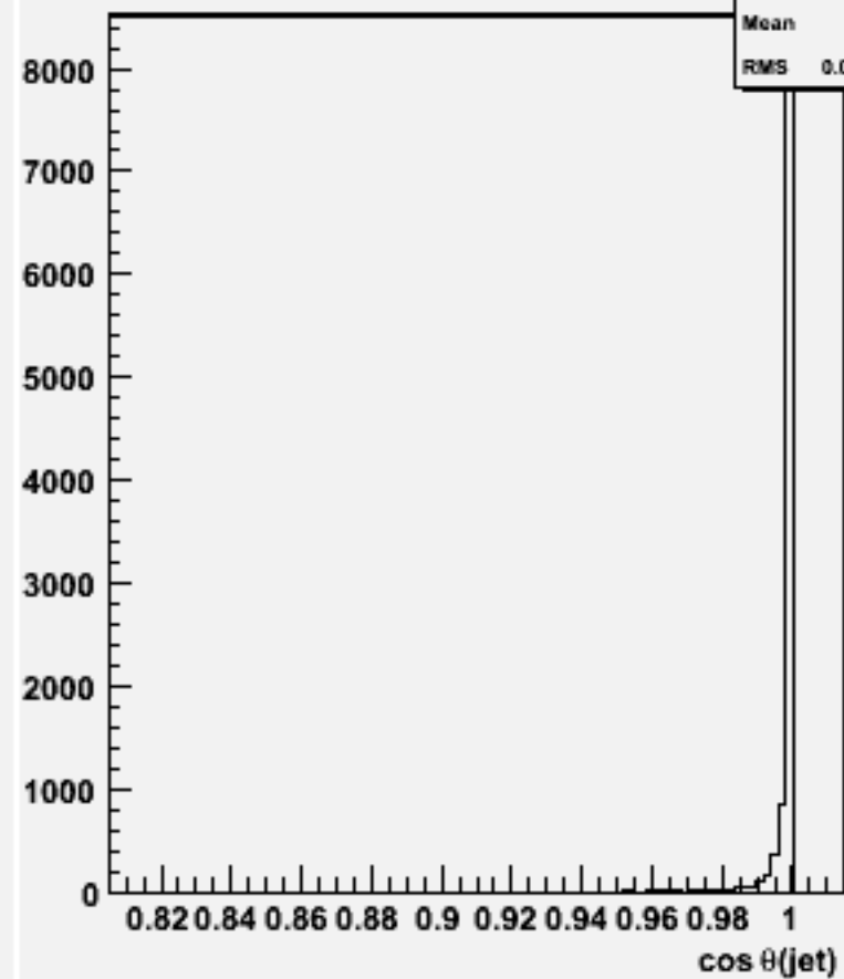
cos \Theta for 2-jets :w103779 ae1_e1uucc_o
