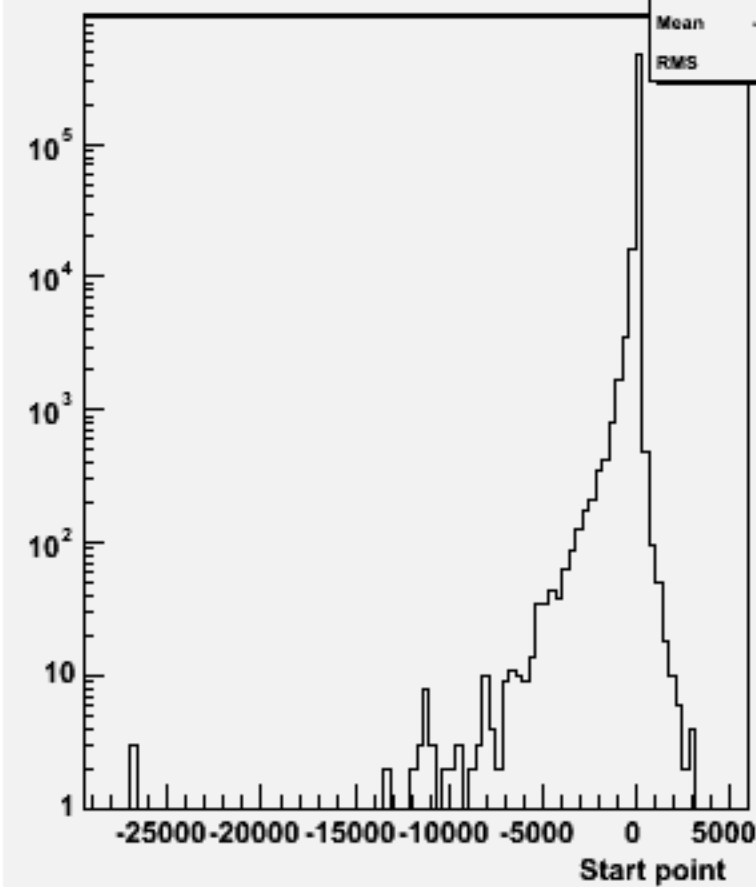
Start point Z : w103779 ae1_e1uucc_o
