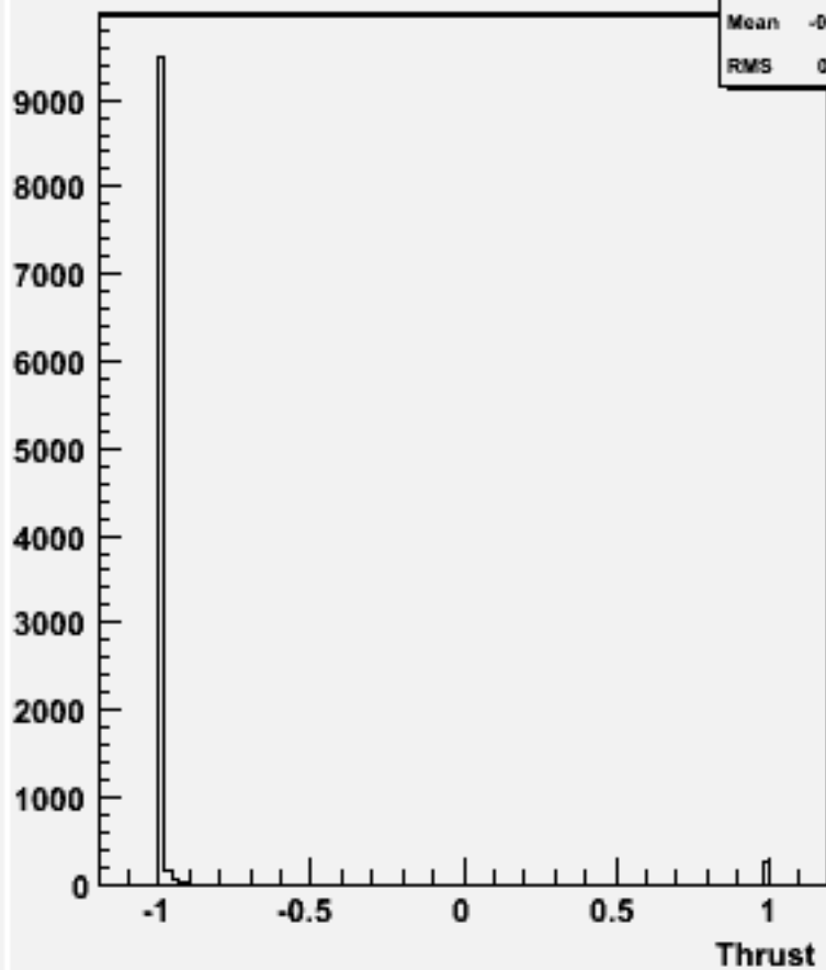
cos \Theta (thrust) w103779 ae1_e1uucc_o
