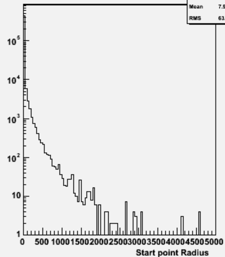
Start point R : w103773 ae1_e1uuuu_o
