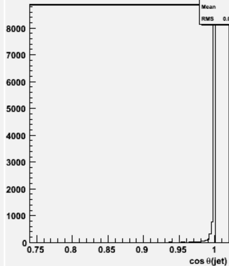
cos \theta for 2-jets :w103773 ae1_e1uuuu_o
