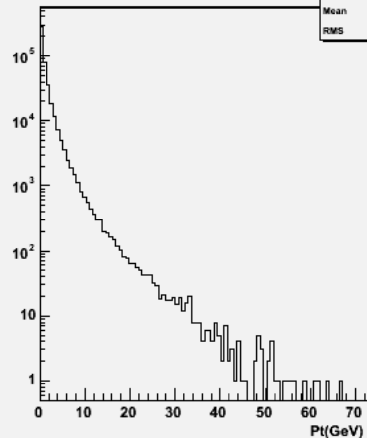
Particle Pt : w103773 ae1_e1uuuu_o
