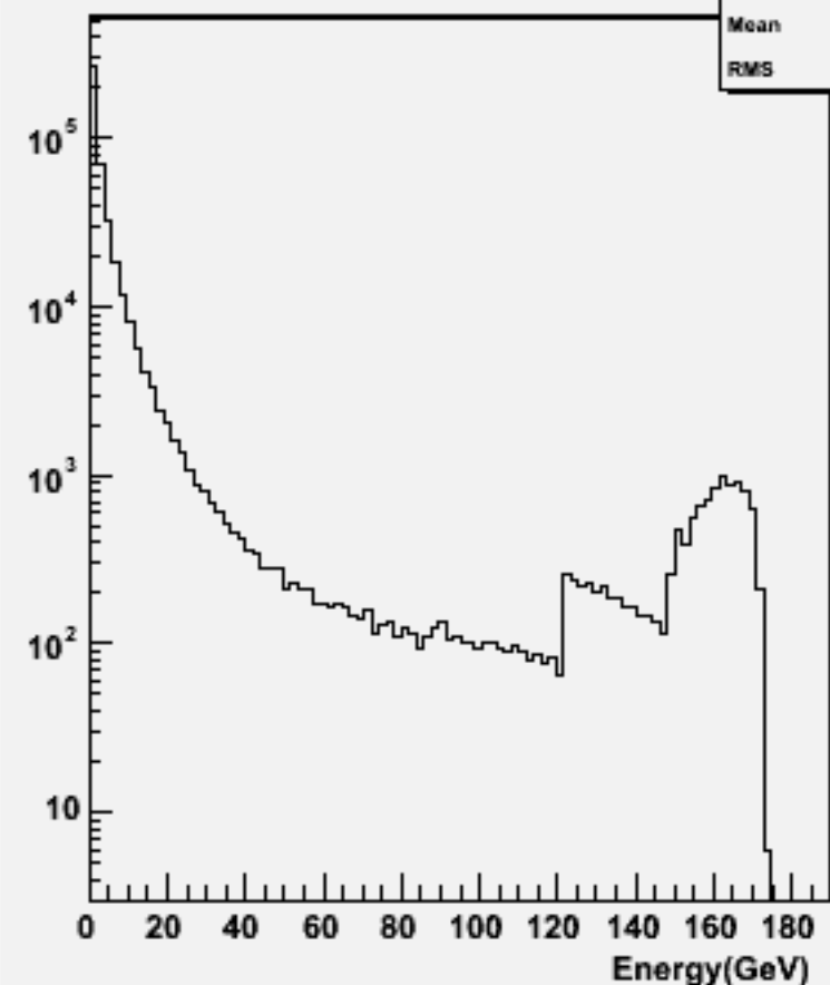
Particle Energy : w103773 ae1_e1uuuu_o
