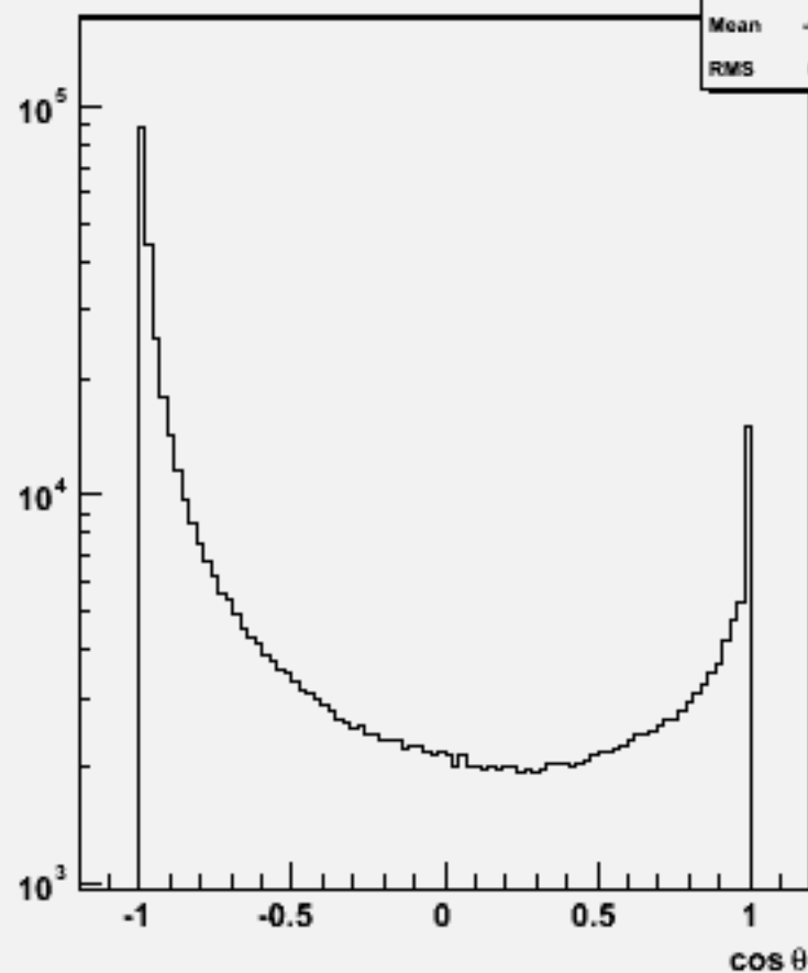
Particle cosθ : w103773 ae1_e1uuuu_o
