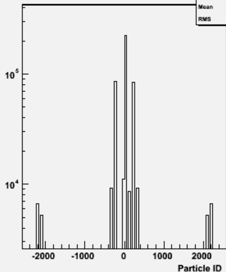
Particle ID : w103773 ae1_e1uuuu_o
