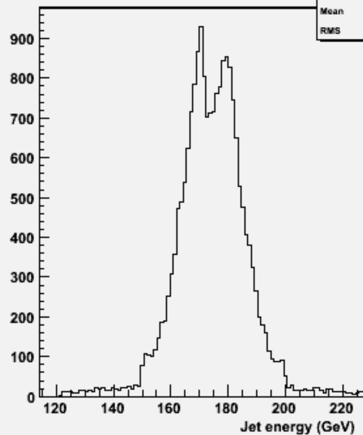
energy for 2-jets :w103773 ae1_e1uuuu_o
