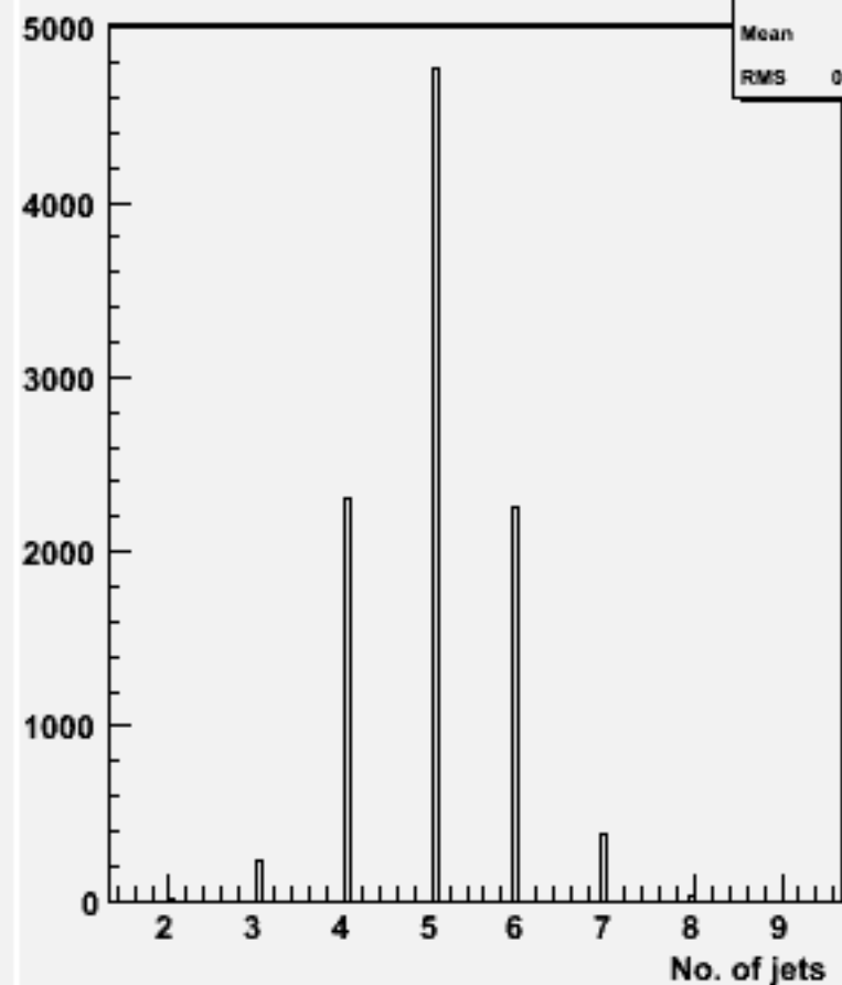
No. jets (ycut=0.001) : w103773 ae1_e1uuuu_o
