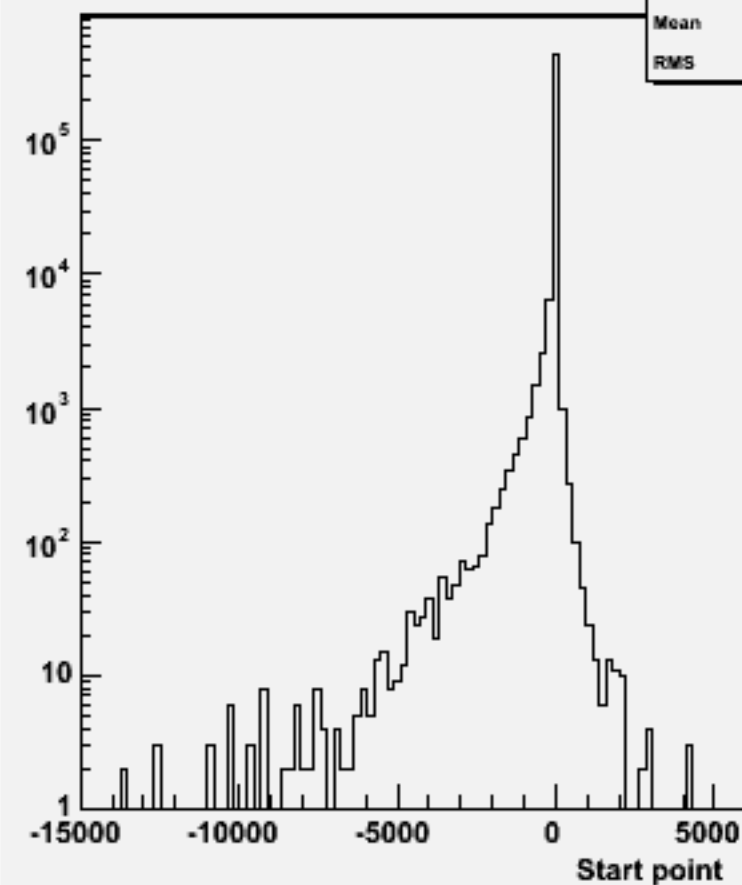
Start point Z : w103773 ae1_e1uuuu_o
