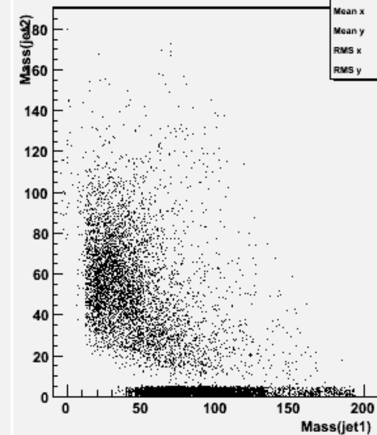
Jet mass for forced 2-jets : w103773 ae1_e1uuuu_o
