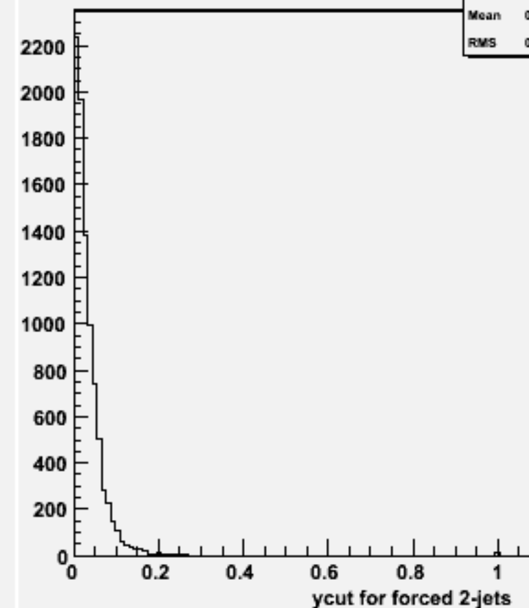
Ycut for 2-jets :w103773 ae1_e1uuuu_o
