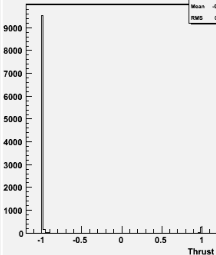
cos \Theta (thrust) w103773 ae1_e1uuuu_o
