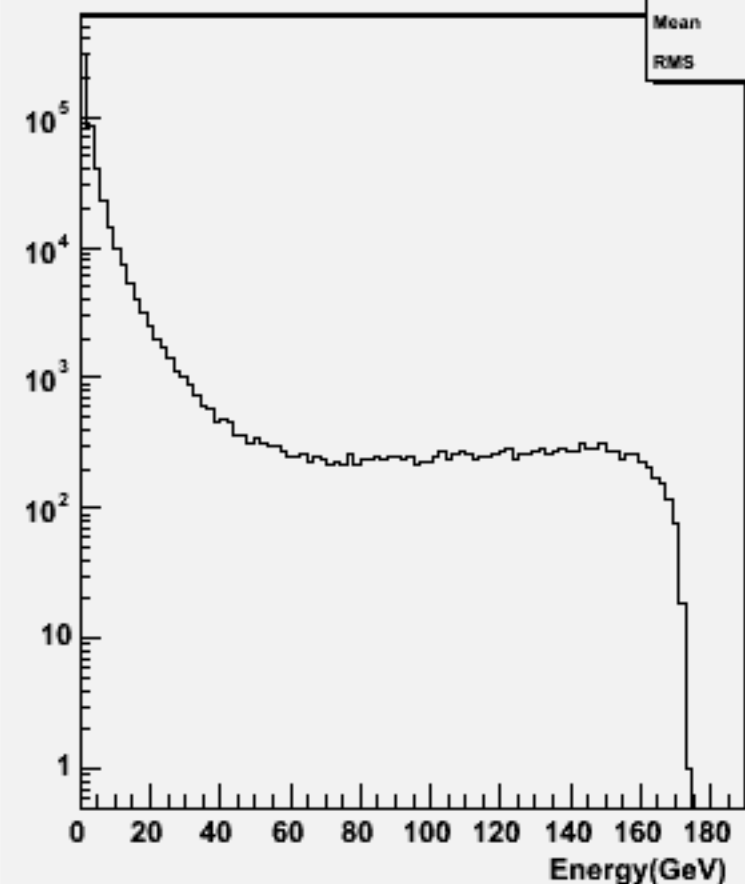
Particle Energy : w103772 ae1_e1uuuu_o
