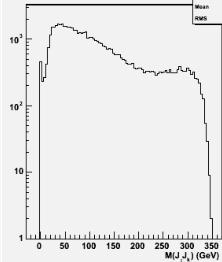
2jets mass(All comb)w103772 ae1_e1uuuu_o
