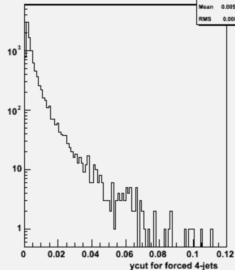
Ycut for 4-jets :w103772 ae1_e1uuuu_o
