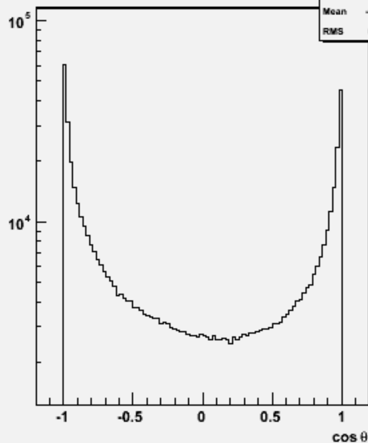
Particle cosθ : w103772 ae1_e1uuuu_o
