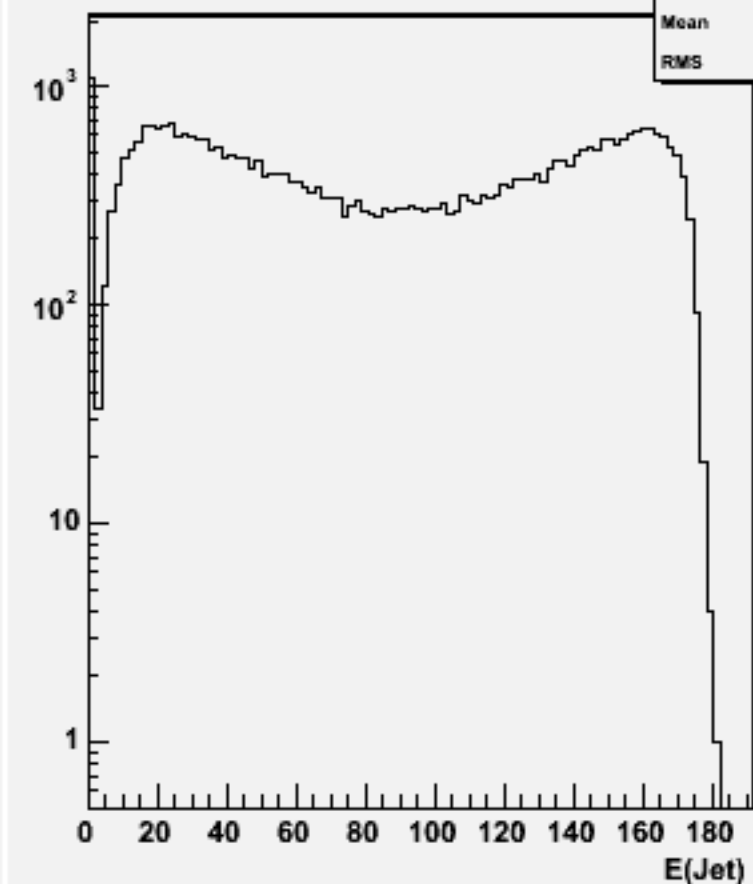
Jet energies(All jets)w103772 ae1_e1uuuu_o
