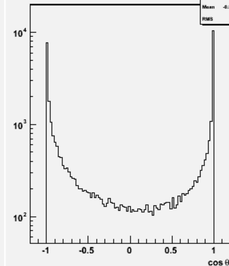
Jet cos \theta (All jets)w103772 ae1_e1uuuu_o
