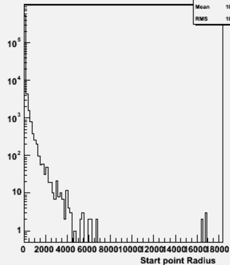
Start point R : w103772 ae1_e1uuuu_o
