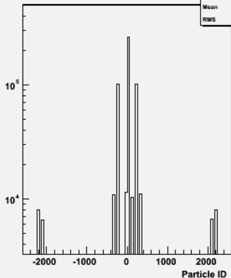
Particle ID : w103772 ae1_e1uuuu_o
