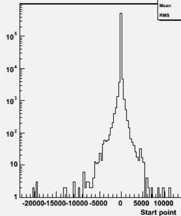
Start point Z : w103772 ae1_e1uuuu_o
