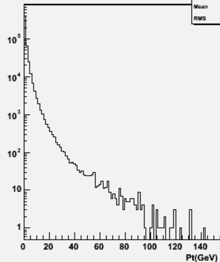
Particle Pt : w103772 ae1_e1uuuu_o
