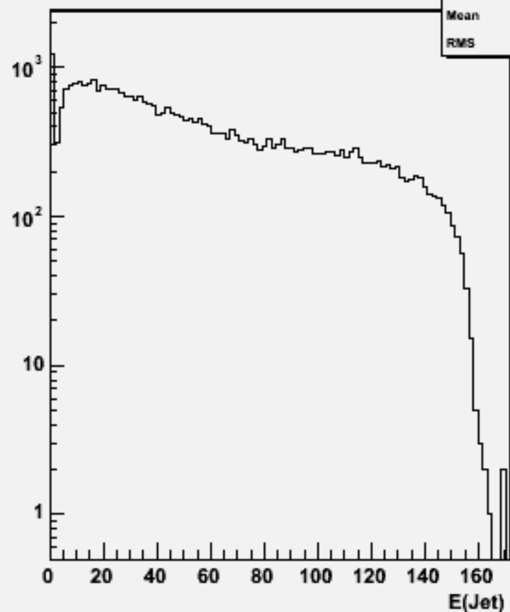
Jet energies(All jets)w103768 ae1_e1n3n3cc_o
