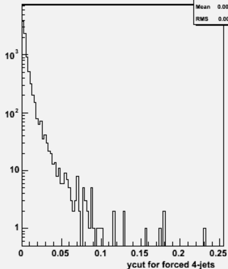
Ycut for 4-jets :w103768 ae1_e1n3n3cc_o
