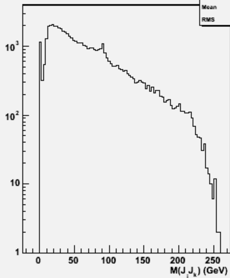
2jets mass(All comb)w103768 ae1_e1n3n3cc_o
