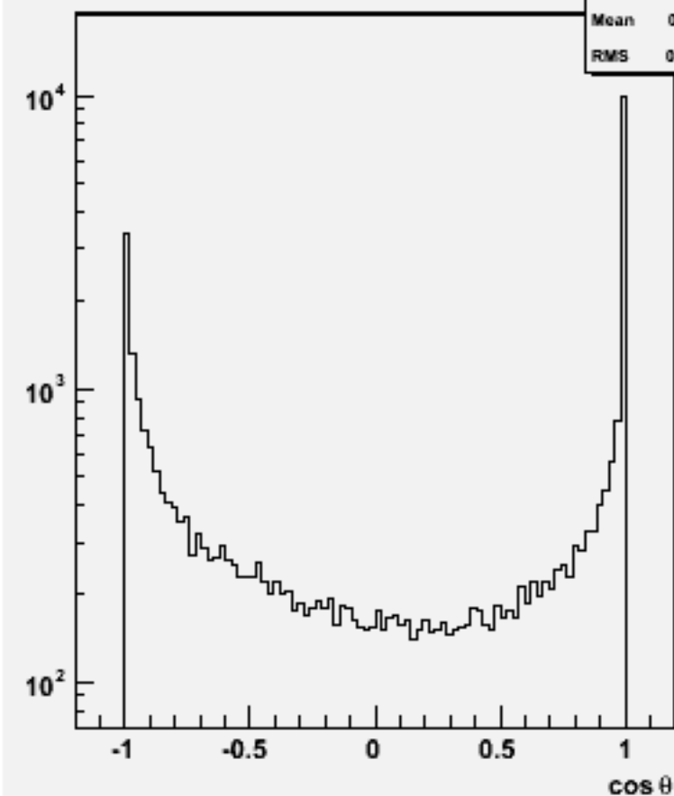
Jet cos \theta (All jets)w103768 ae1_e1n3n3cc_o
