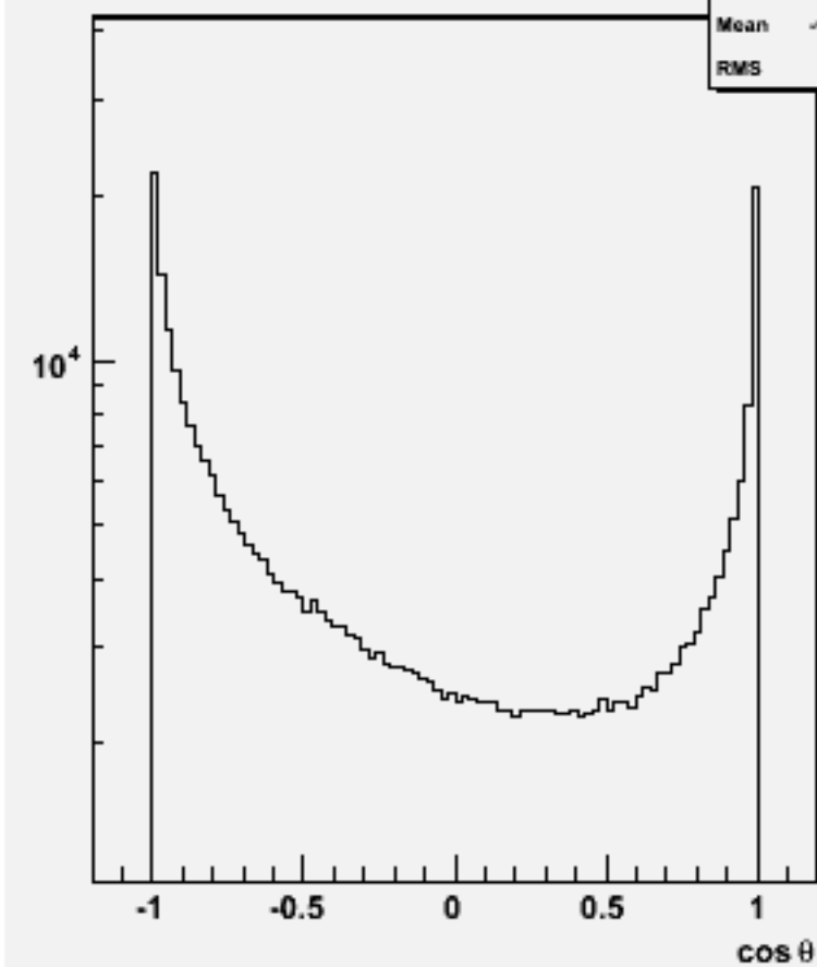
Particle cos θ : w103764 ae1_e1n3n3uu_o
