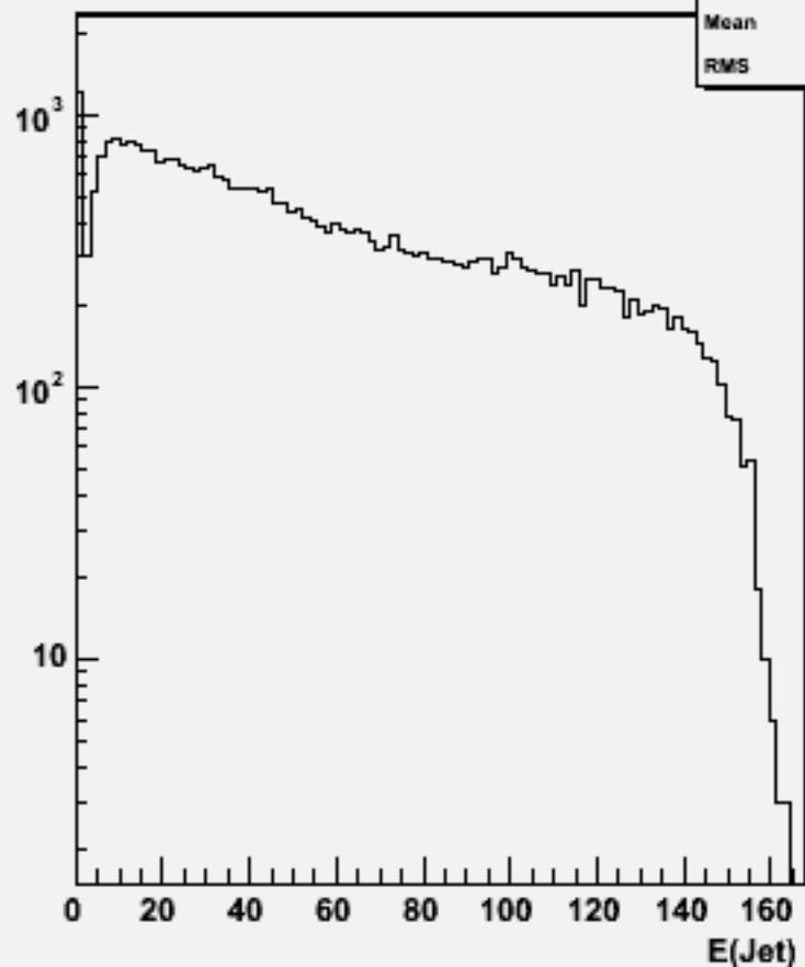
Jet energies(All jets)w103764 ae1_e1n3n3uu_o
