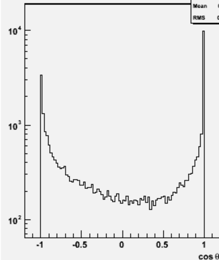
Jet cos \theta (All jets)w103764 ae1_e1n3n3uu_o
