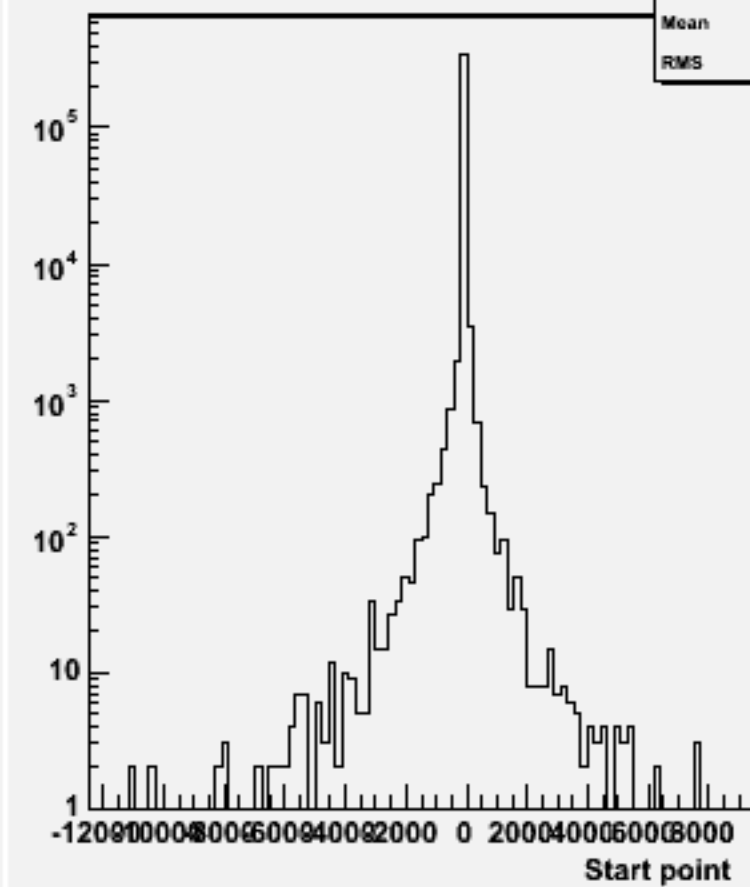
Start point Z : w103764 ae1_e1n3n3uu_o
