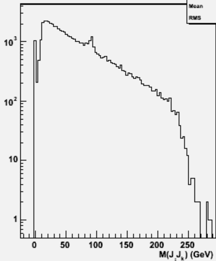
2jets mass(All comb)w103764 ae1_e1n3n3uu_o
