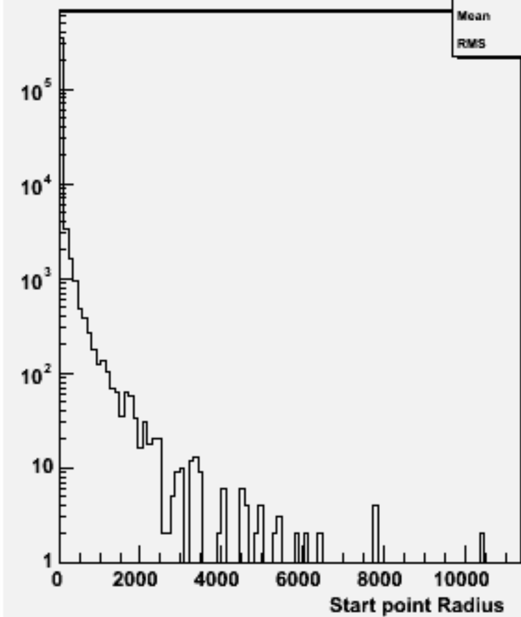
Start point R : w103764 ae1_e1n3n3uu_o
