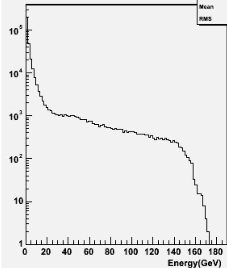
Particle Energy : w103764 ae1_e1n3n3uu_o
