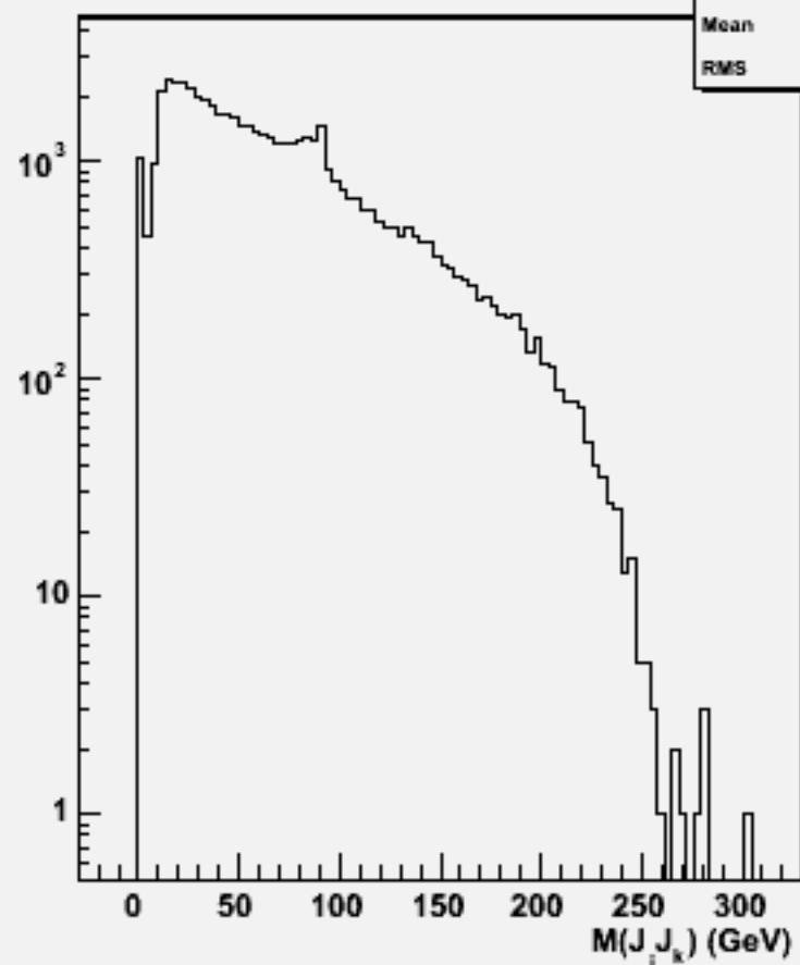
2jets mass(All comb)w103758 ae1_e1n2n2cc_o
