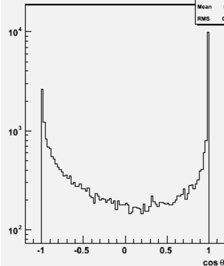
Jet cos \theta (All jets)w103758 ae1_e1n2n2cc_o
