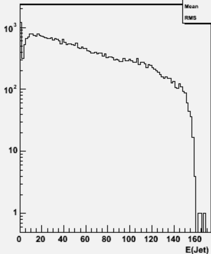
Jet energies(All jets)w103758 ae1_e1n2n2cc_o
