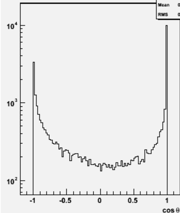
Jet cos \theta (All jets)w103752 ae1_e1n2n2uu_o
