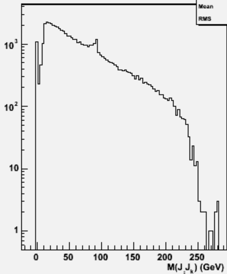
2jets mass(All comb)w103752 ae1_e1n2n2uu_o
