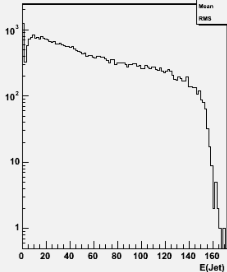
Jet energies(All jets)w103752 ae1_e1n2n2uu_o
