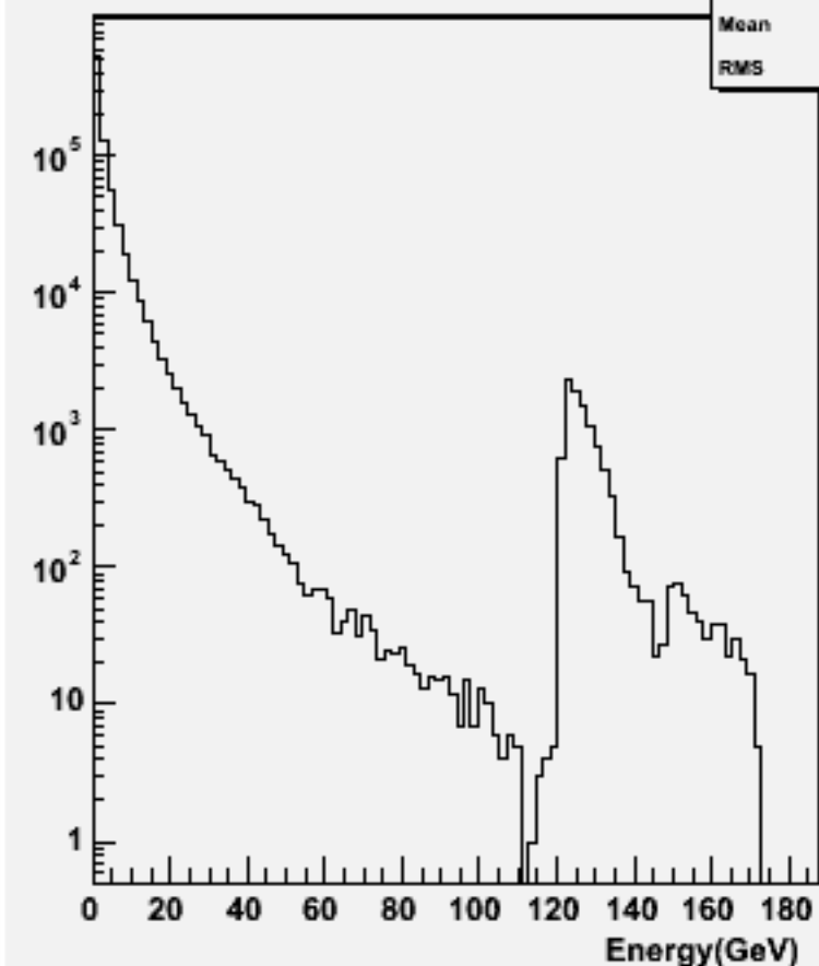
Particle Energy : w103743 ae1_e1cssc_o
