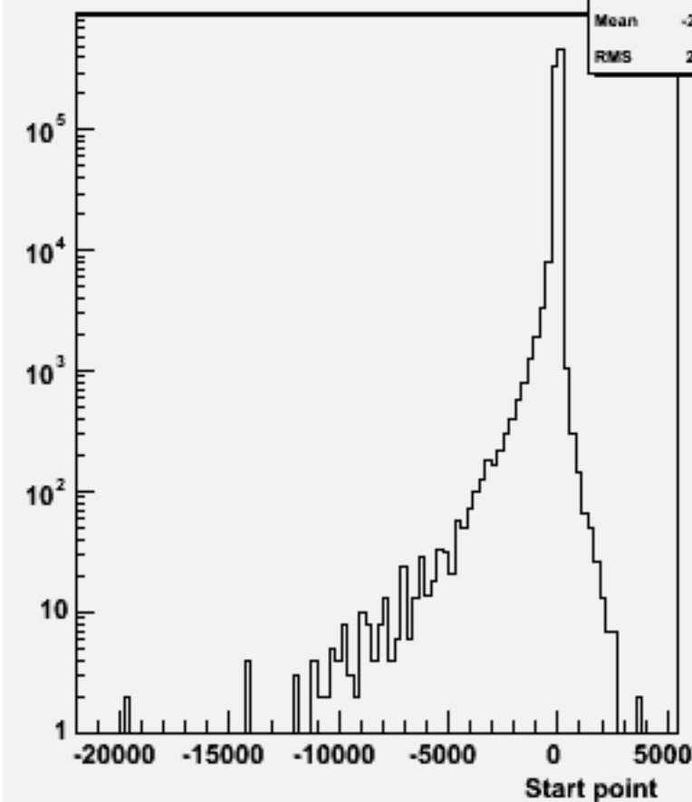
Start point Z : w103743 ae1_e1cssc_o
