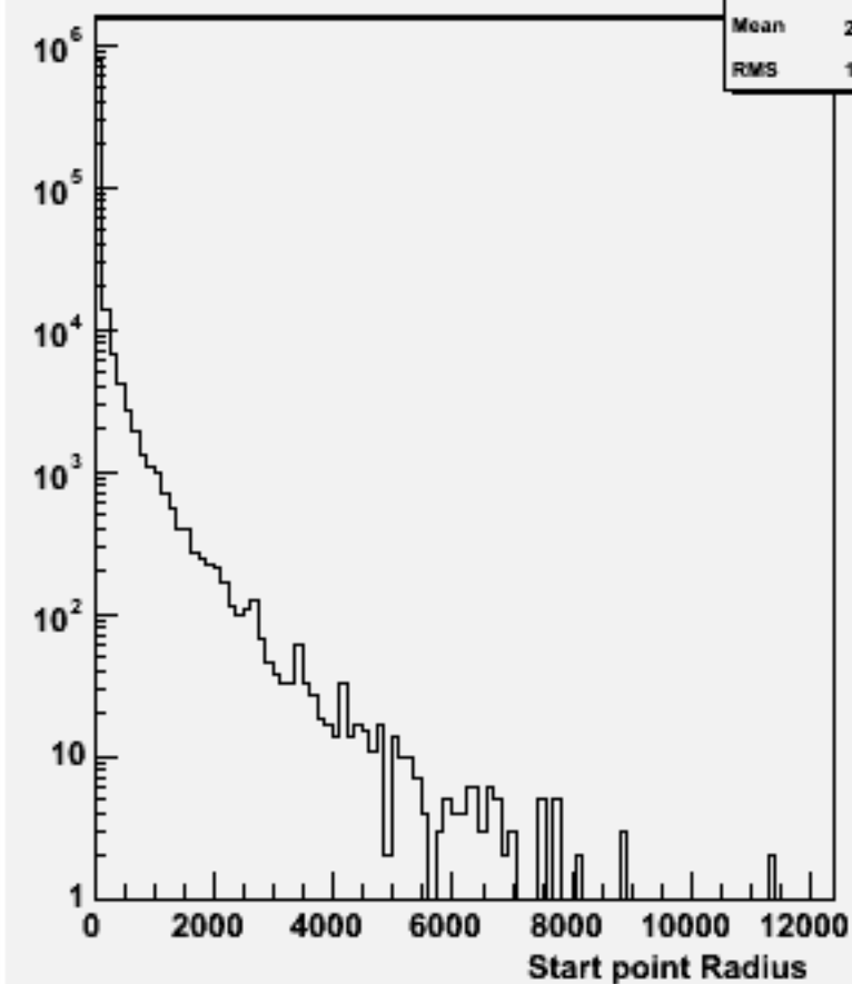
Start point R : w103743 ae1_e1cssc_o
