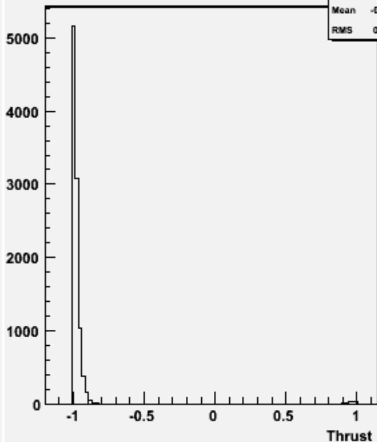
cos \Theta (thrust) w103743 ae1_e1cssc_o
