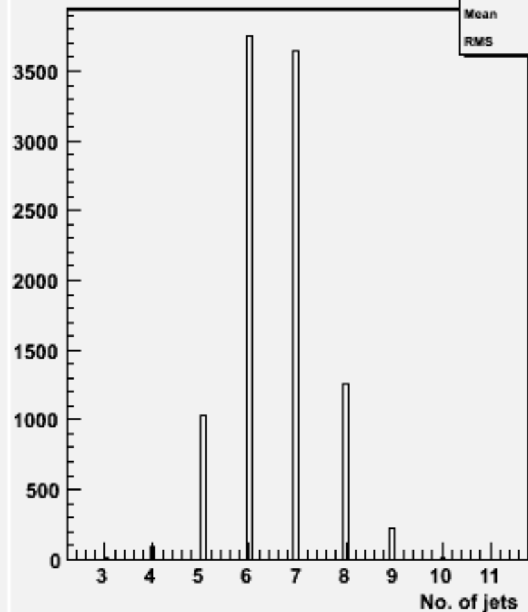
No. jets (ycut=0.001) : w103743 ae1_e1cssc_o
