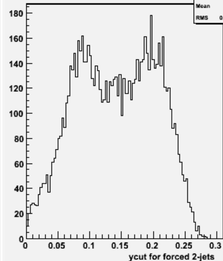
Ycut for 2-jets :w103743 ae1_e1cssc_o
