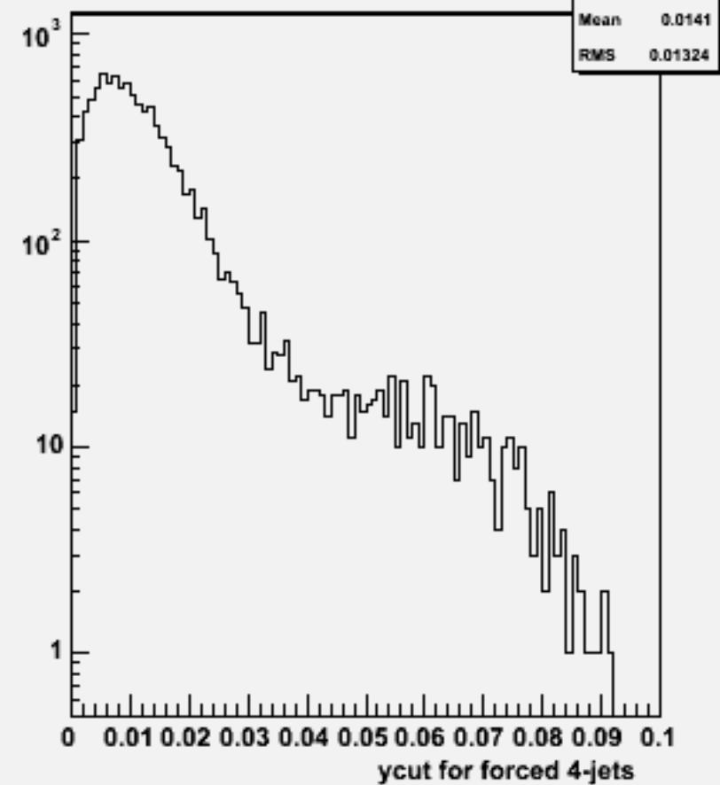
Ycut for 4-jets :w103743 ae1_e1cssc_o
