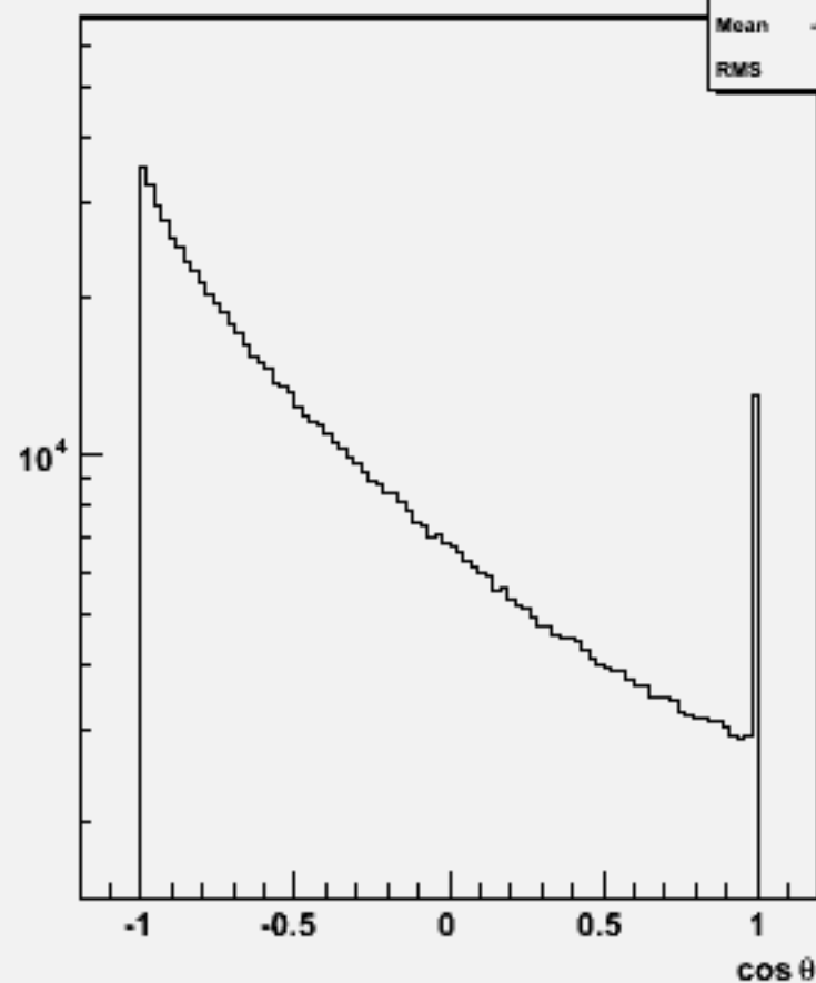
Particle cos \theta : w103743 ae1_e1cssc_o
