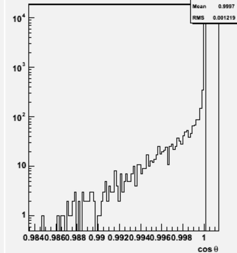
Jet cos \theta (All jets)w103743 ae1_e1cssc_o
