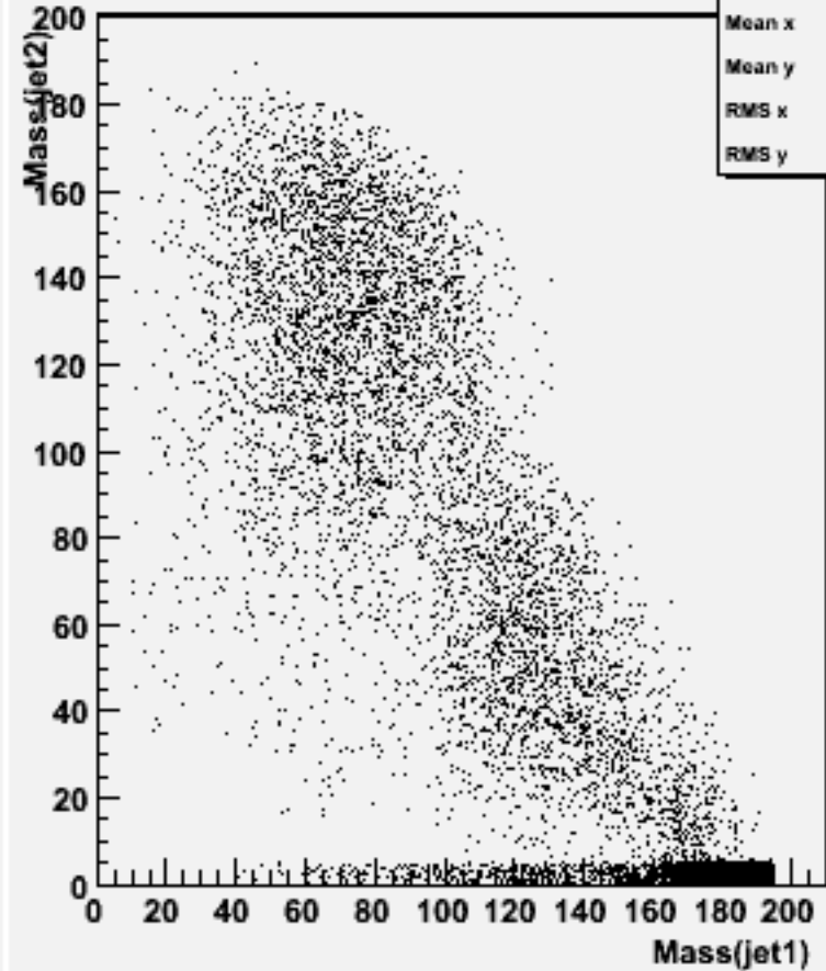
Jet mass for forced 2-jets : w103743 ae1_e1cssc_o
