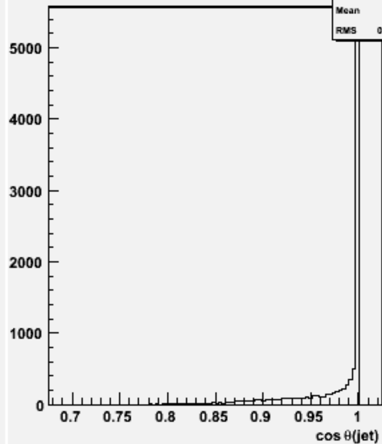
cos \theta for 2-jets :w103743 ae1_e1cssc_o
