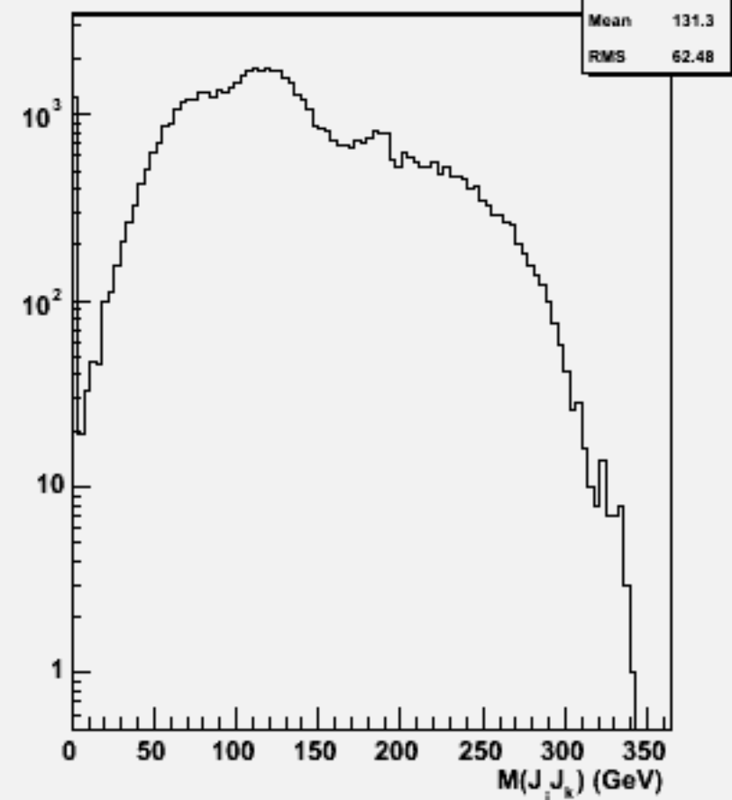
2jets mass(All comb)w103743 ae1_e1cssc_o
