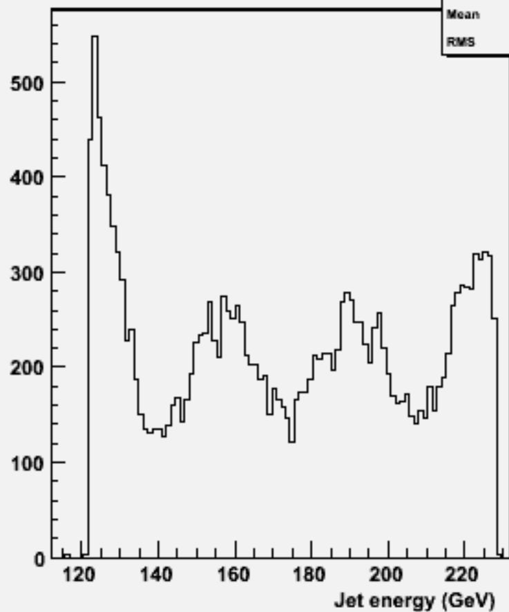
energy for 2-jets :w103743 ae1_e1cssc_o
