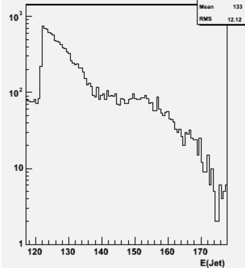
Jet energies(All jets)w103743 ae1_e1cssc_o
