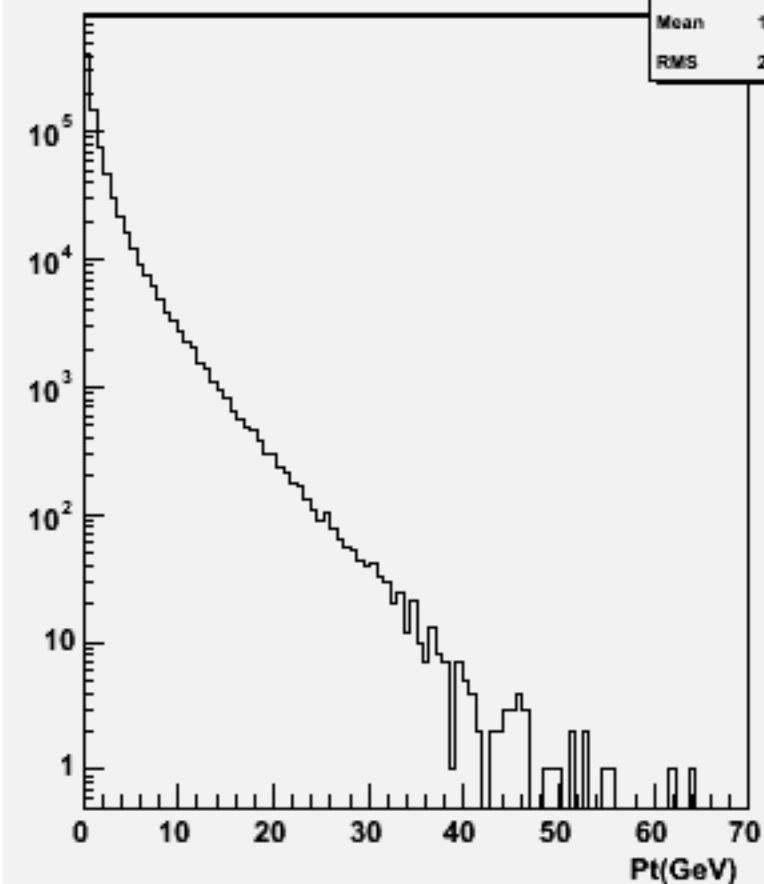
Particle Pt : w103743 ae1_e1cssc_o
