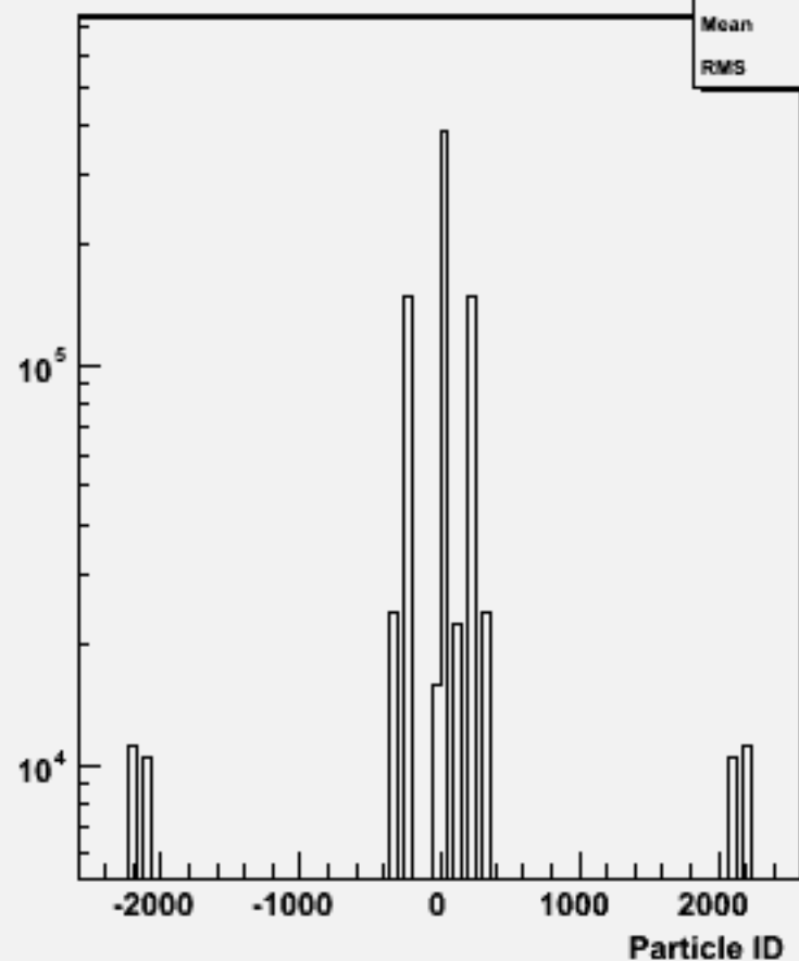
Particle ID : w103743 ae1_e1cssc_o
