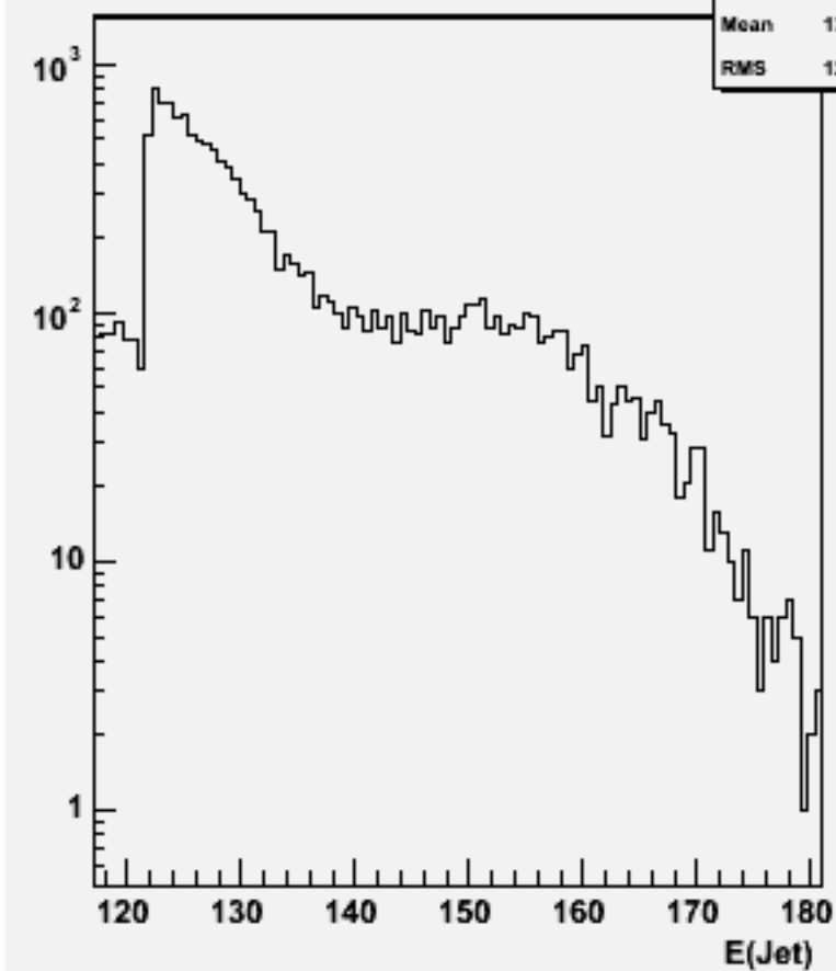
Jet energies(All jets)w103741 ae1_e1cssc_o
