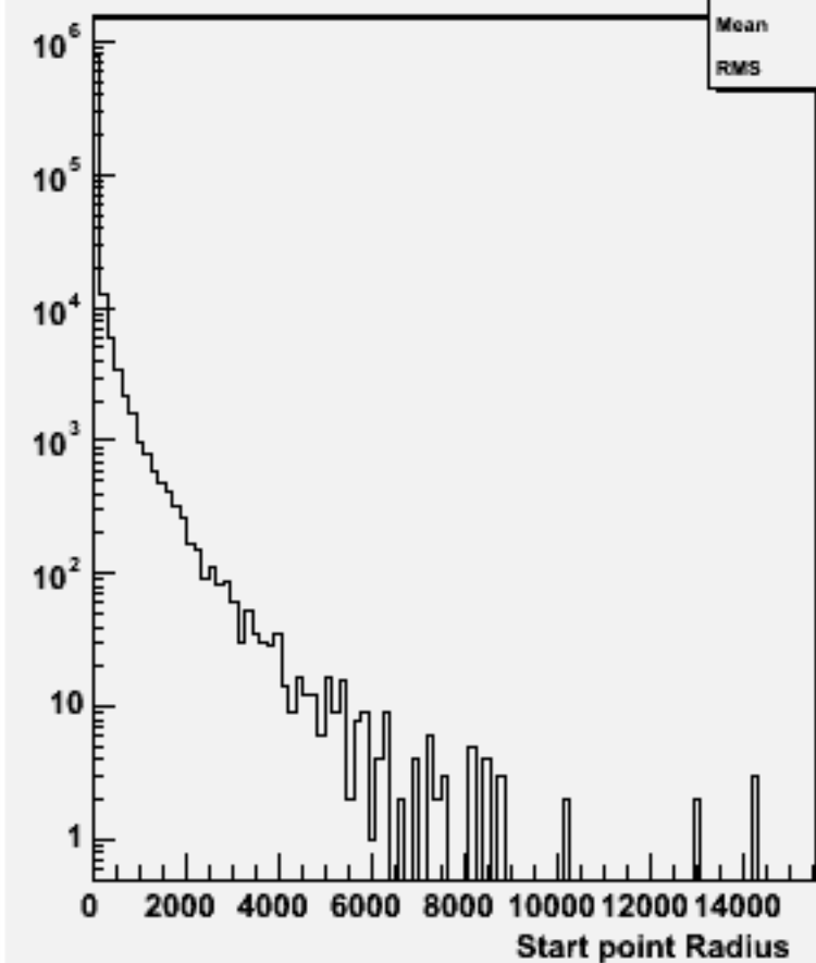
Start point R : w103741 ae1_e1cssc_o
