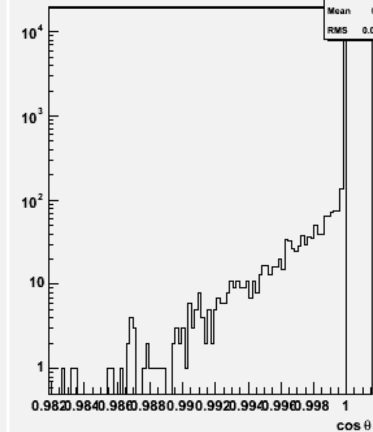
Jet cos \theta (All jets)w103741 ae1_e1cssc_o
