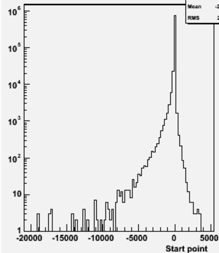
Start point Z : w103741 ae1_e1cssc_o
