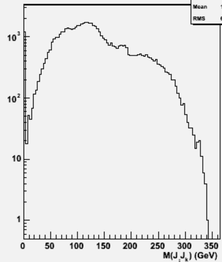
2jets mass(All comb)w103741 ae1_e1cssc_o
