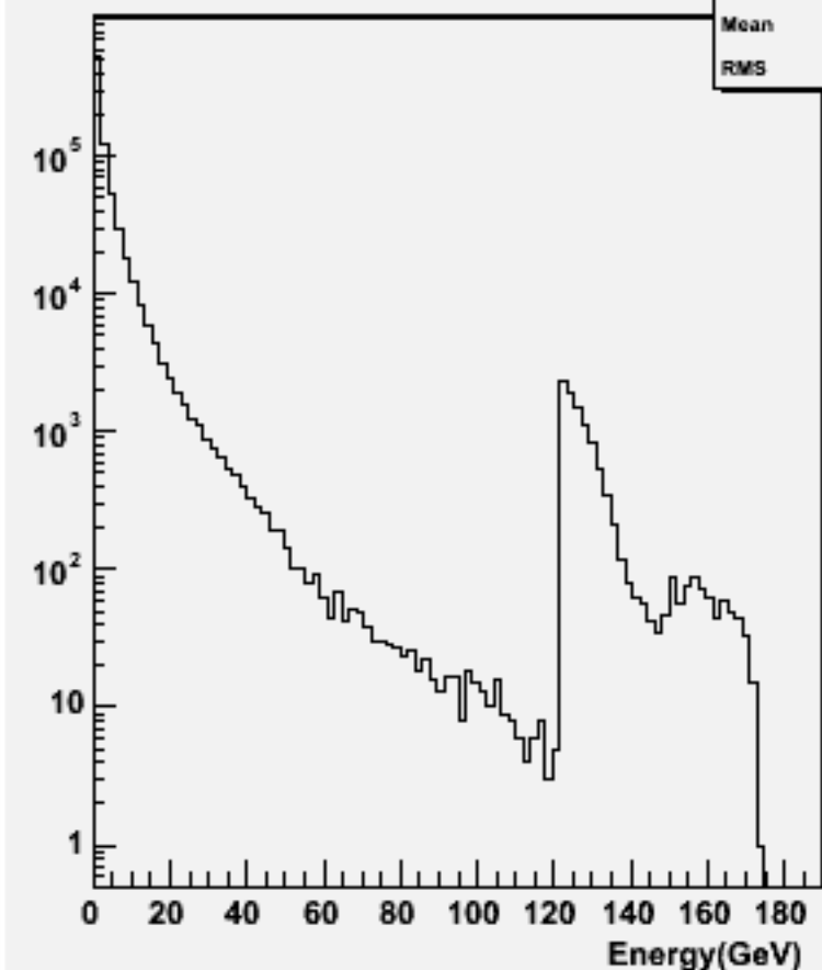
Particle Energy : w103741 ae1_e1cssc_o
