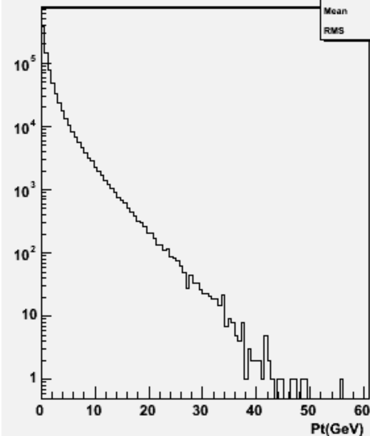
Particle Pt : w103741 ae1_e1cssc_o
