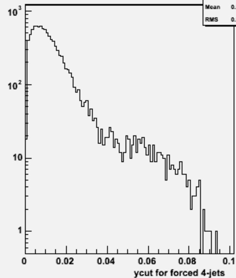
Ycut for 4-jets :w103741 ae1_e1cssc_o
