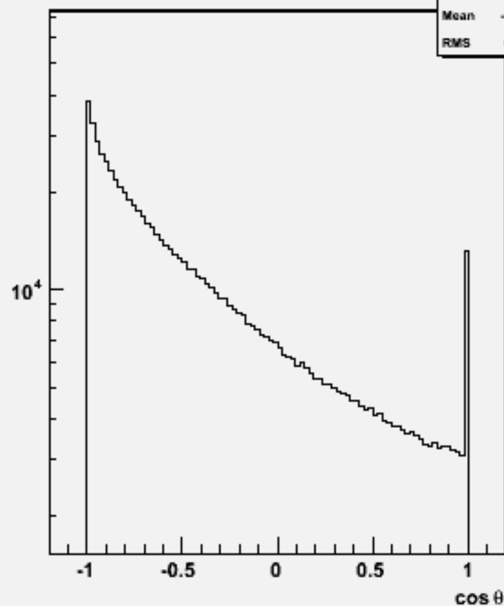
Particle \cos\theta : w103741 ae1_e1cssc_o
