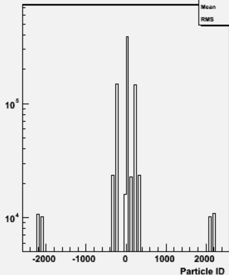
Particle ID : w103741 ae1_e1cssc_o
