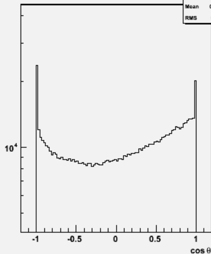
Particle cosθ : w103740 ae1_e1cssc_o
