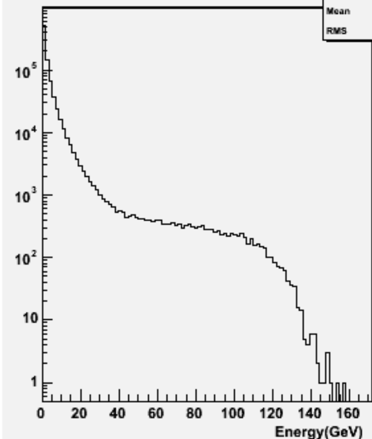
Particle Energy : w103740 ae1_e1cssc_o
