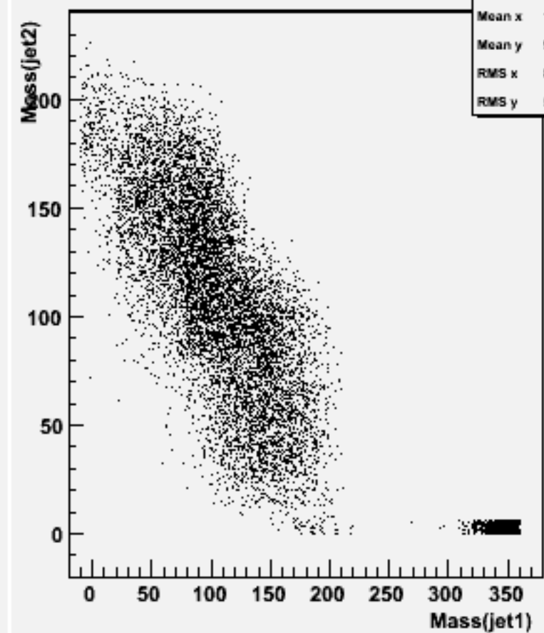
Jet mass for forced 2-jets : w103740 ae1_e1cssc_o
