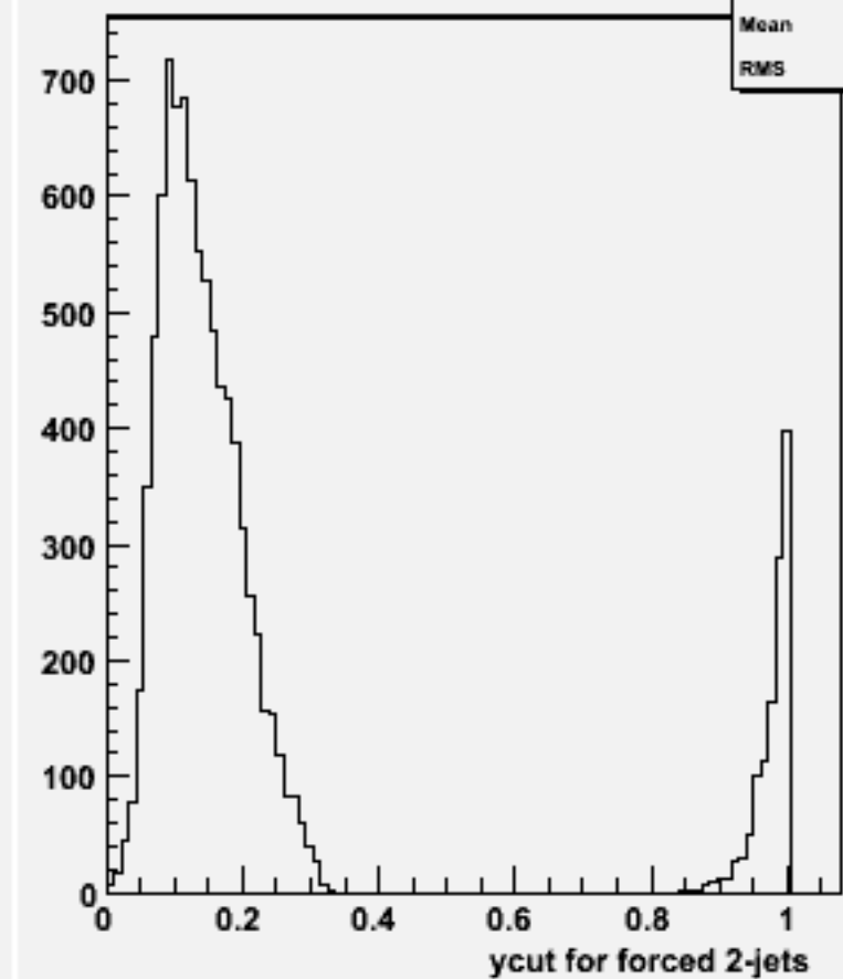
Ycut for 2-jets :w103740 ae1_e1cssc_o
