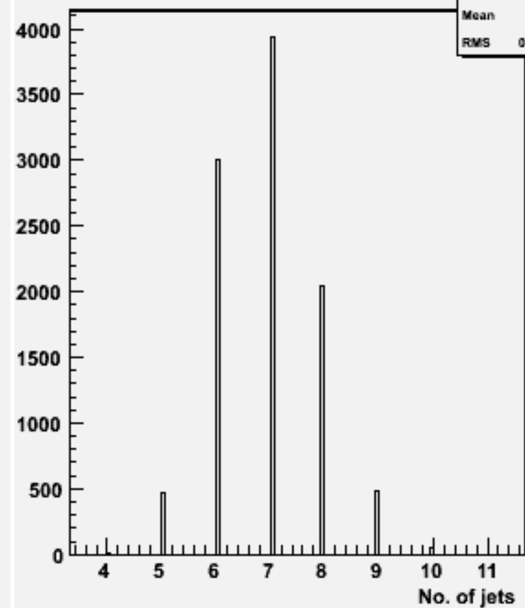
No. jets (ycut=0.001) : w103740 ae1_e1cssc_o
