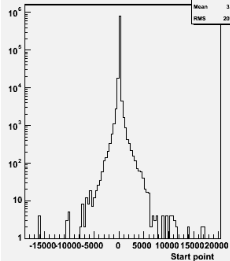
Start point Z : w103740 ae1_e1cssc_o
