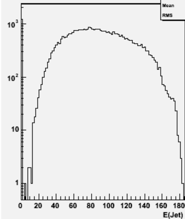
Jet energies(All jets)w103740 ae1_e1cssc_o
