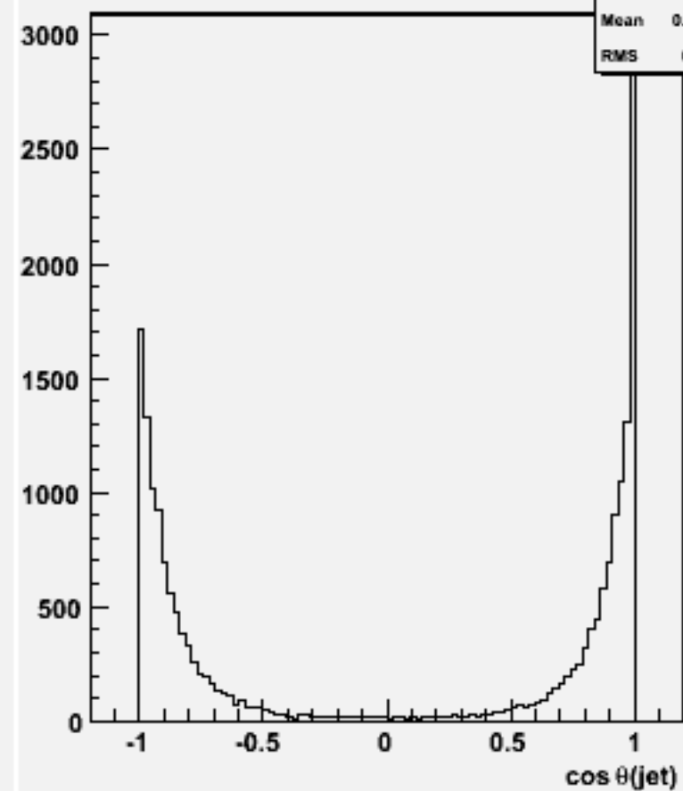
cos \theta for 2-jets :w103740 ae1_e1cssc_o
