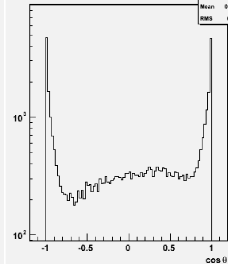
Jet cos \theta (All jets)w103740 ae1_e1cssc_o
