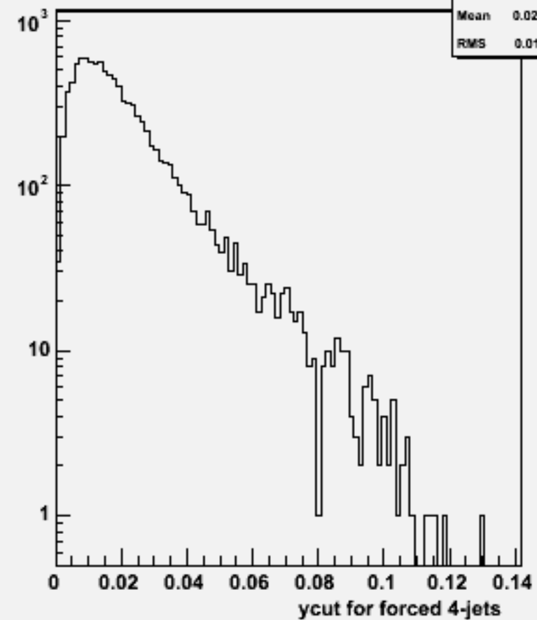
Ycut for 4-jets :w103740 ae1_e1cssc_o
