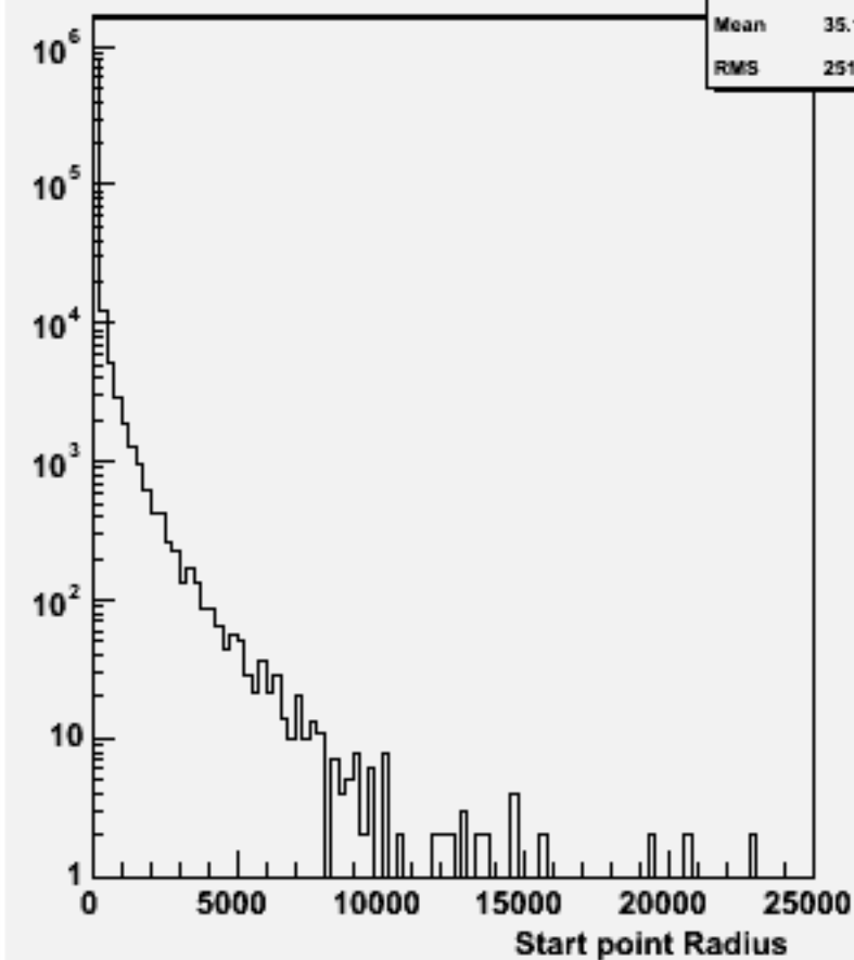
Start point R : w103740 ae1_e1cssc_o
