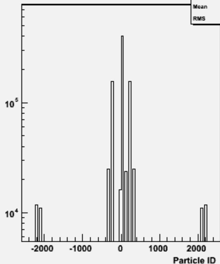
Particle ID : w103740 ae1_e1cssc_o
