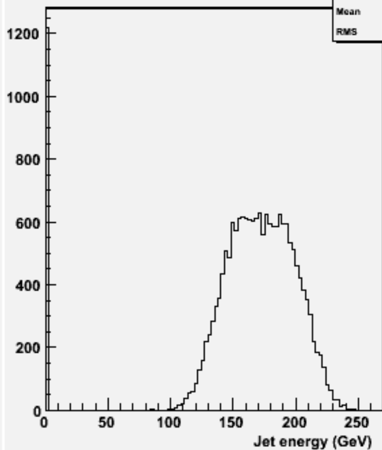
energy for 2-jets :w103740 ae1_e1cssc_o
