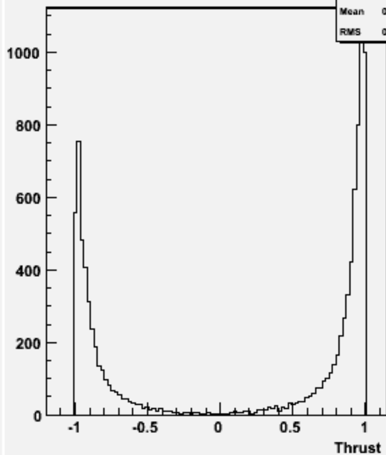
cos \Theta (thrust) w103740 ae1_e1cssc_o
