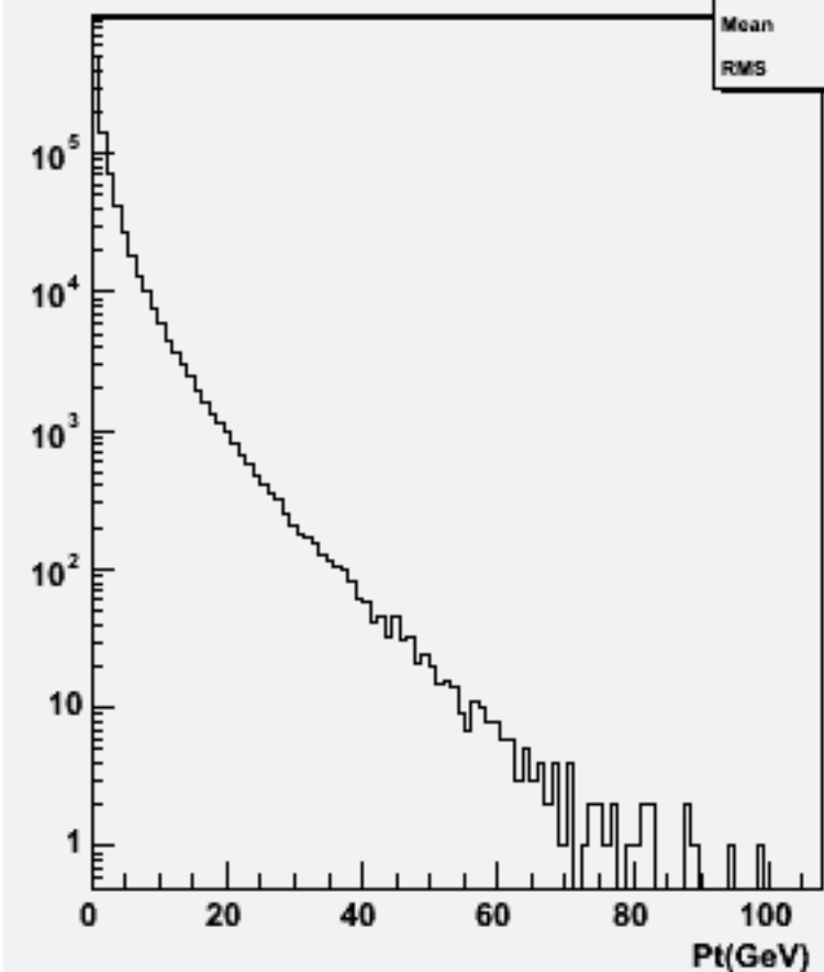
Particle Pt : w103740 ae1_e1cssc_o
