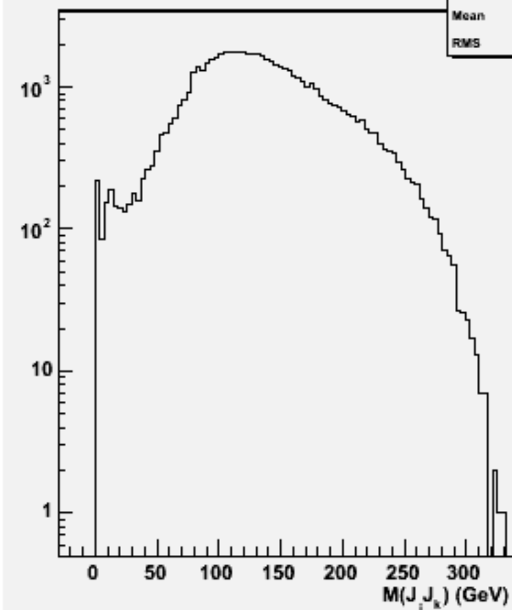
2jets mass(All comb)w103740 ae1_e1cssc_o
