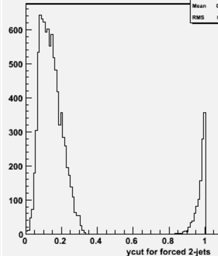
Ycut for 2-jets :w103738 ae1_e1csdu_o
