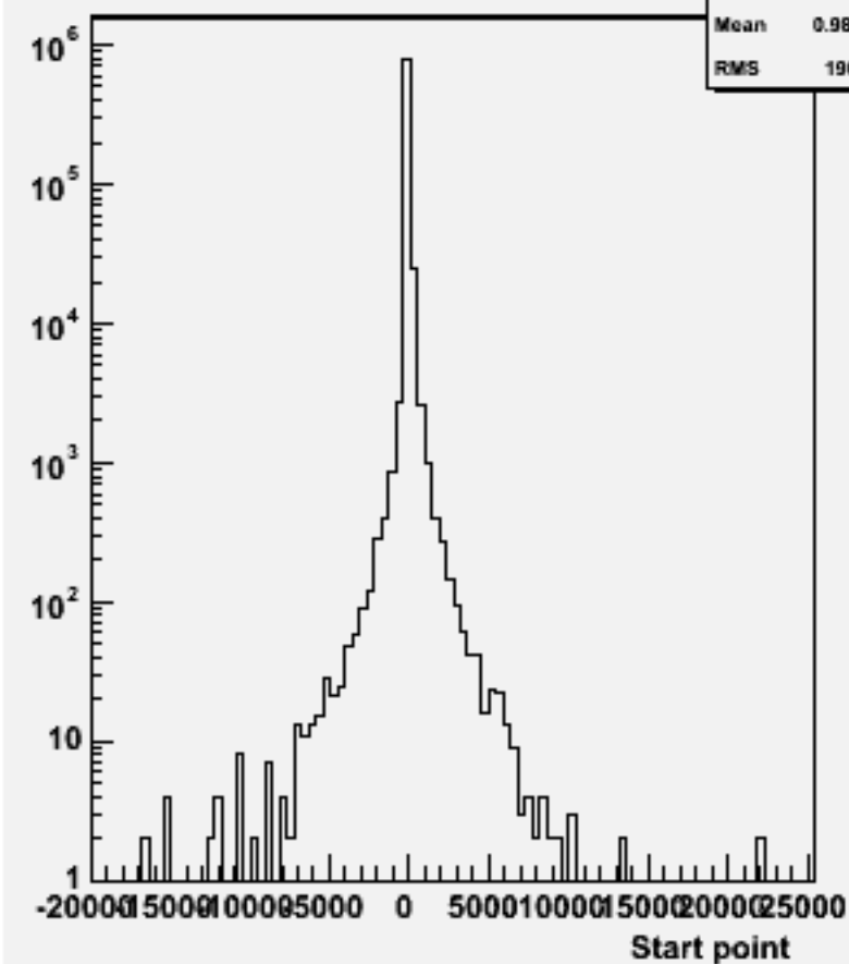
Start point Z : w103738 ae1_e1csdu_o
