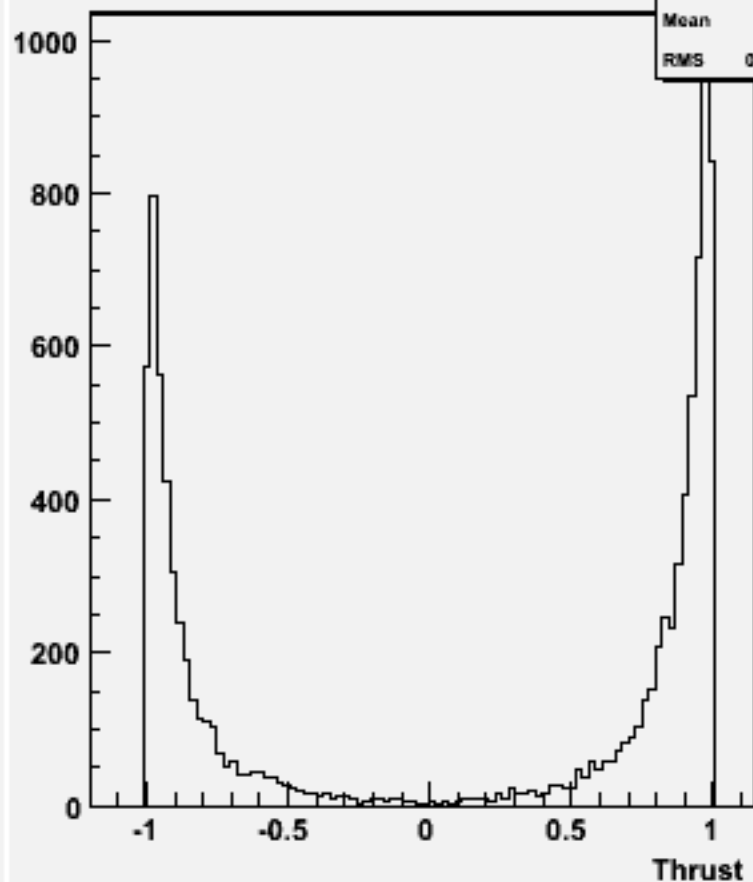
cos \Theta (thrust) w103738 ae1_e1csdu_o
