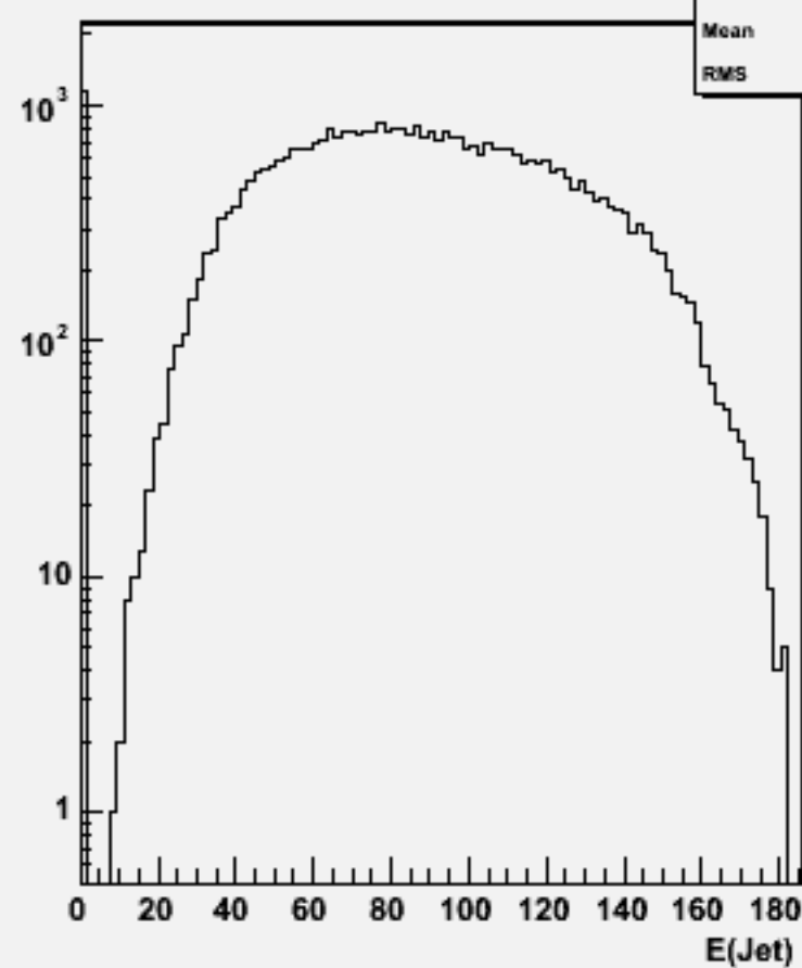
Jet energies(All jets)w103738 ae1_e1csdu_o
