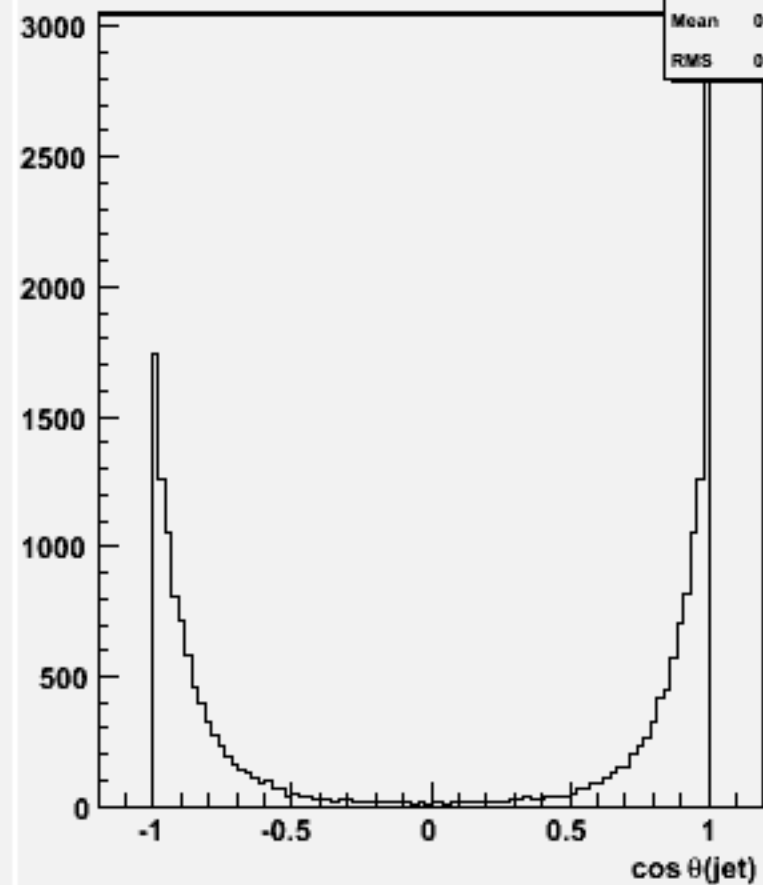
cos \theta for 2-jets :w103738 ae1_e1csdu_o
