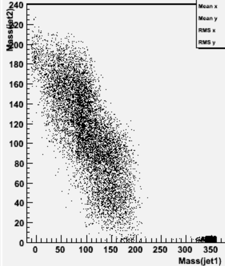
Jet mass for forced 2-jets : w103738 ae1_e1csdu_o
