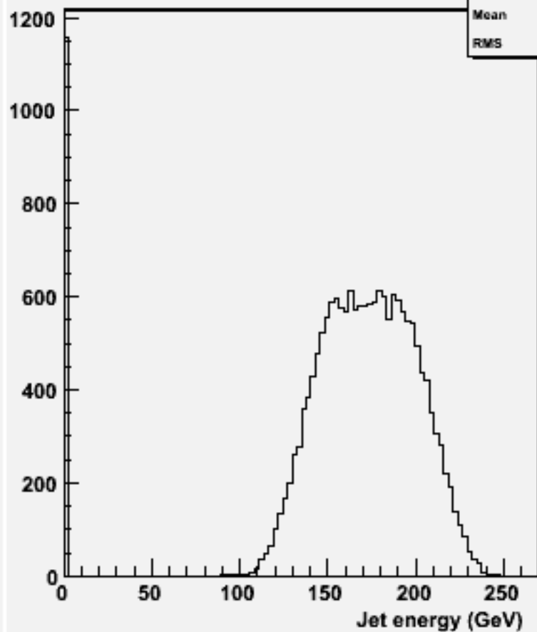
energy for 2-jets :w103738 ae1_e1csdu_o
