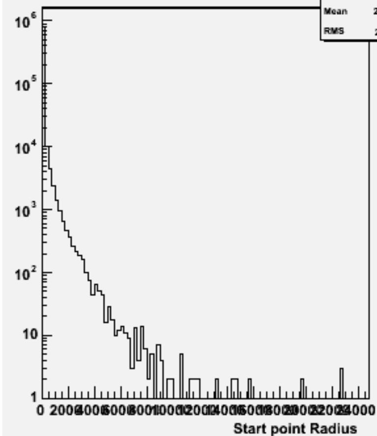
Start point R : w103738 ae1_e1csdu_o
