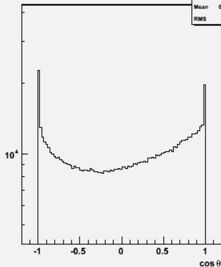
Particle cosθ : w103738 ae1_e1csdu_o
