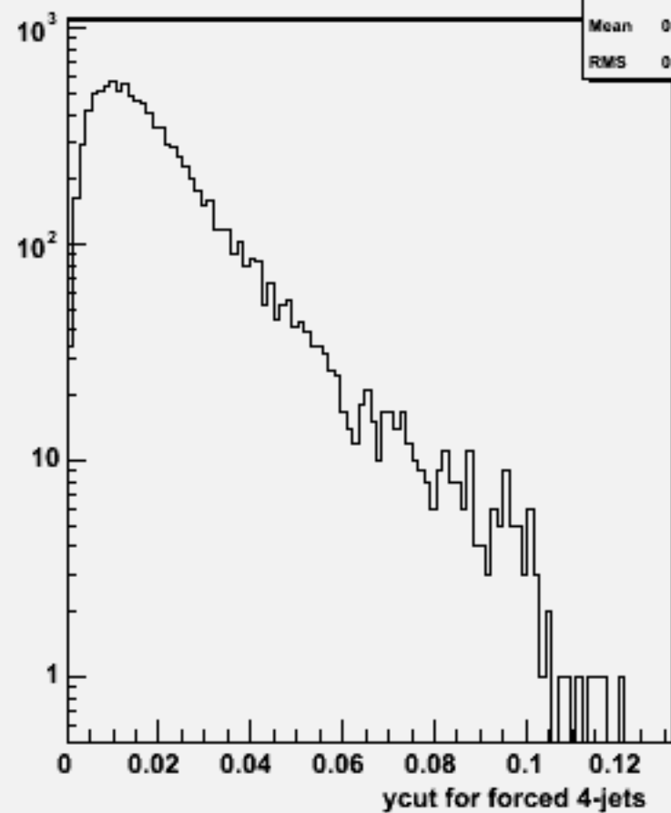
Ycut for 4-jets :w103738 ae1_e1csdu_o
