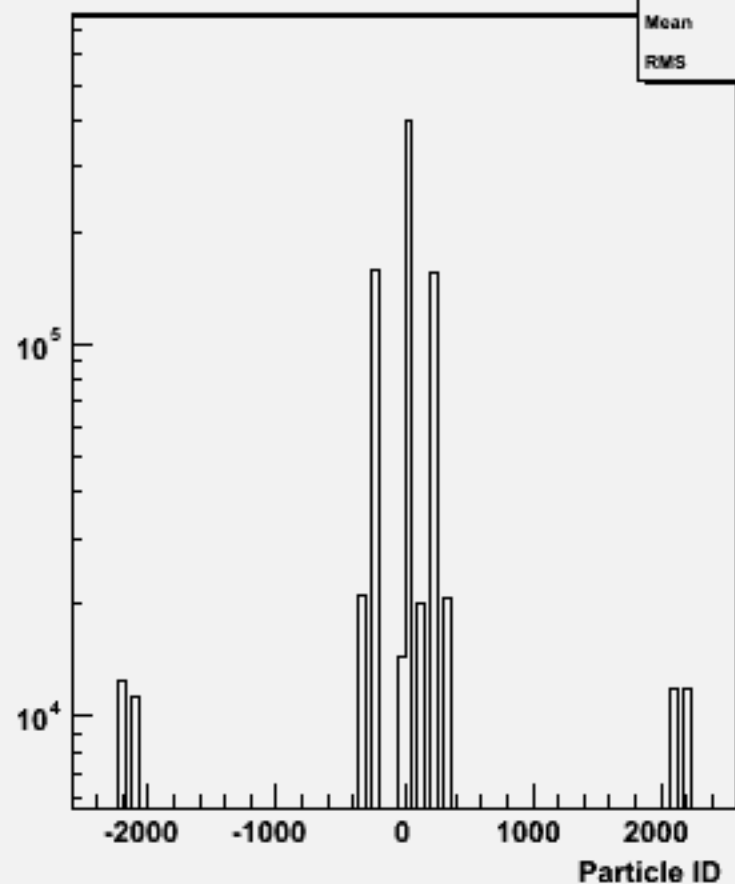
Particle ID : w103738 ae1_e1csdu_o
