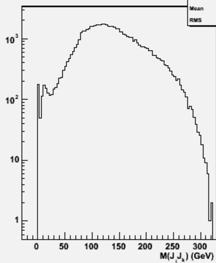
2jets mass(All comb)w103738 ae1_e1csdu_o
