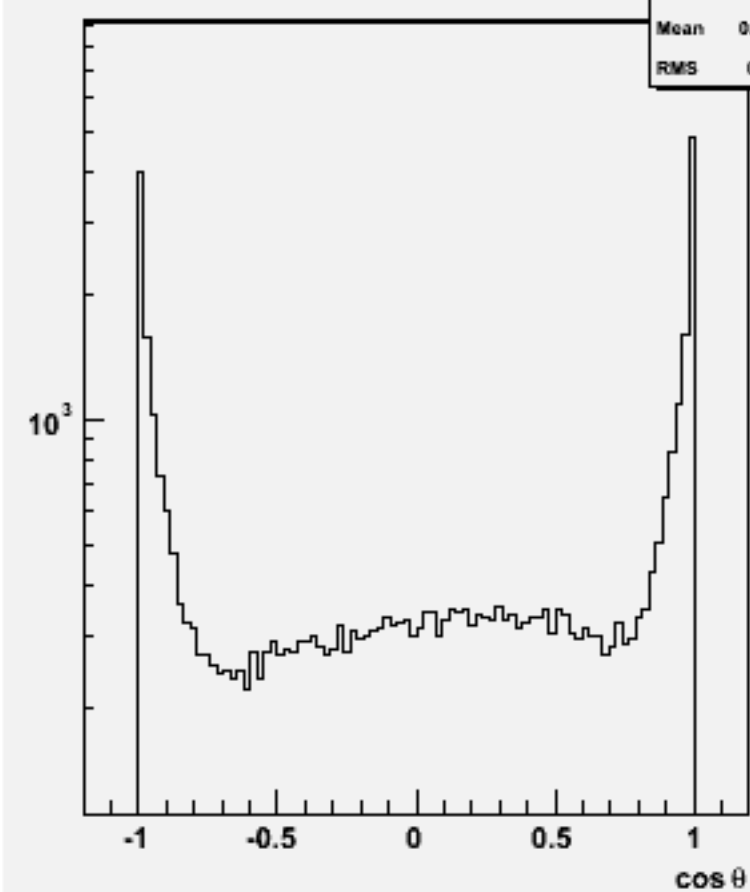
Jet cos \theta (All jets)w103738 ae1_e1csdu_o
