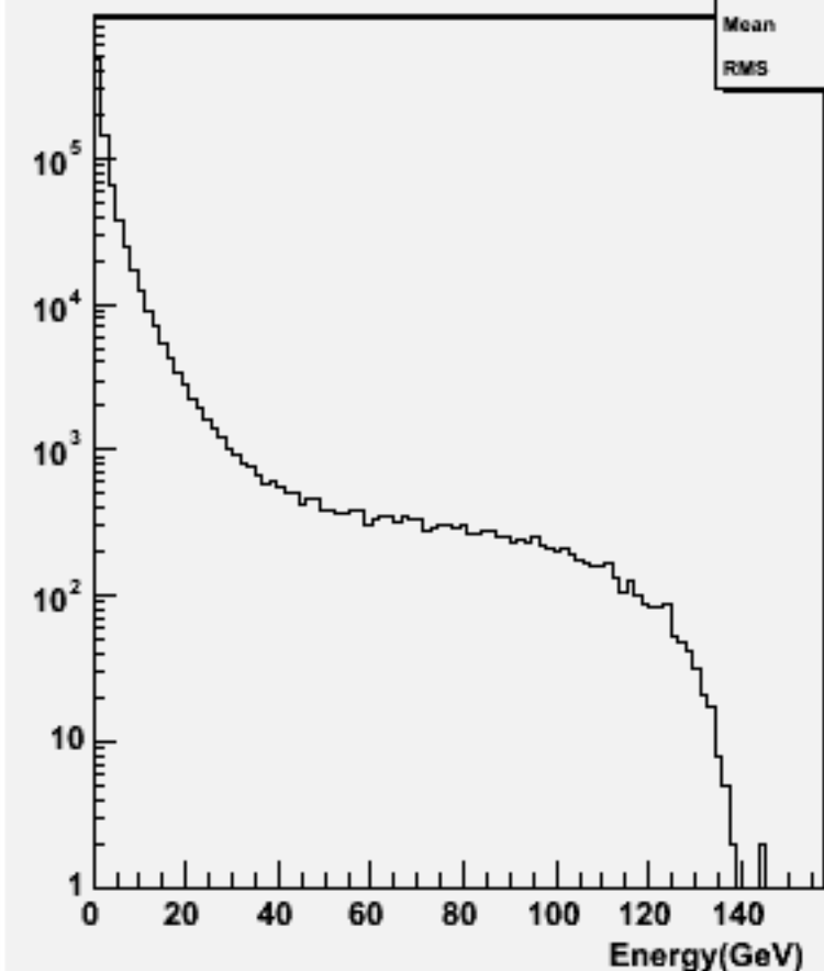
Particle Energy : w103738 ae1_e1csdu_o
