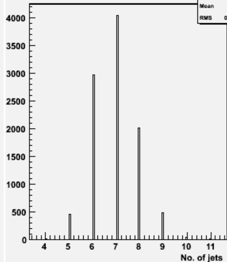
No. jets (ycut=0.001) : w103738 ae1_e1csdu_o
