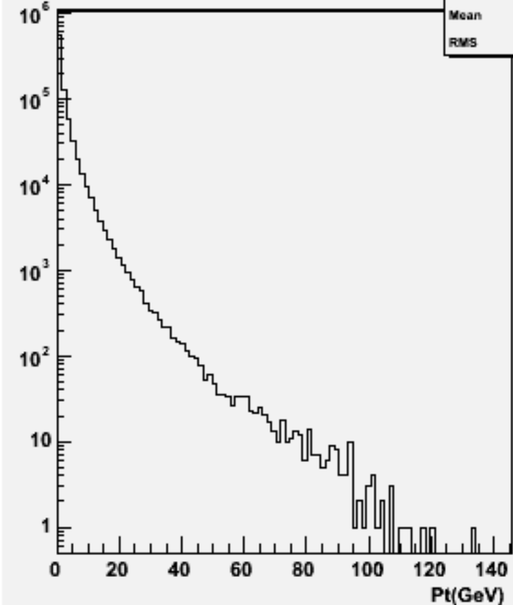
Particle Pt : w103738 ae1_e1csdu_o
