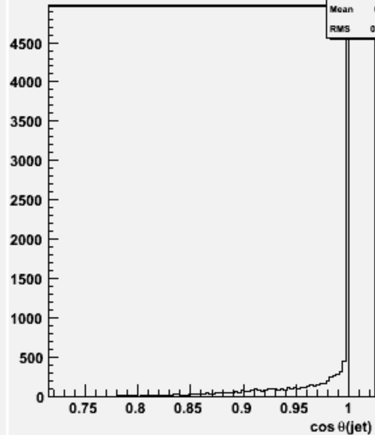
cos \theta for 2-jets :w103737 ae1_e1csdu_o
