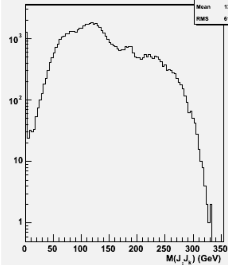
2jets mass(All comb)w103737 ae1_e1csdu_o
