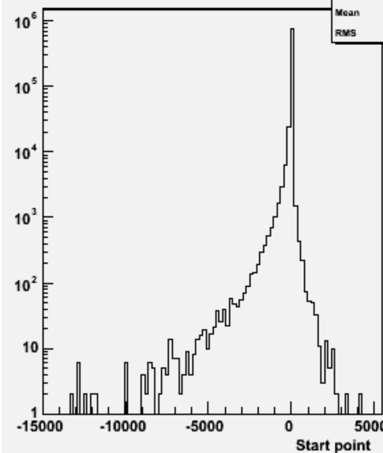
Start point Z : w103737 ae1_e1csdu_o
