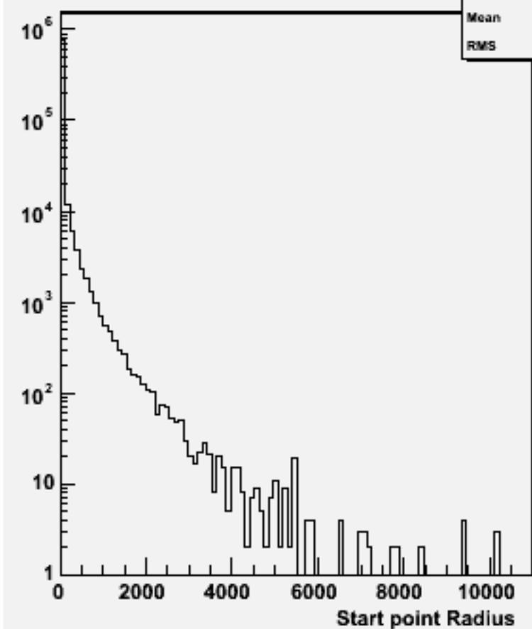
Start point R : w103737 ae1_e1csdu_o
