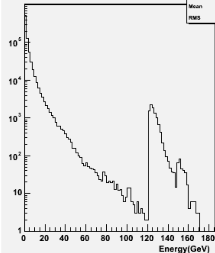
Particle Energy : w103737 ae1_e1csdu_o
