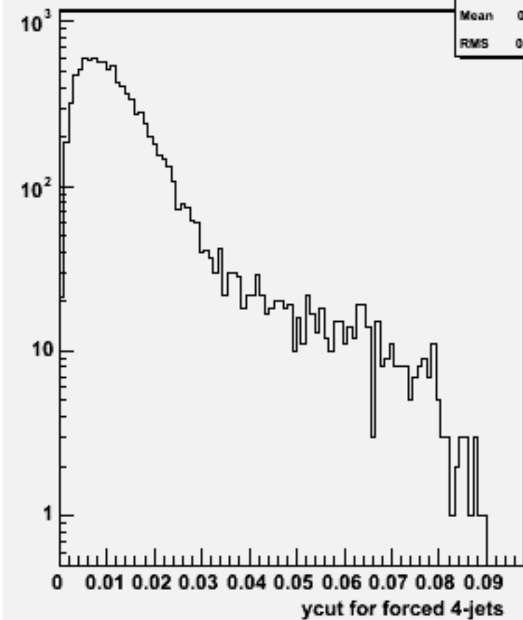
Ycut for 4-jets :w103737 ae1_e1csdu_o
