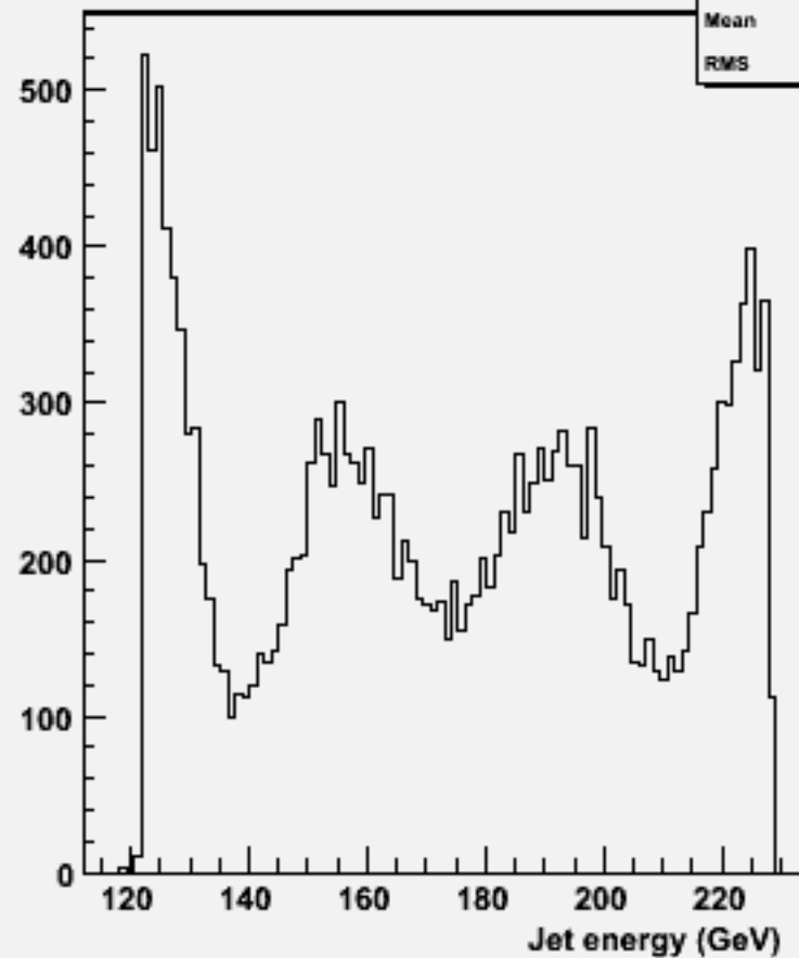
energy for 2-jets :w103737 ae1_e1csdu_o
