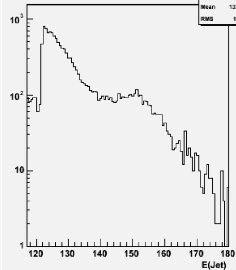
Jet energies(All jets)w103737 ae1_e1csdu_o
