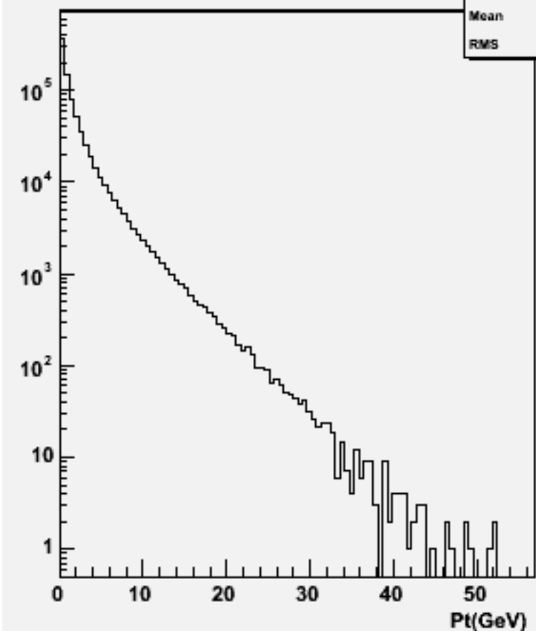
Particle Pt : w103737 ae1_e1csdu_o
