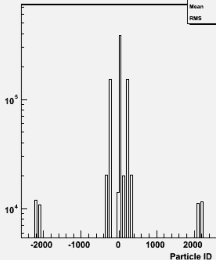
Particle ID : w103737 ae1_e1csdu_o
