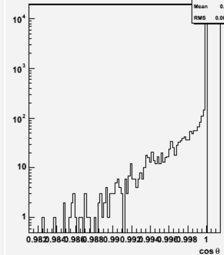
Jet cos \theta (All jets)w103737 ae1_e1csdu_o
