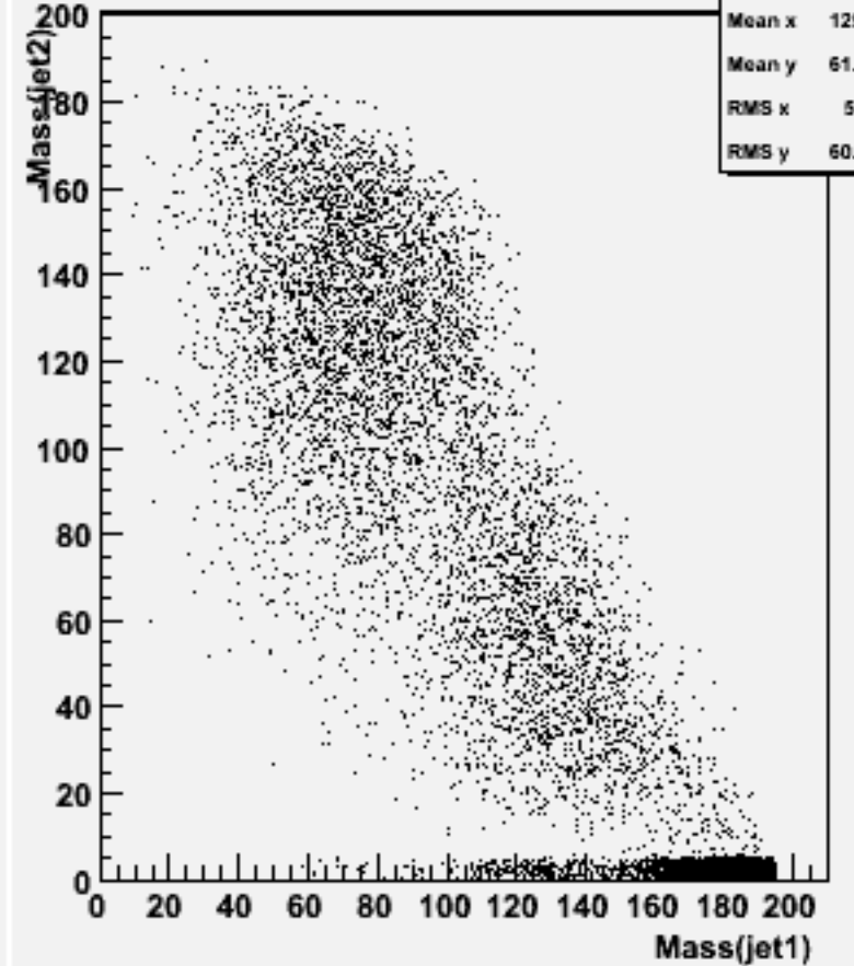
Jet mass for forced 2-jets : w103737 ae1_e1csdu_o
