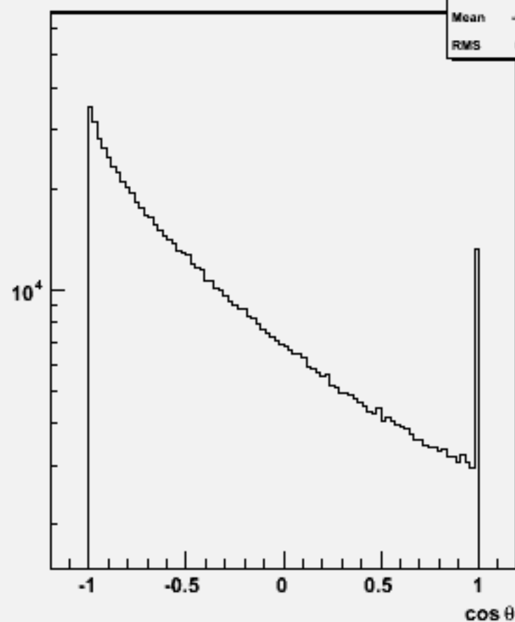
Particle cosθ : w103737 ae1_e1csdu_o
