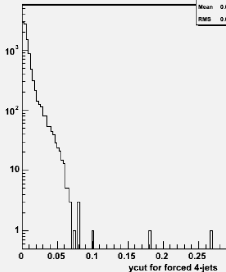
Ycut for 4-jets :w103735 ae1_e1cse3n3_o
