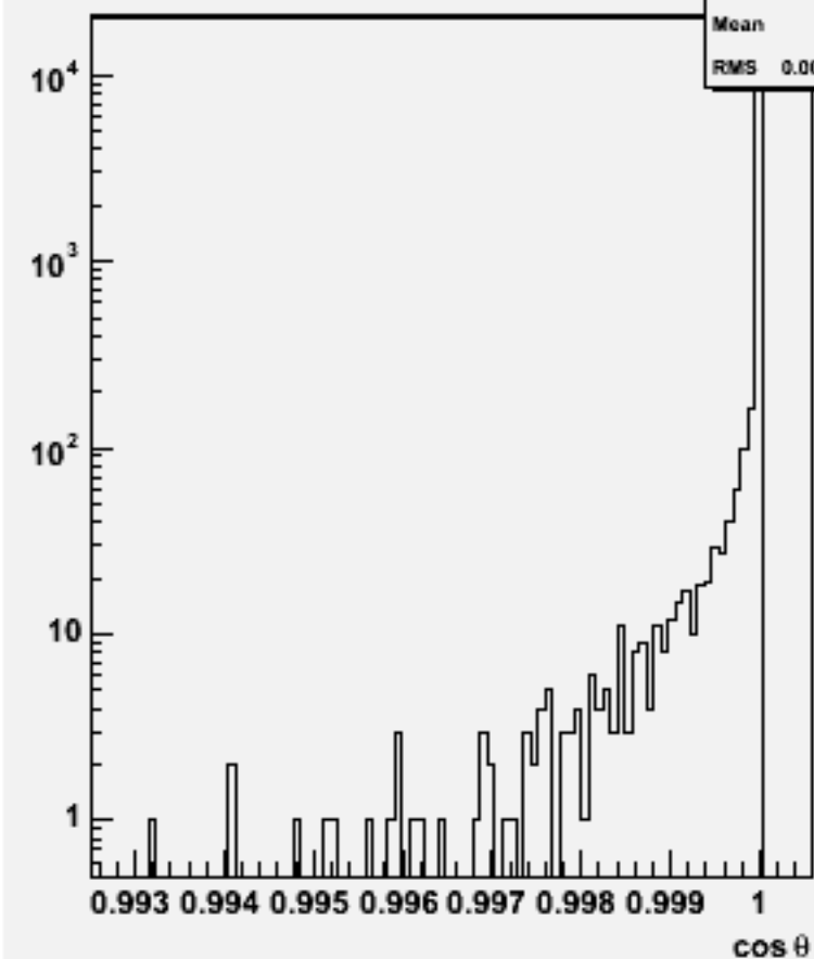
Jet cos \theta (All jets)w103735 ae1_e1cse3n3_o
