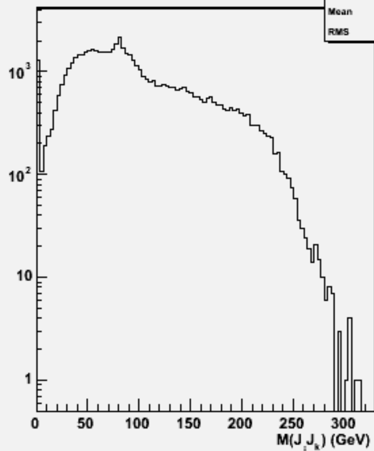
2jets mass(All comb)w103735 ae1_e1cse3n3_o
