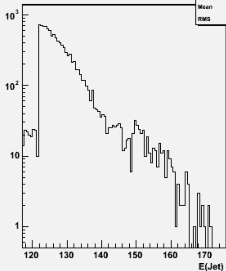
Jet energies(All jets)w103735 ae1_e1cse3n3_o
