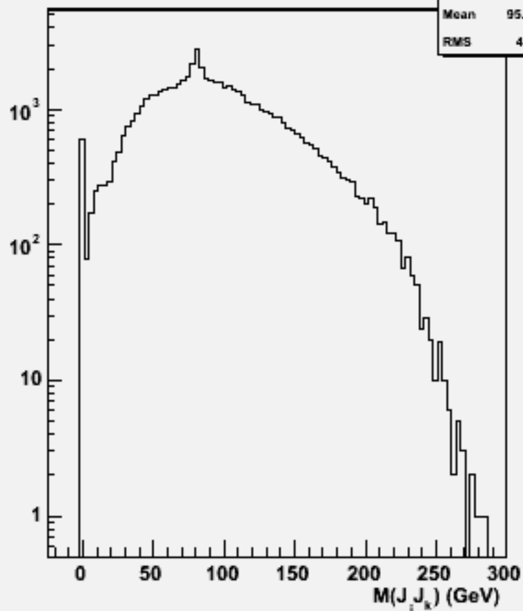
2jets mass(All comb)w103734 ae1_e1cse3n3_o
