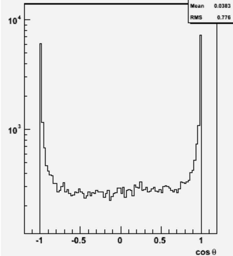
Jet cos \theta (All jets)w103734 ae1_e1cse3n3_o
