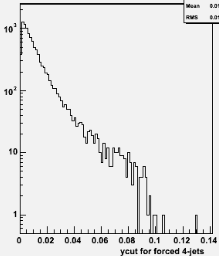
Ycut for 4-jets :w103734 ae1_e1cse3n3_o
