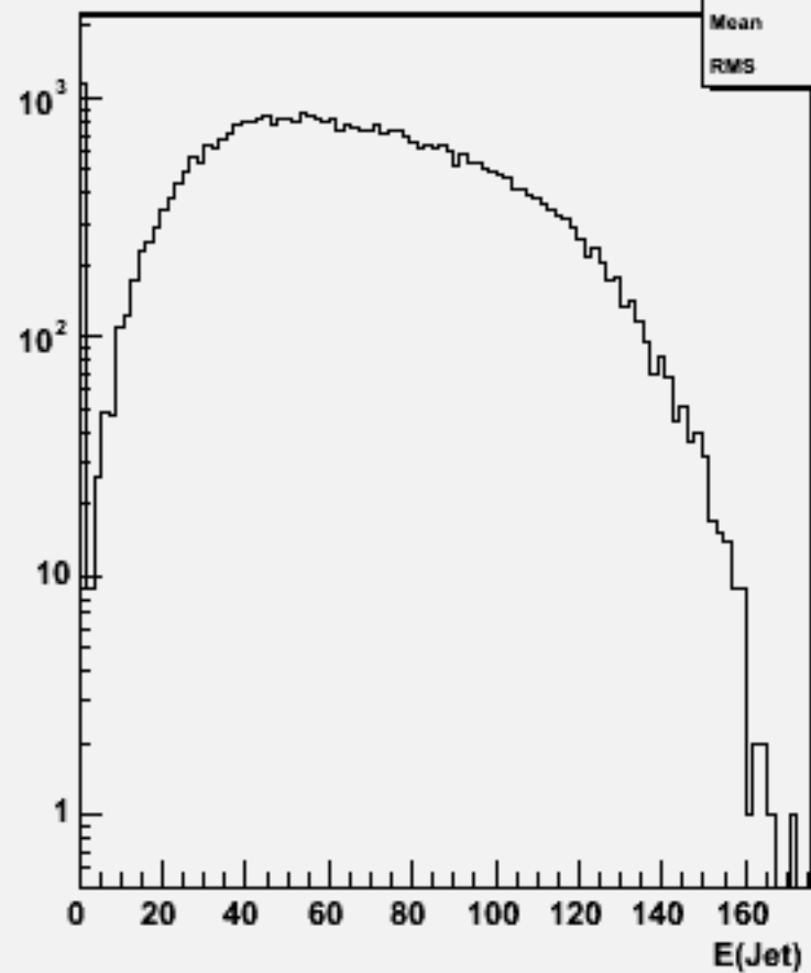
Jet energies(All jets)w103734 ae1_e1cse3n3_o
