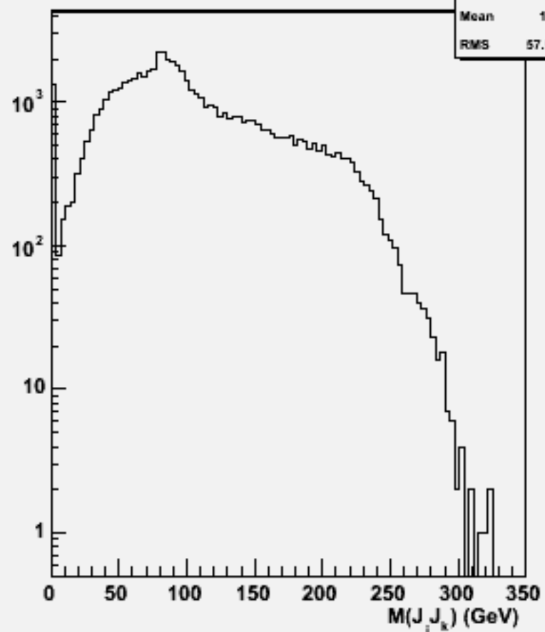
2jets mass(All comb)w103731 ae1_e1cse2n2_o
