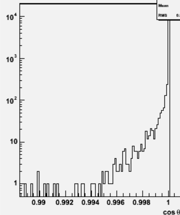
Jet cos \theta (All jets)w103731 ae1_e1cse2n2_o
