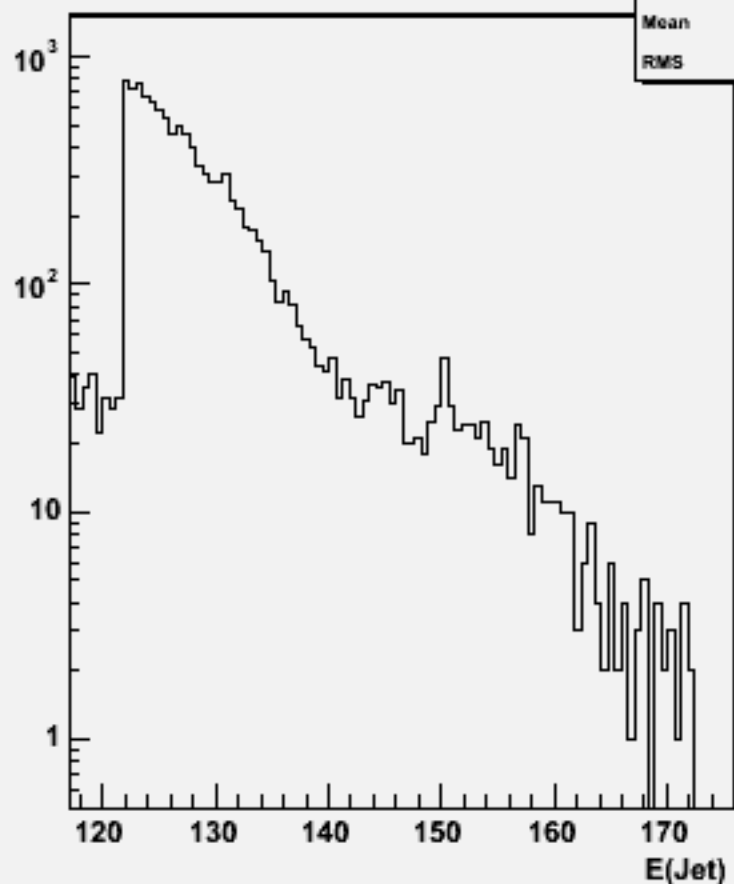
Jet energies(All jets)w103731 ae1_e1cse2n2_o
