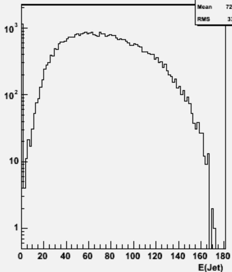
Jet energies(All jets)w103730 ae1_e1cse2n2_o
