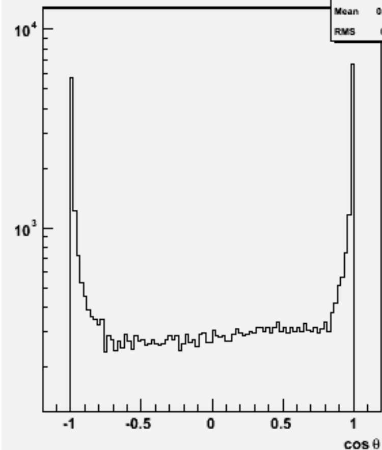
Jet cos \theta (All jets)w103730 ae1_e1cse2n2_o
