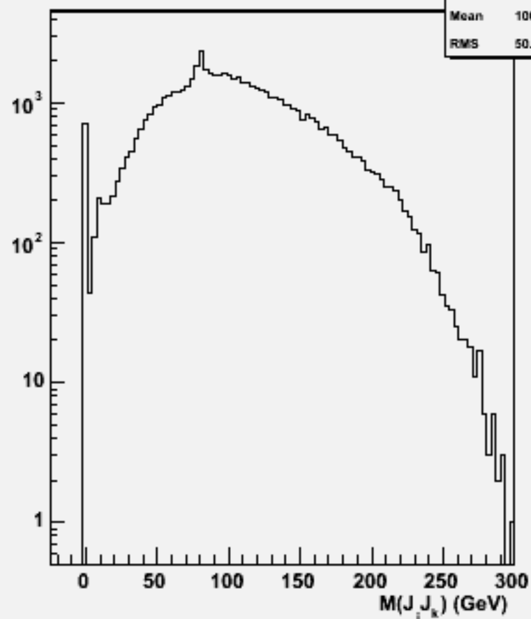
2jets mass(All comb)w103730 ae1_e1cse2n2_o
