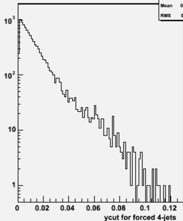
Ycut for 4-jets :w103730 ae1_e1cse2n2_o
