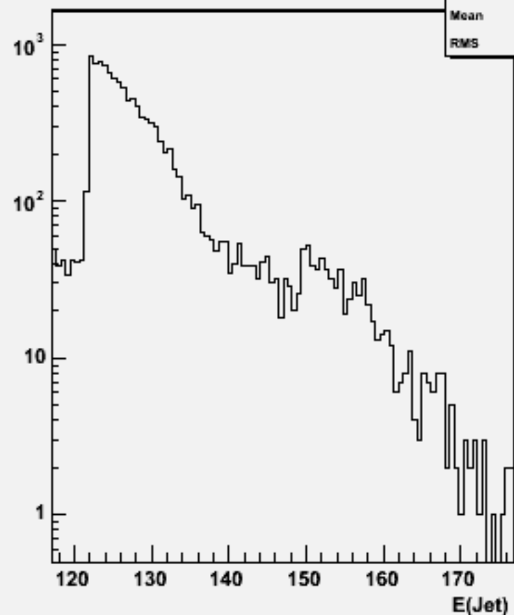
Jet energies(All jets)w103729 ae1_e1cse2n2_o
