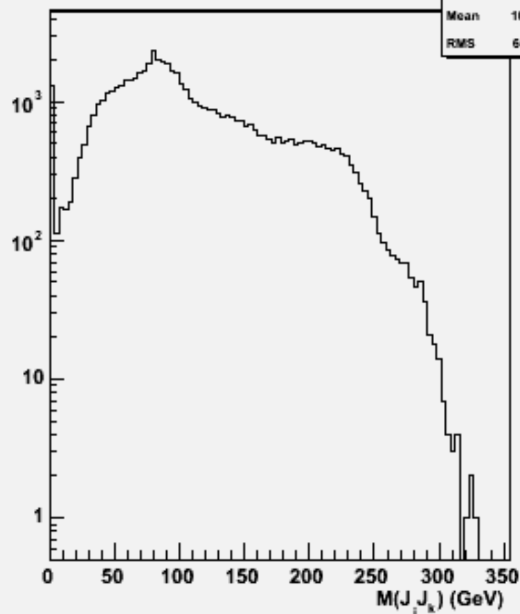
2jets mass(All comb)w103729 ae1_e1cse2n2_o
