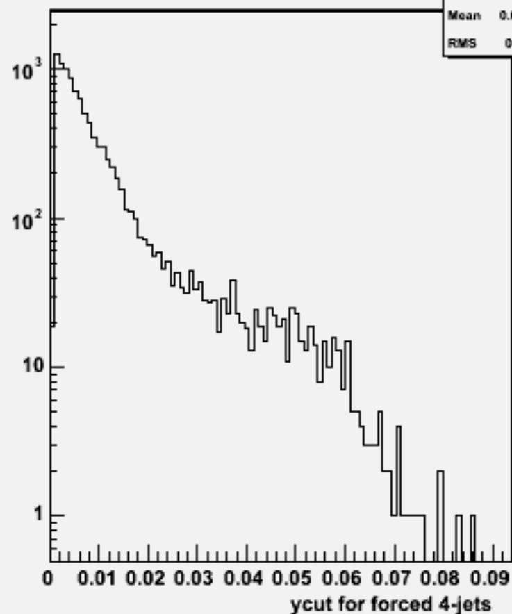
Ycut for 4-jets :w103729 ae1_e1cse2n2_o
