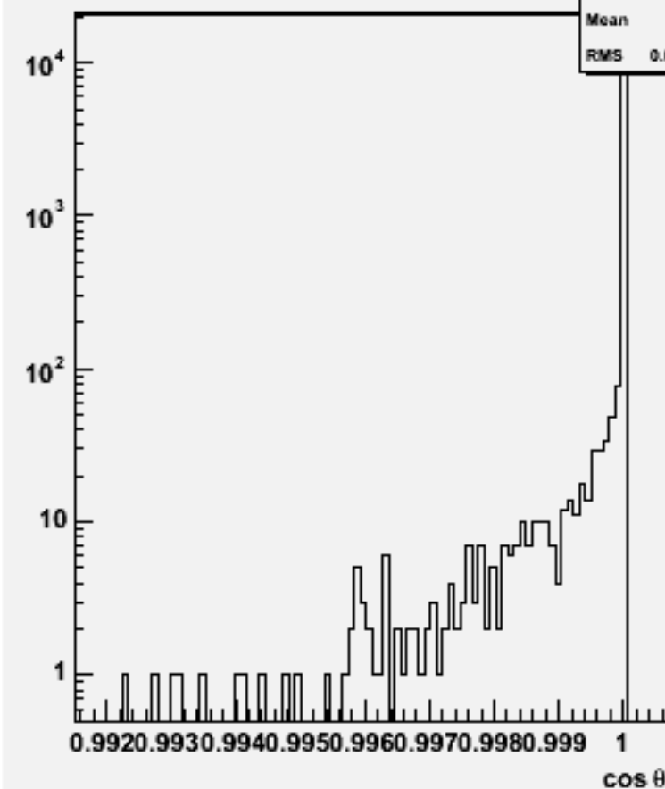
Jet cos \theta (All jets)w103729 ae1_e1cse2n2_o
