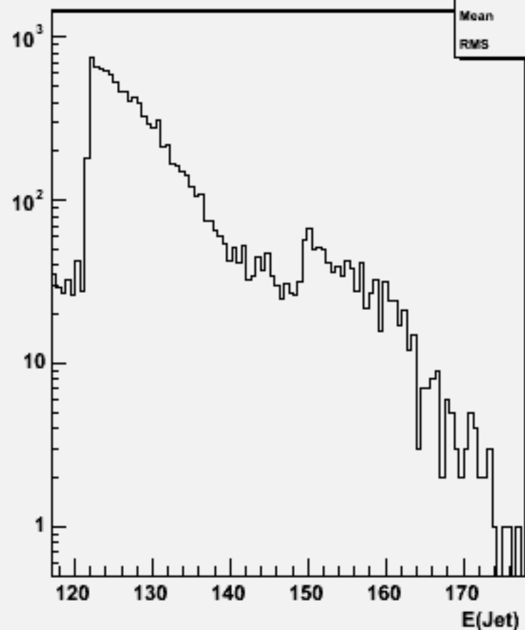
Jet energies(All jets)w103727 ae1_e1cse1n1_o
