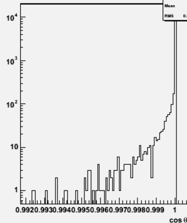
Jet cos \theta (All jets)w103727 ae1_e1cse1n1_o
