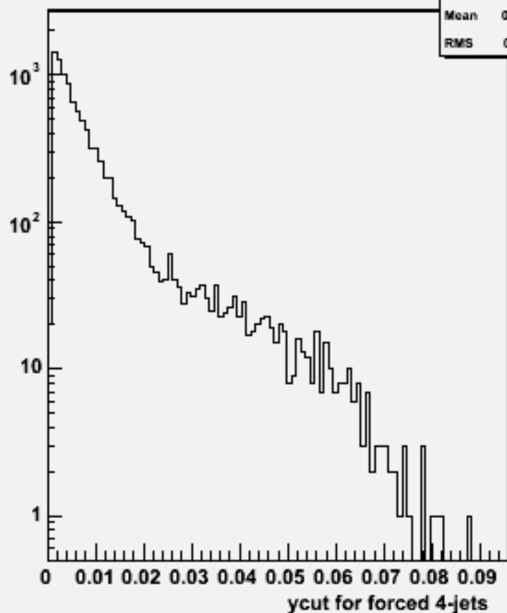
Ycut for 4-jets :w103727 ae1_e1cse1n1_o
