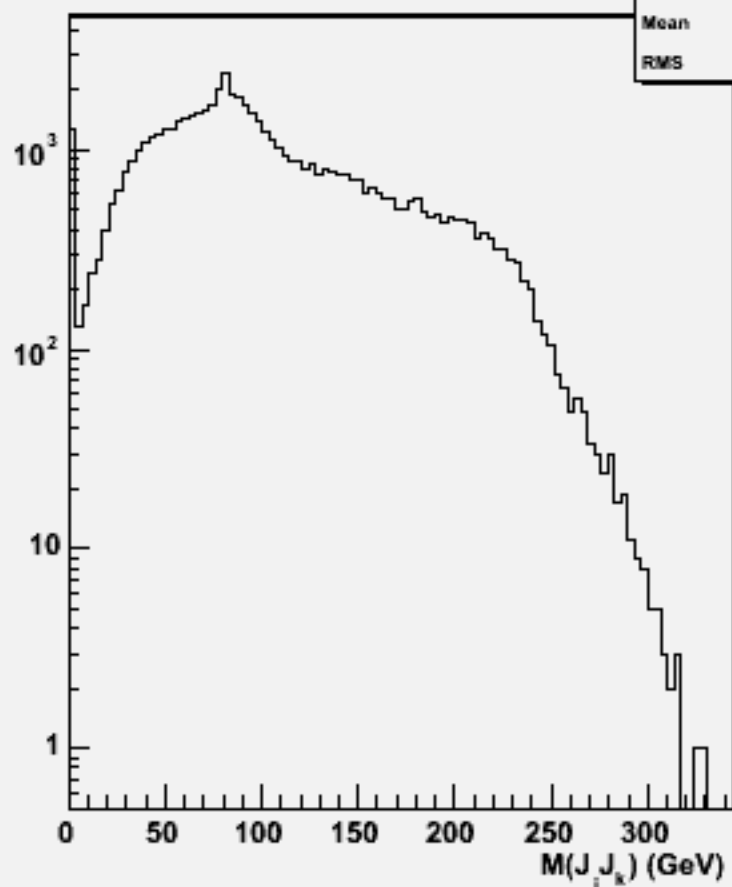
2jets mass(All comb)w103727 ae1_e1cse1n1_o
