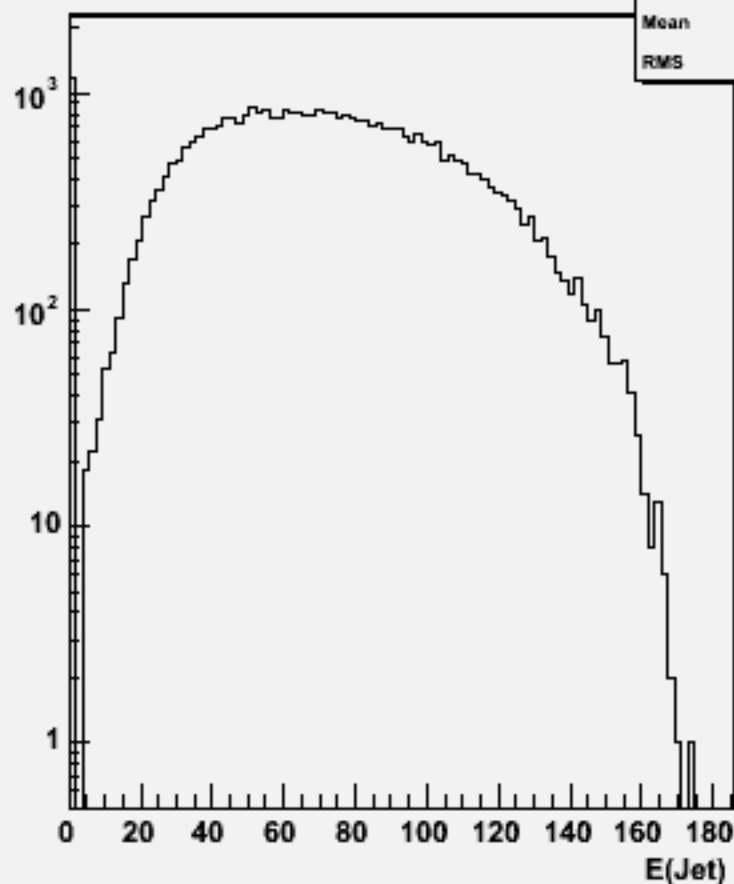
Jet energies(All jets)w103726 ae1_e1cse1n1_o
