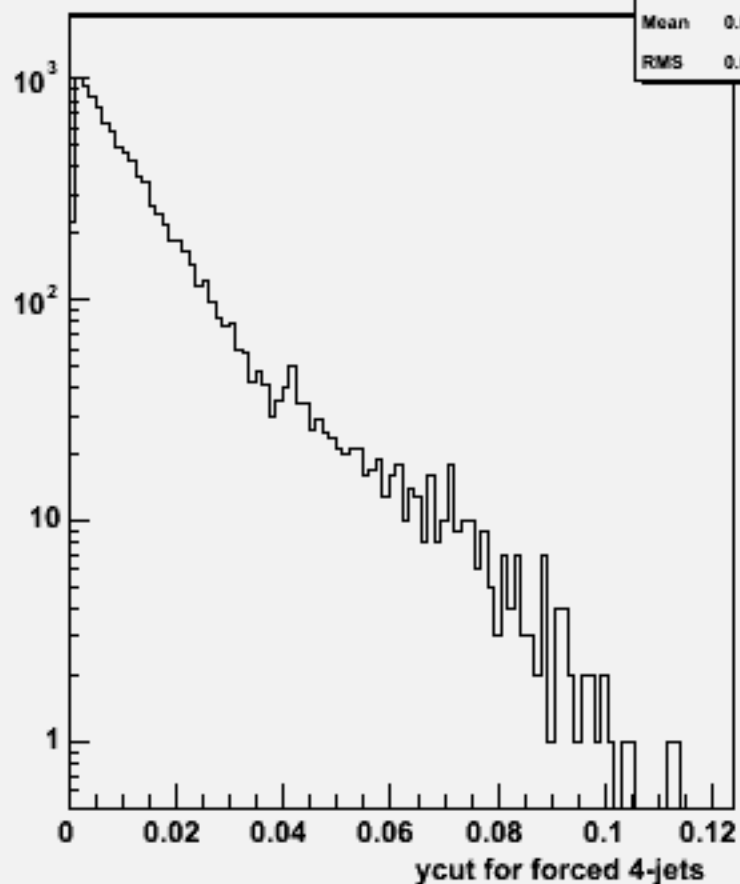
Ycut for 4-jets :w103726 ae1_e1cse1n1_o
