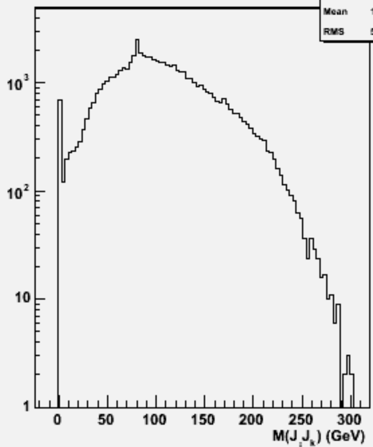
2jets mass(All comb)w103726 ae1_e1cse1n1_o
