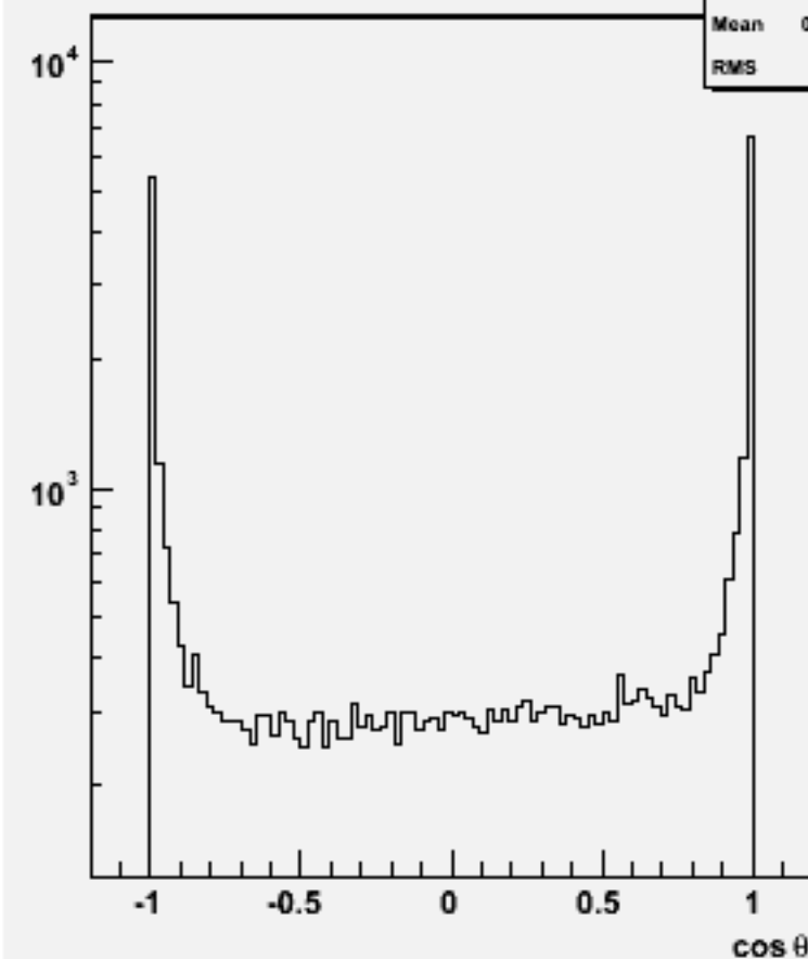
Jet cos \theta (All jets)w103726 ae1_e1cse1n1_o
