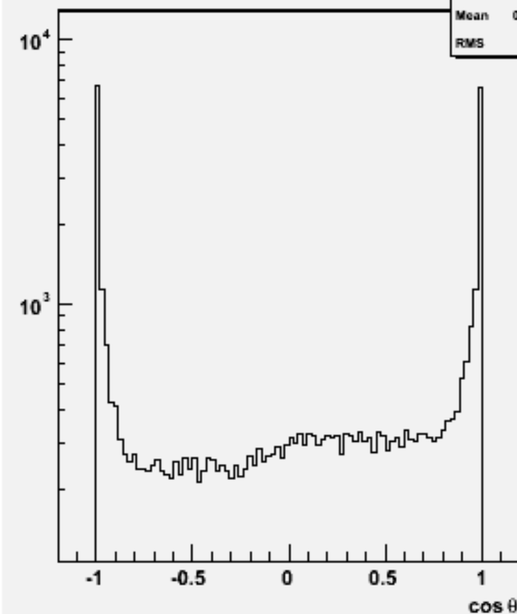
Jet cos \theta (All jets)w103724 ae1_e1cse1n1_o
