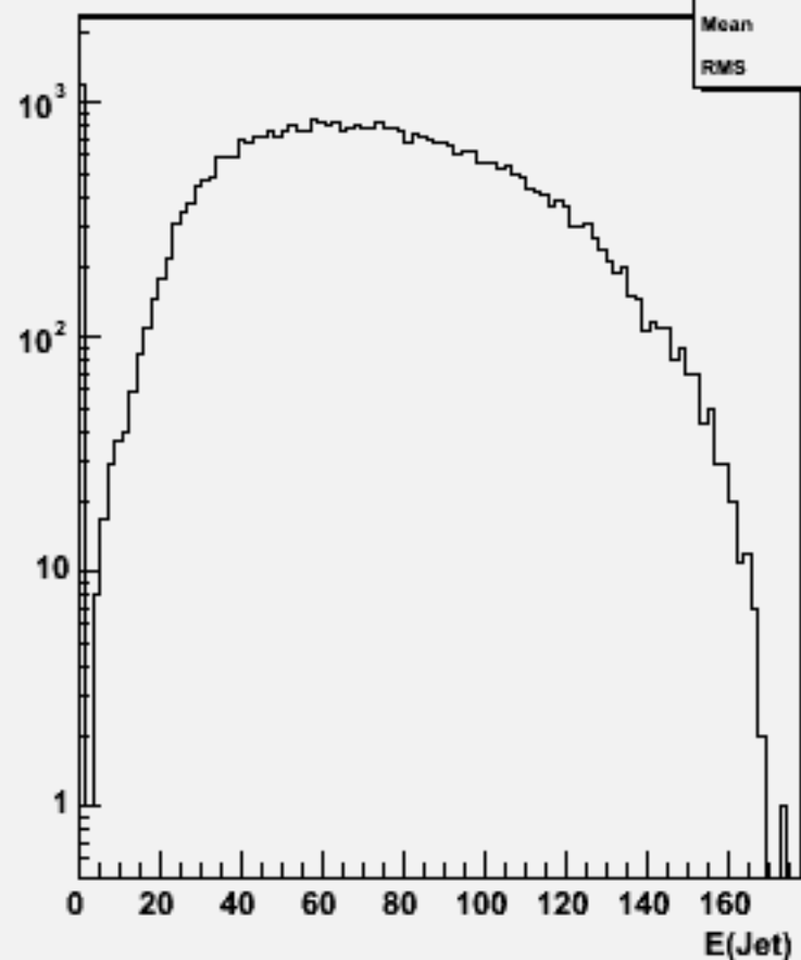
Jet energies(All jets)w103724 ae1_e1cse1n1_o
