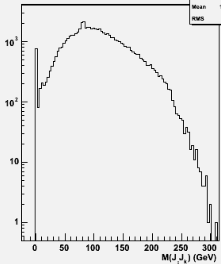
2jets mass(All comb)w103724 ae1_e1cse1n1_o
