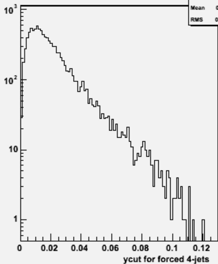
Ycut for 4-jets :w103722 ae1_e1udsc_o
