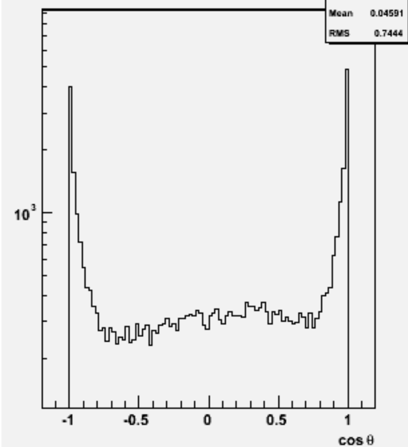
Jet cos \theta (All jets)w103722 ae1_e1udsc_o
