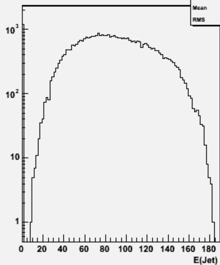
Jet energies(All jets)w103722 ae1_e1udsc_o
