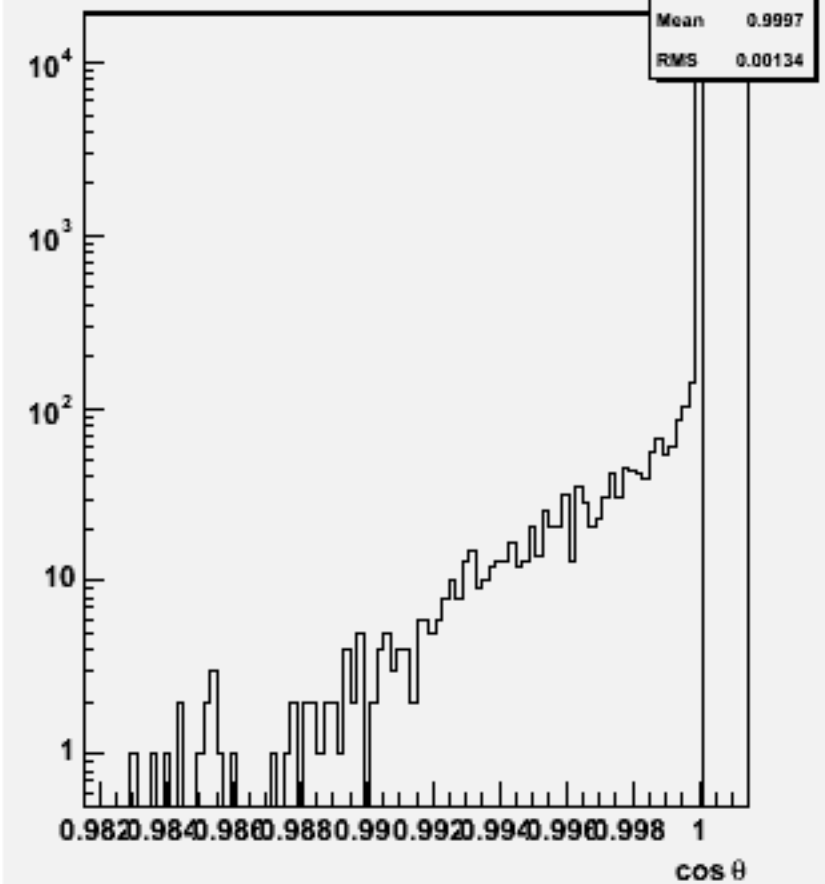
Jet cos \theta (All jets)w103721 ae1_e1udsc_o
