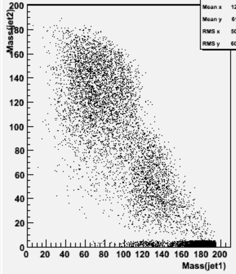
Jet mass for forced 2-jets : w103721 ae1_e1udsc_o
