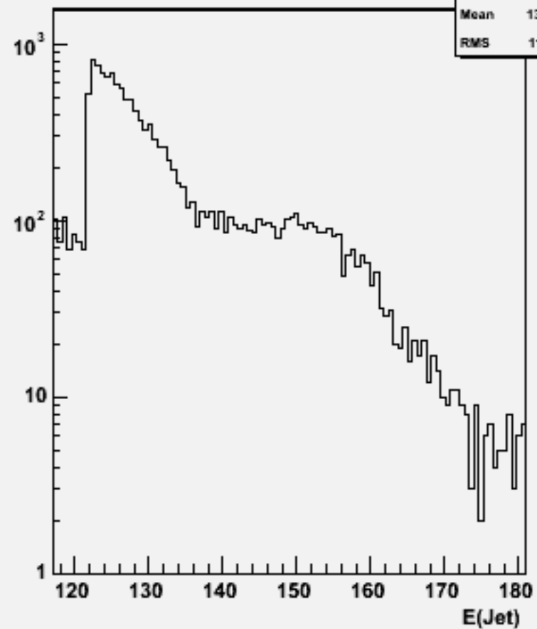
Jet energies(All jets)w103721 ae1_e1udsc_o
