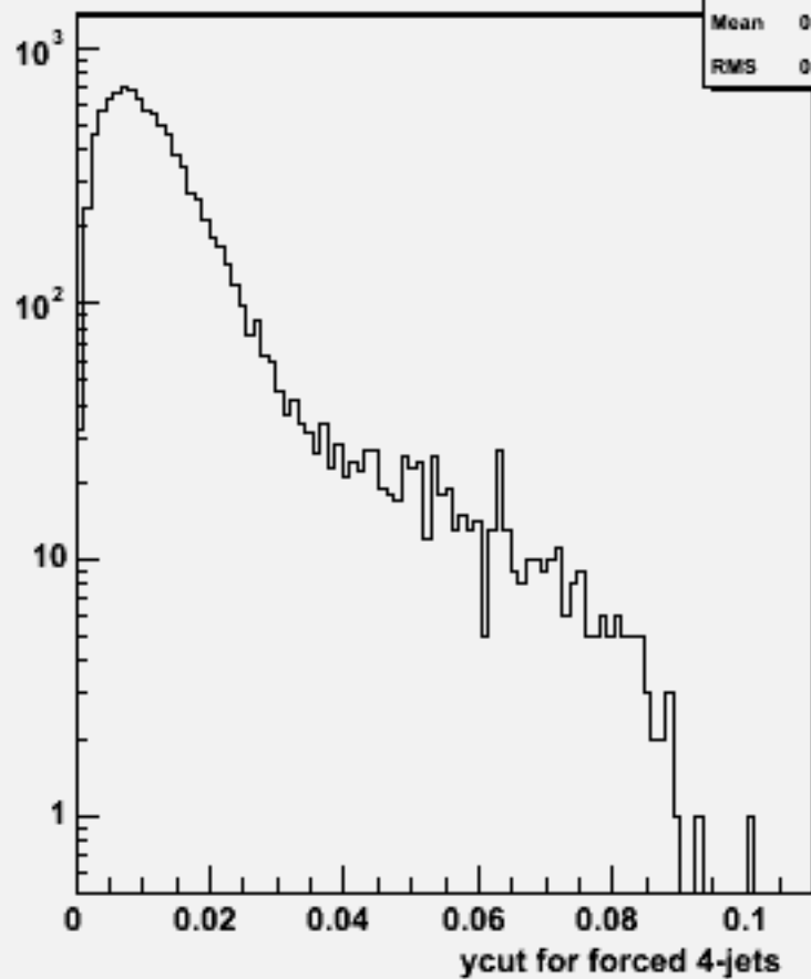
Ycut for 4-jets :w103721 ae1_e1udsc_o
