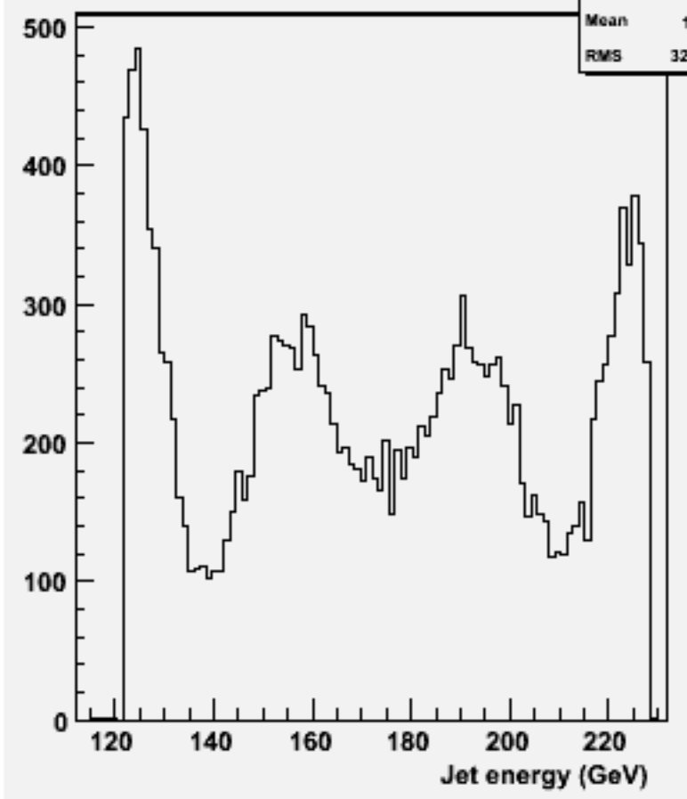
energy for 2-jets :w103721 ae1_e1udsc_o
