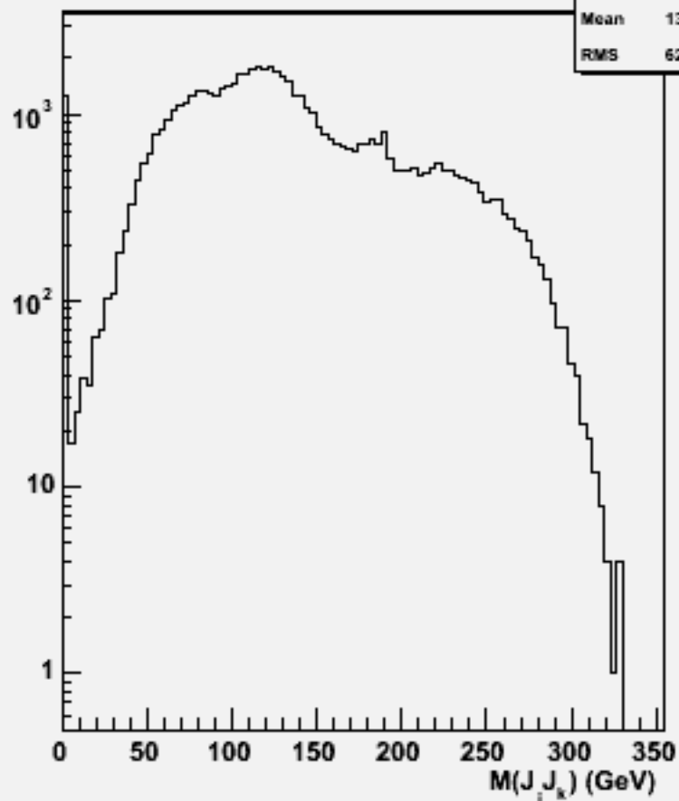
2jets mass(All comb)w103721 ae1_e1udsc_o
