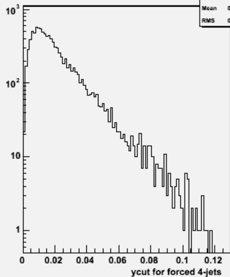
Ycut for 4-jets :w103720 ae1_e1udsc_o
