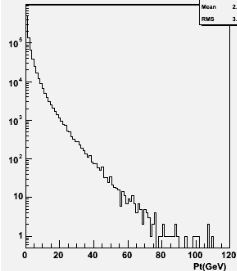
Particle Pt : w103720 ae1_e1udsc_o
