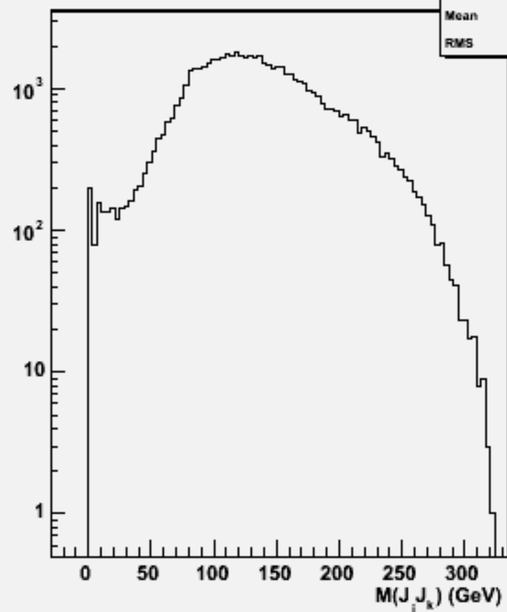
2jets mass(All comb)w103720 ae1_e1udsc_o
