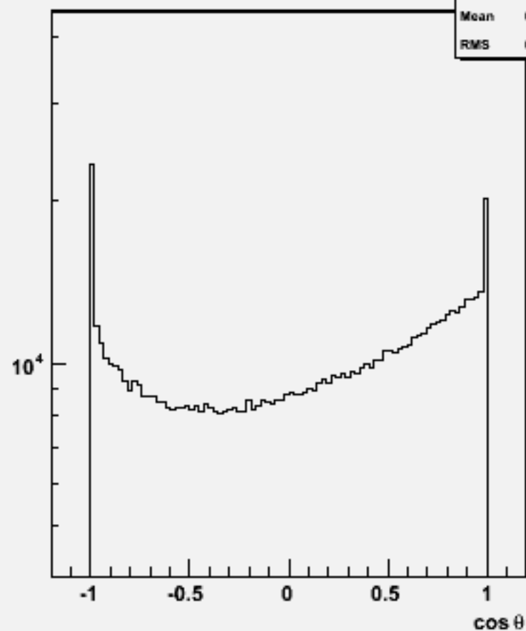
Particle \cos\theta : w103720 ae1_e1udsc_o
