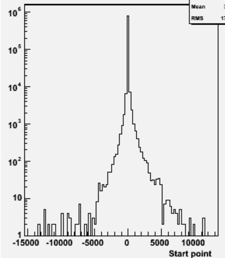
Start point Z : w103720 ae1_e1udsc_o
