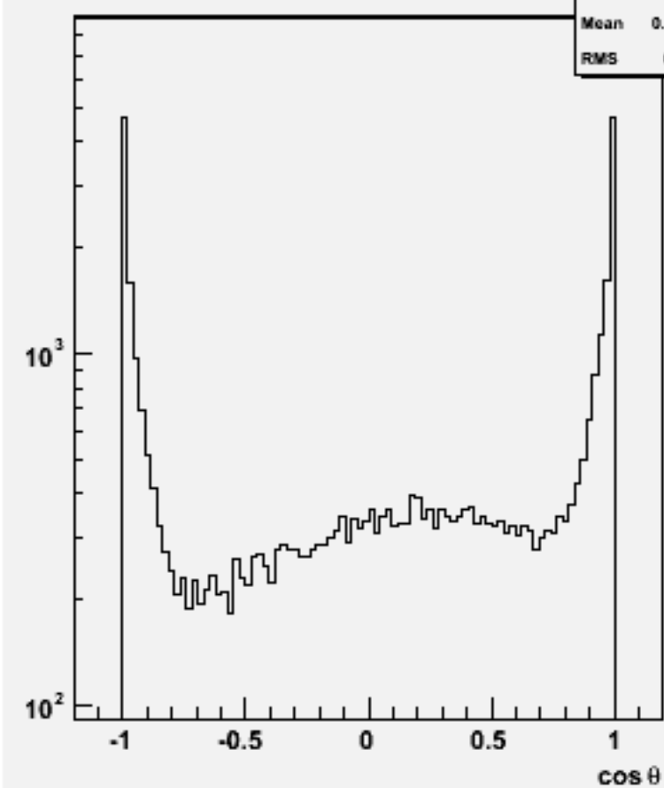
Jet cos \theta (All jets)w103720 ae1_e1udsc_o
