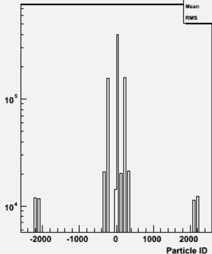
Particle ID : w103720 ae1_e1udsc_o
