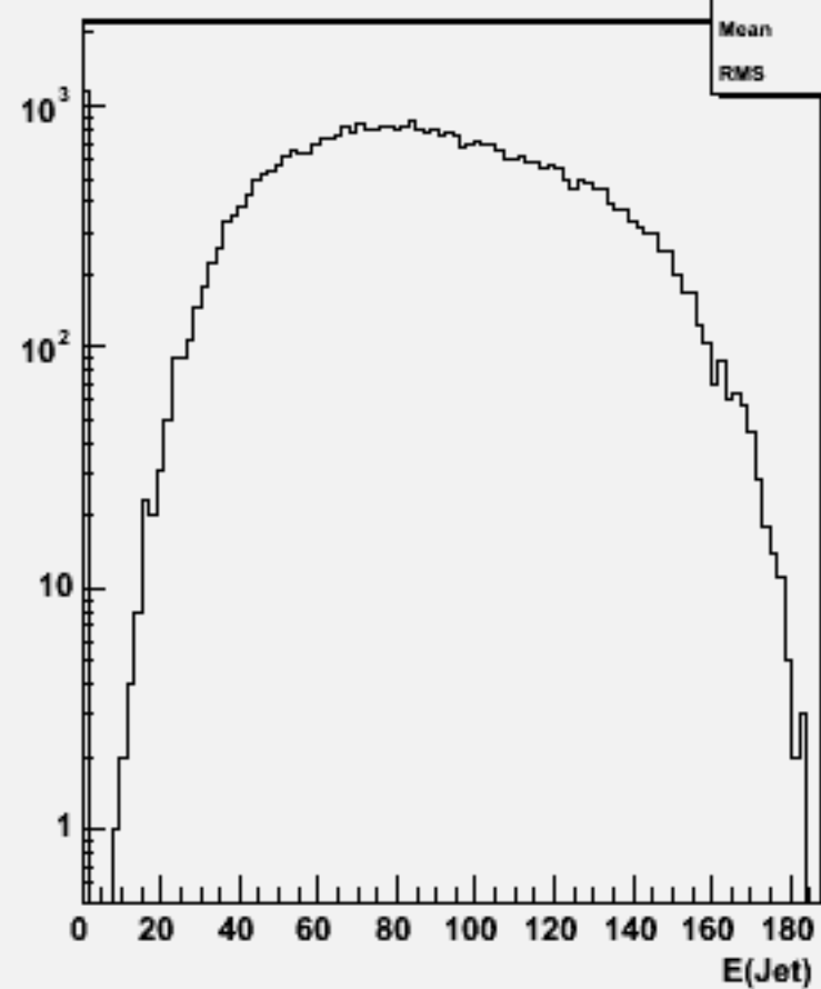
Jet energies(All jets)w103720 ae1_e1udsc_o
