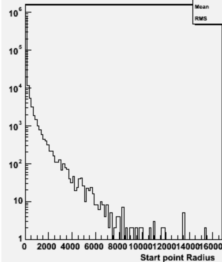
Start point R : w103720 ae1_e1udsc_o
