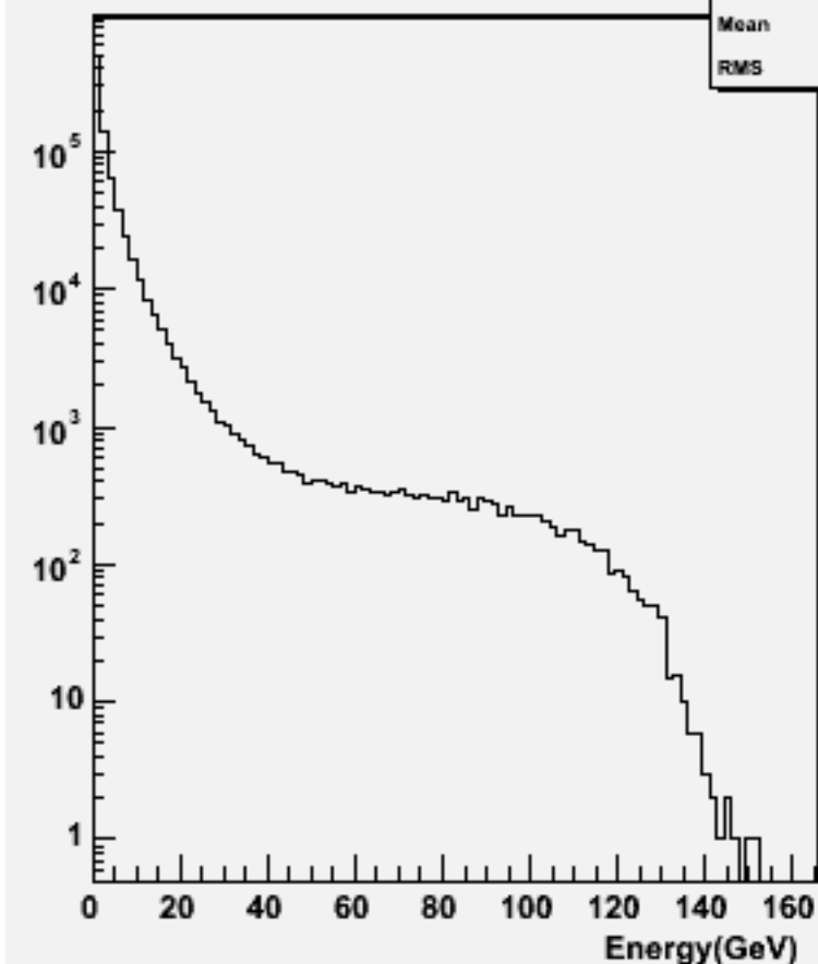
Particle Energy : w103720 ae1_e1udsc_o
