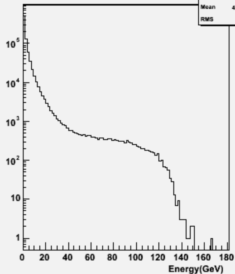
Particle Energy : w103718 ae1_e1uddu_o
