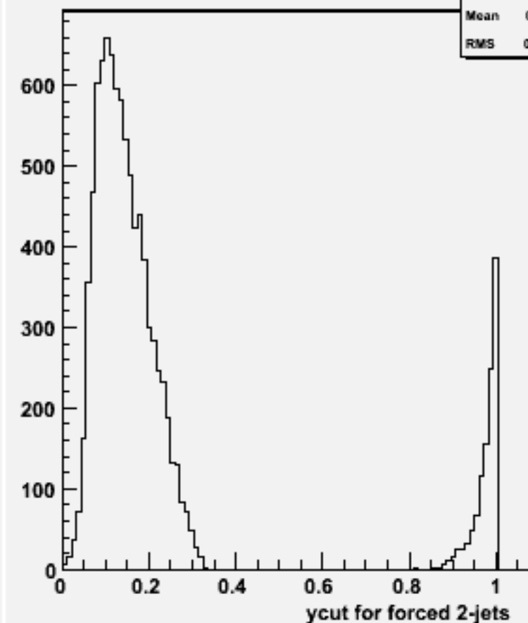
Ycut for 2-jets :w103718 ae1_e1uddu_o
