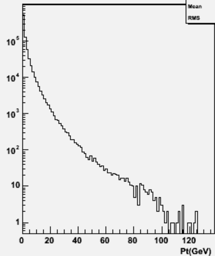
Particle Pt : w103718 ae1_e1uddu_o
