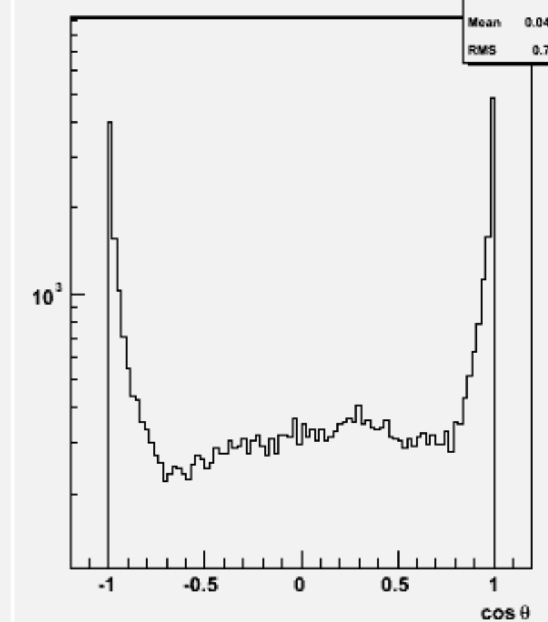
Jet cos \theta (All jets)w103718 ae1_e1uddu_o
