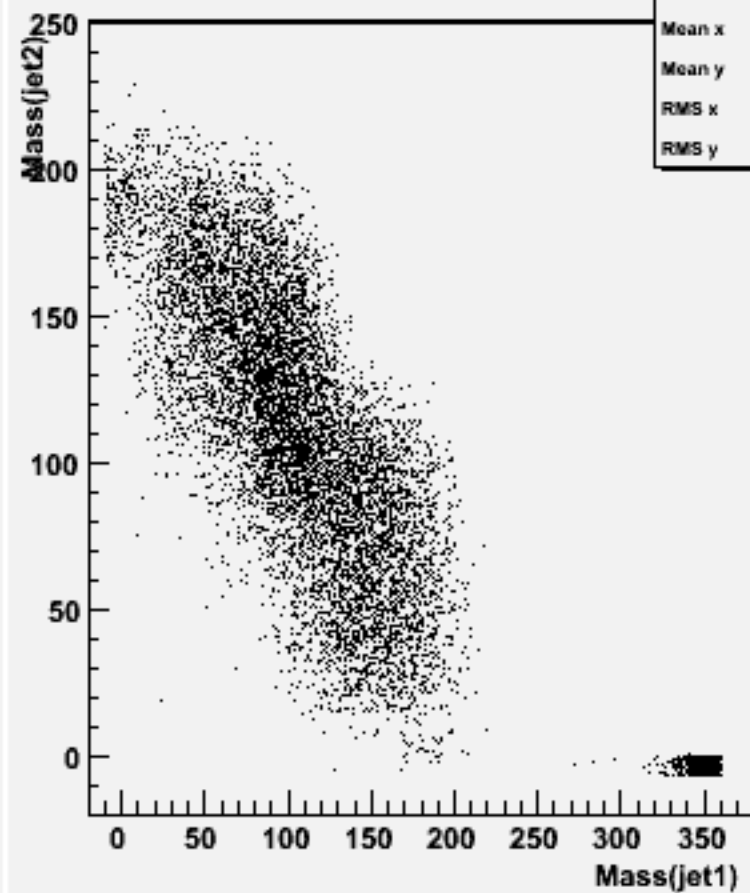
Jet mass for forced 2-jets : w103718 ae1_e1uddu_o
