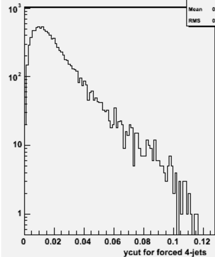
Ycut for 4-jets :w103718 ae1_e1uddu_o
