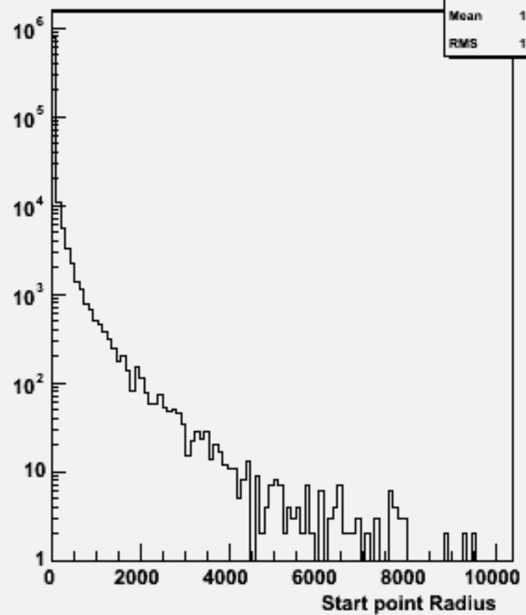
Start point R : w103718 ae1_e1uddu_o
