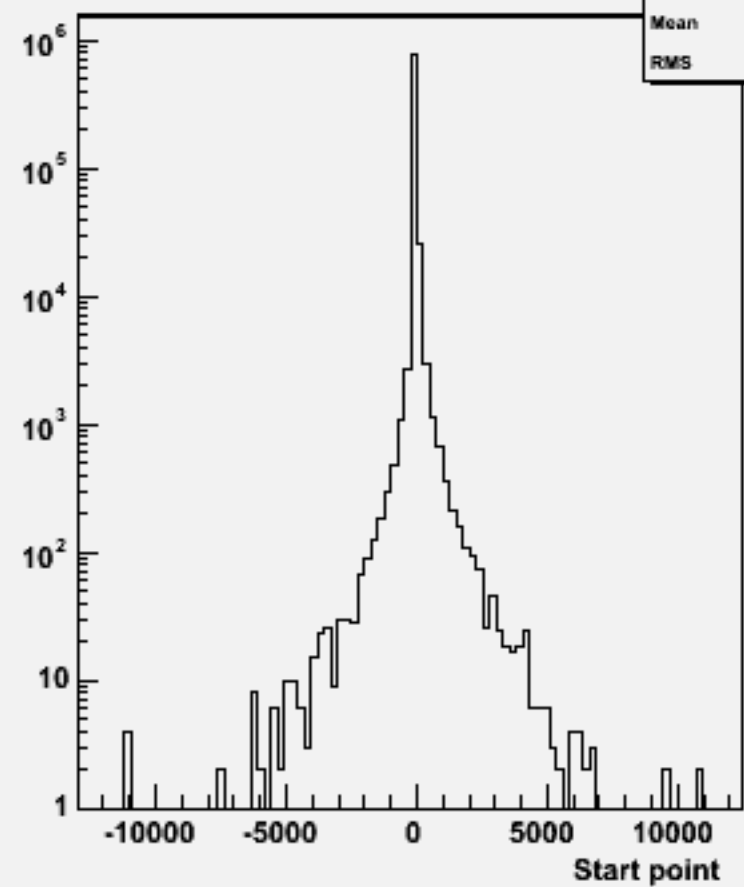
Start point Z : w103718 ae1_e1uddu_o
