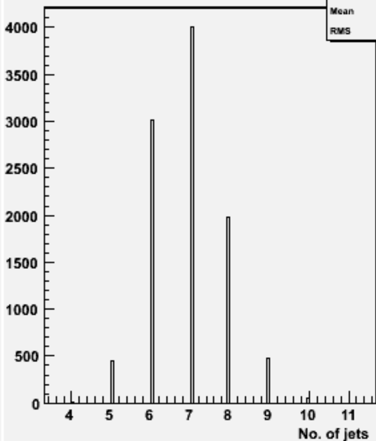
No. jets (ycut=0.001) : w103718 ae1_e1uddu_o
