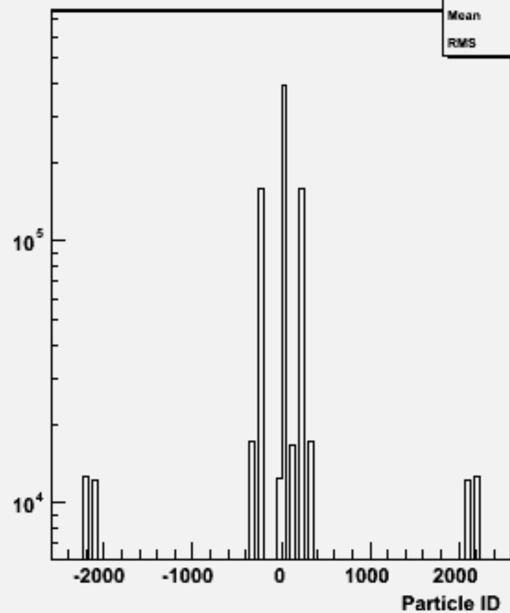
Particle ID : w103718 ae1_e1uddu_o
