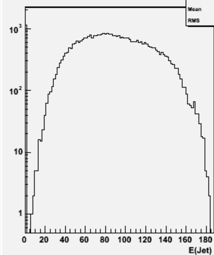
Jet energies(All jets)w103718 ae1_e1uddu_o
