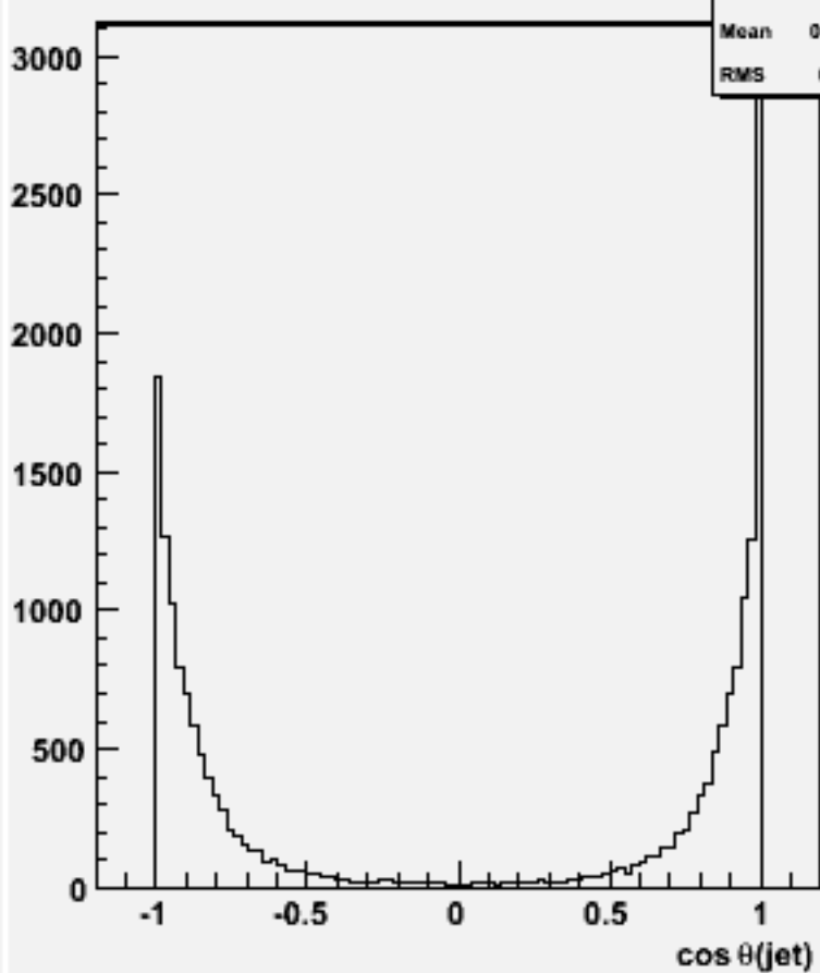
cos \theta for 2-jets :w103718 ae1_e1uddu_o
