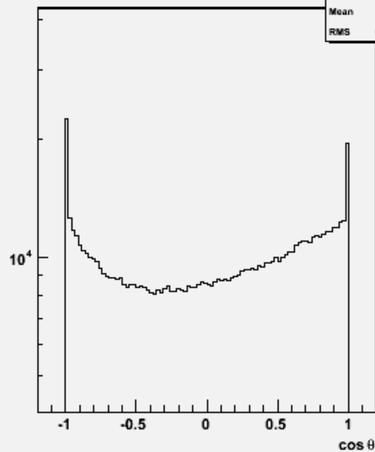
Particle cos \theta : w103718 ae1_e1uddu_o
