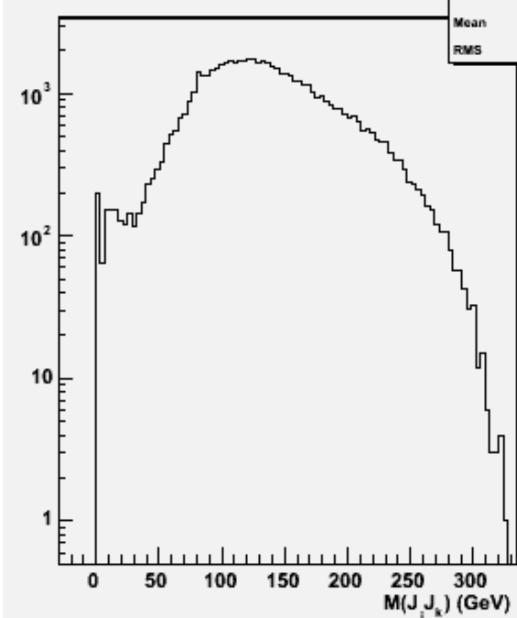
2jets mass(All comb)w103718 ae1_e1uddu_o
