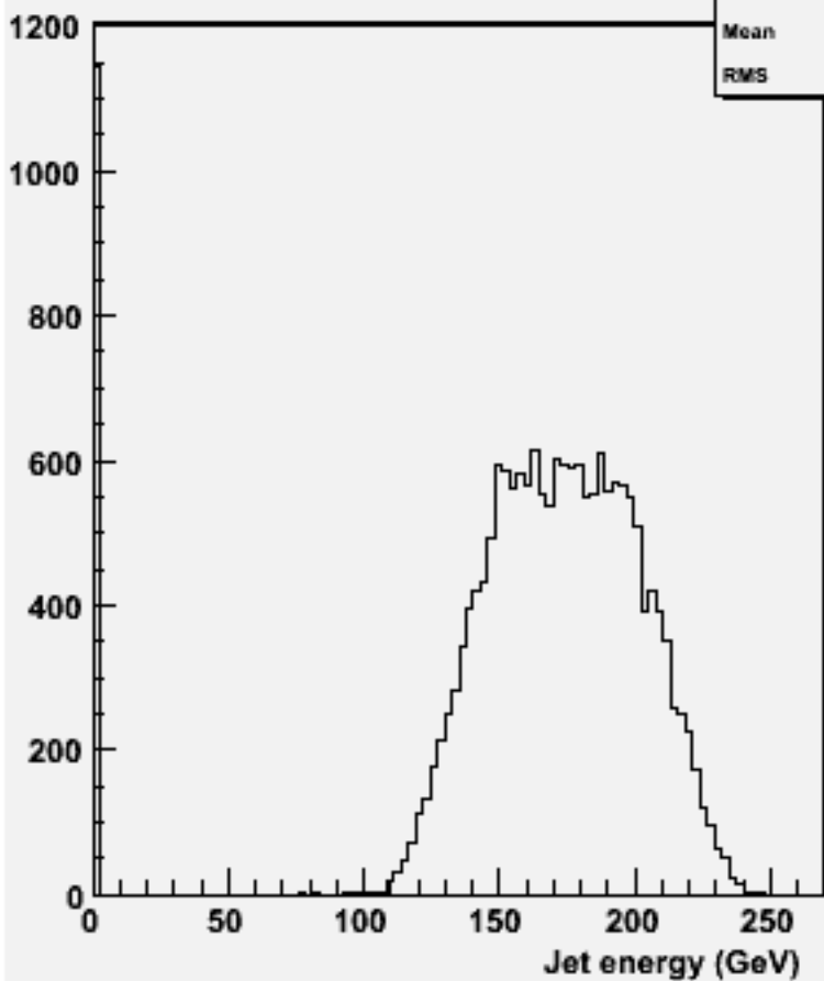
energy for 2-jets :w103718 ae1_e1uddu_o
