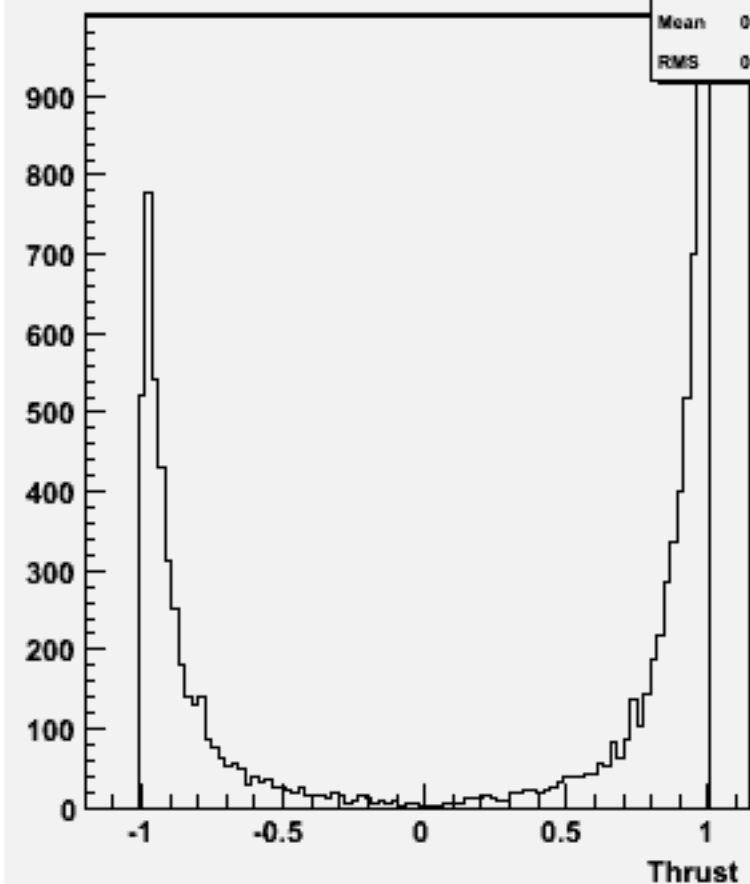
cos \Theta (thrust) w103718 ae1_e1uddu_o
