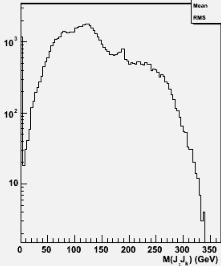
2jets mass(All comb)w103717 ae1_e1uddu_o
