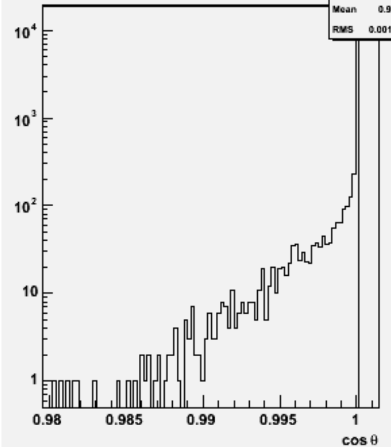
Jet cos \theta (All jets)w103717 ae1_e1uddu_o
