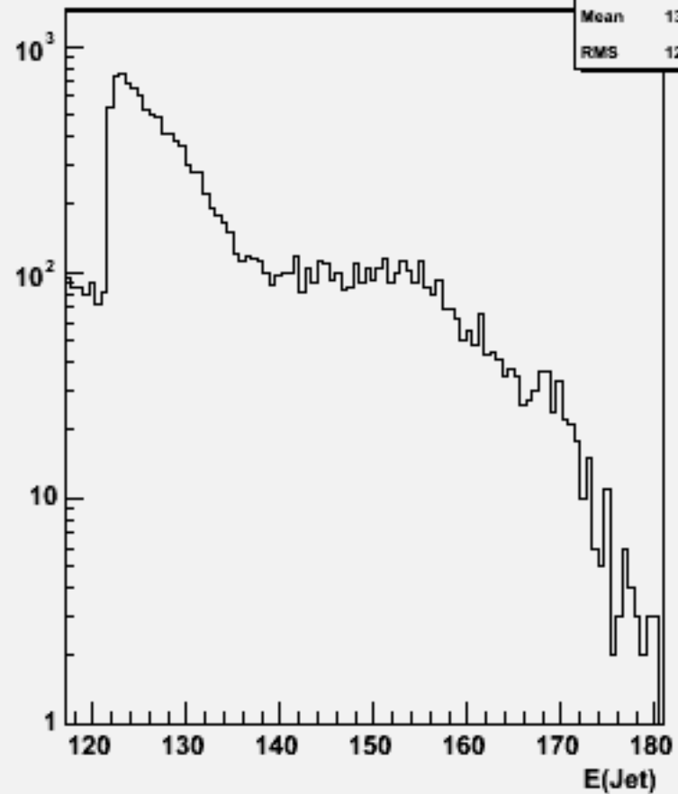
Jet energies(All jets)w103717 ae1_e1uddu_o
