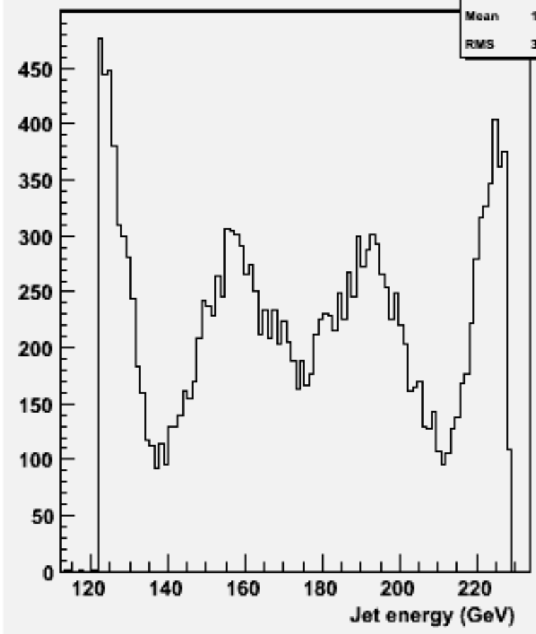
energy for 2-jets :w103717 ae1_e1uddu_o
