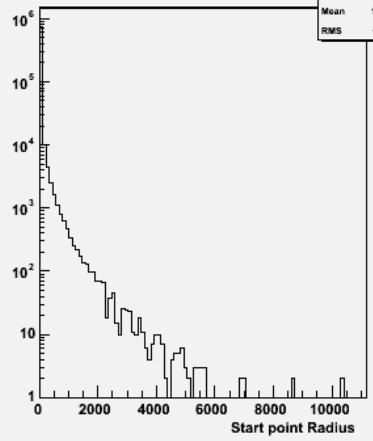
Start point R : w103717 ae1_e1uddu_o
