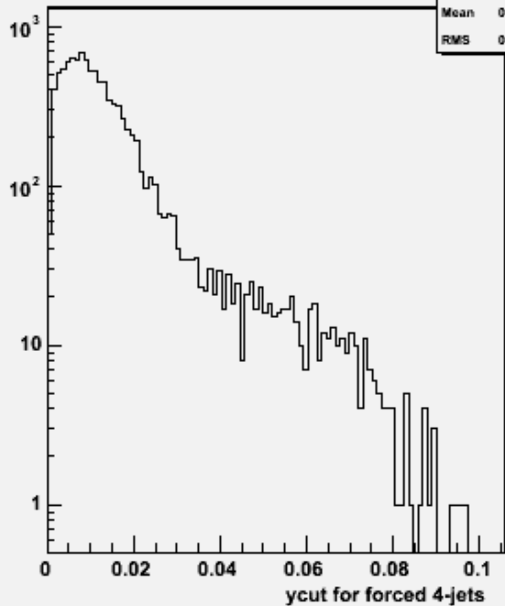
Ycut for 4-jets :w103717 ae1_e1uddu_o
