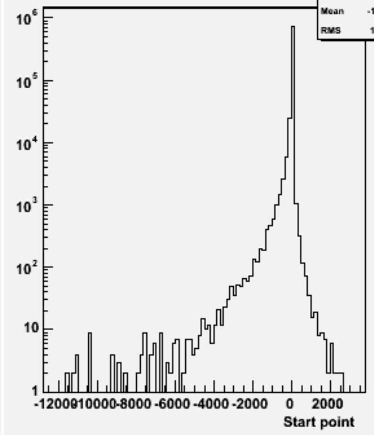
Start point Z : w103717 ae1_e1uddu_o
