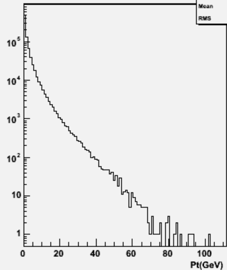
Particle Pt : w103716 ae1_e1uddu_o
