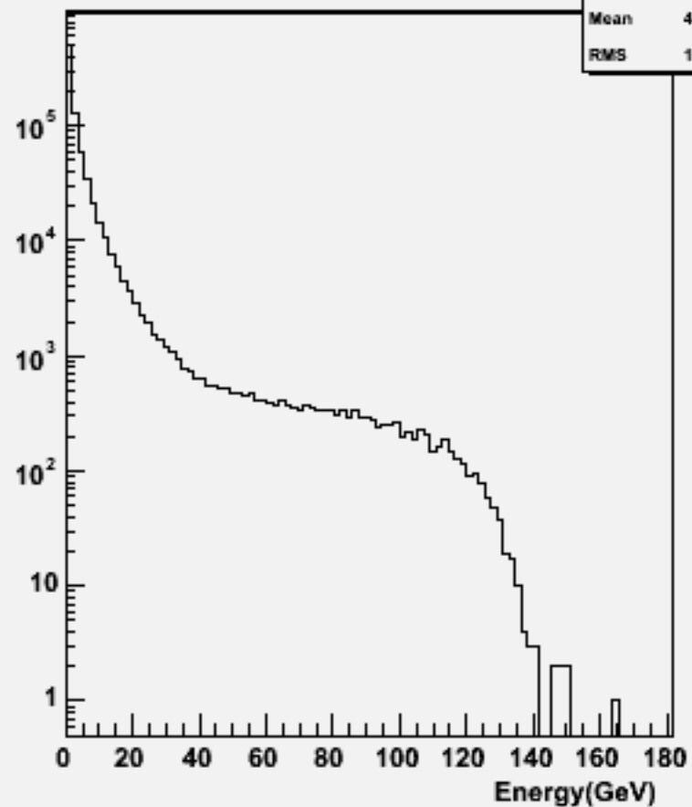
Particle Energy : w103716 ae1_e1uddu_o
