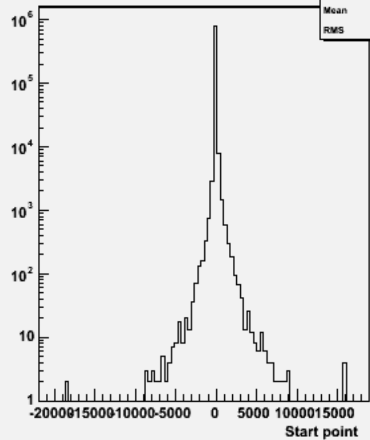
Start point Z : w103716 ae1_e1uddu_o
