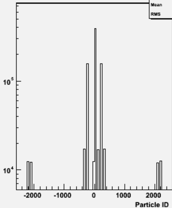
Particle ID : w103716 ae1_e1uddu_o
