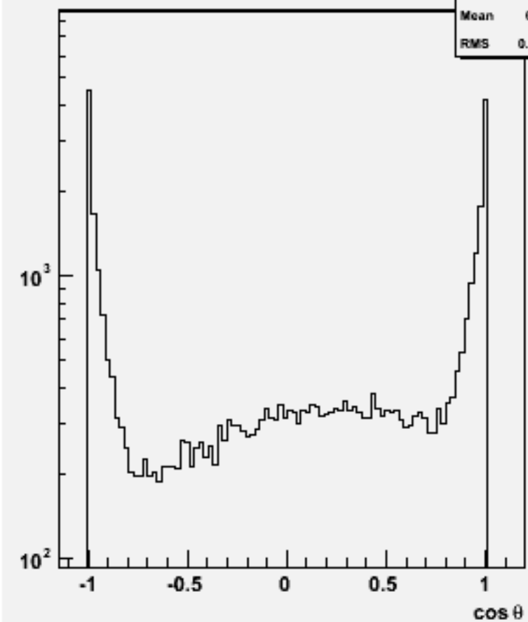
Jet cos \theta (All jets)w103716 ae1_e1uddu_o
