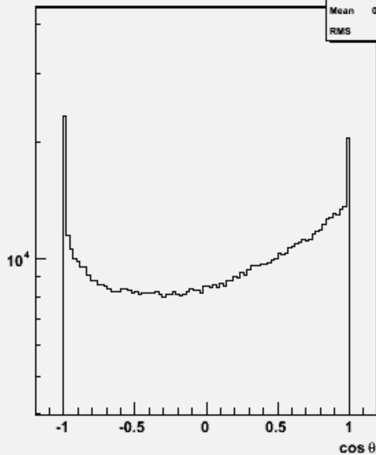
Particle \cos\theta : w103716 ae1_e1uddu_o
