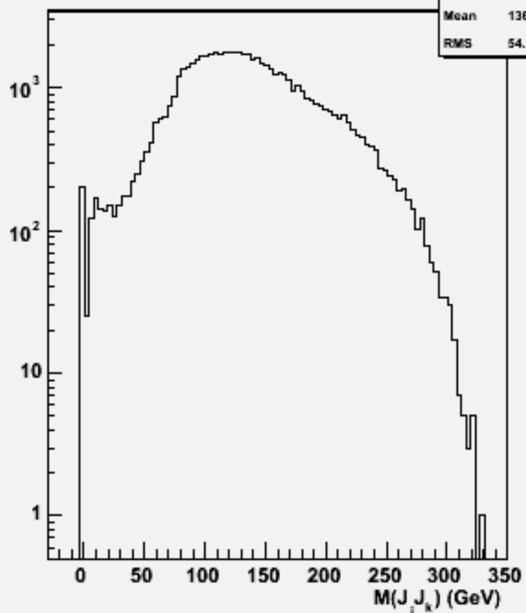
2jets mass(All comb)w103716 ae1_e1uddu_o
