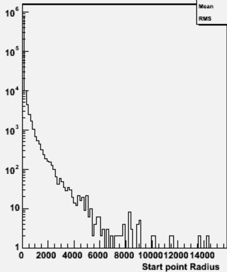
Start point R : w103716 ae1_e1uddu_o
