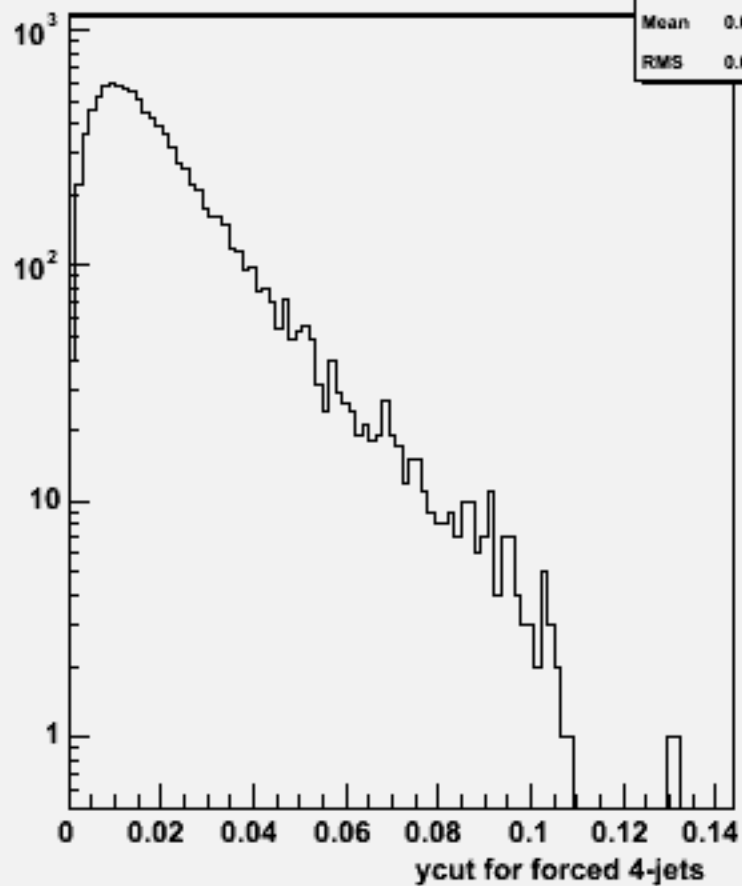
Ycut for 4-jets :w103716 ae1_e1uddu_o
