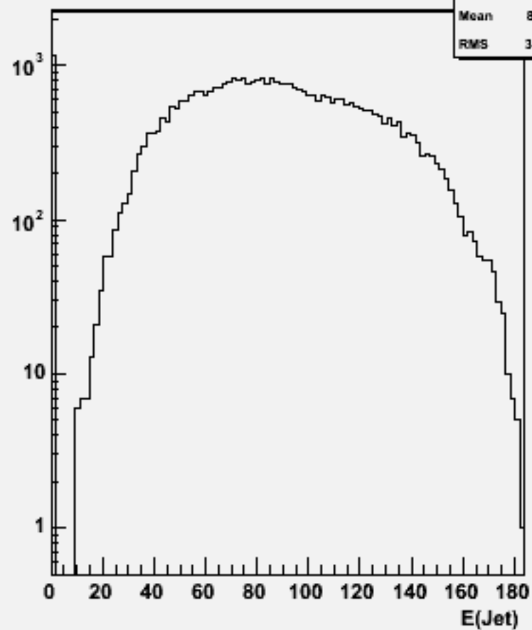
Jet energies(All jets)w103716 ae1_e1uddu_o
