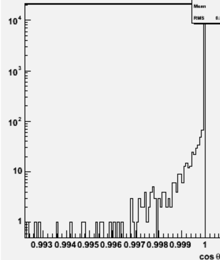
Jet cos \theta (All jets)w103713 ae1_e1ude3n3_o
