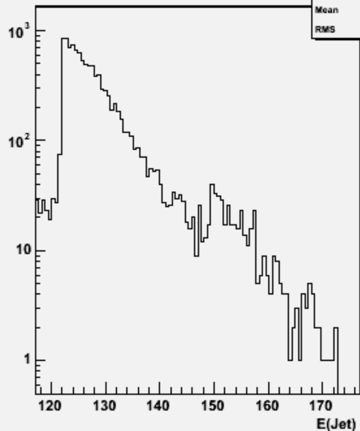
Jet energies(All jets)w103713 ae1_e1ude3n3_o
