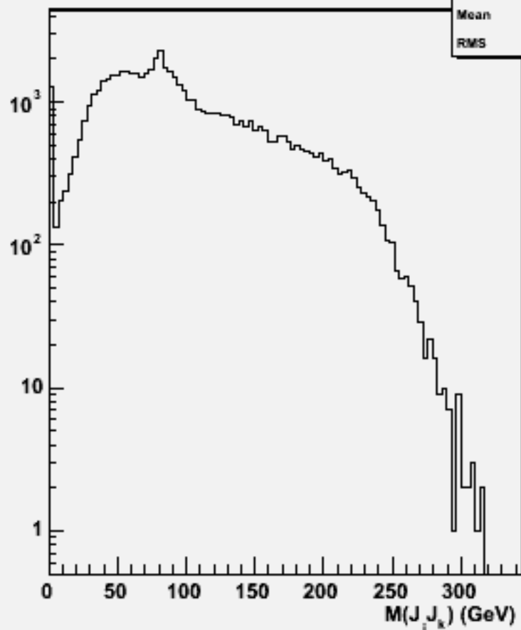
2jets mass(All comb)w103713 ae1_e1ude3n3_o
