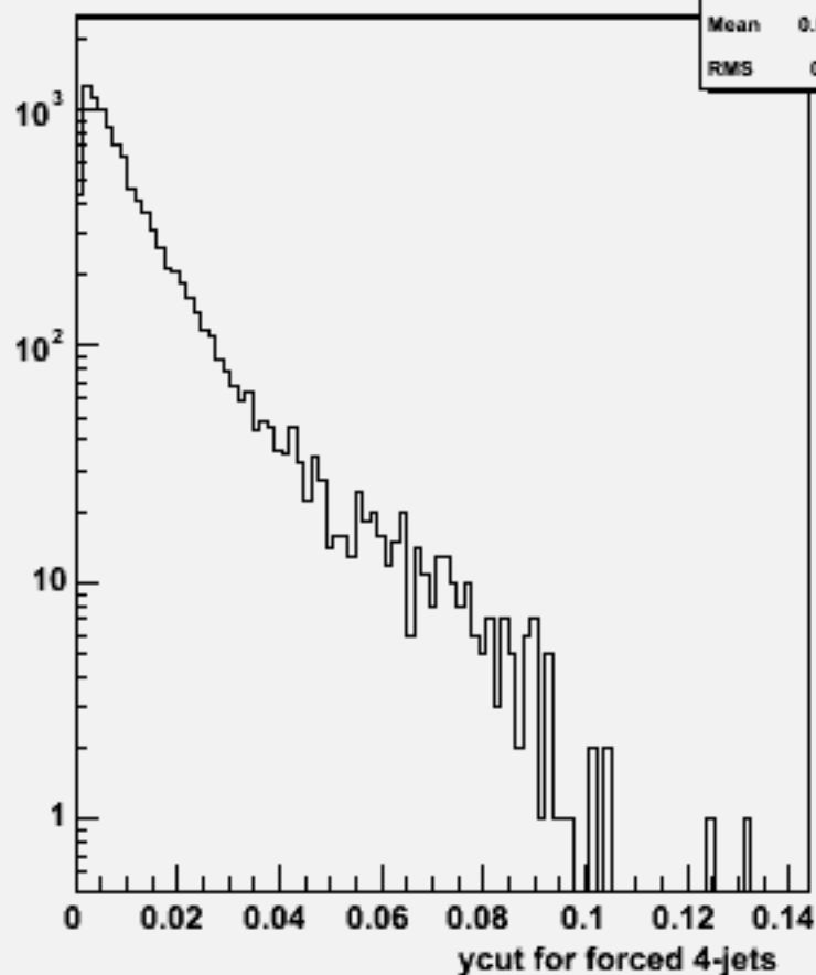
Ycut for 4-jets :w103712 ae1_e1ude3n3_o
