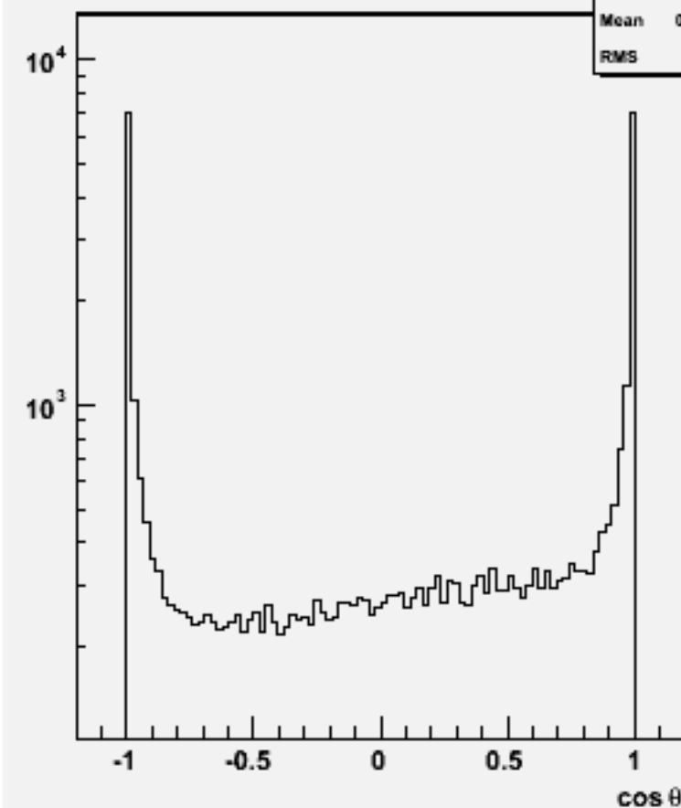
Jet cos \theta (All jets)w103712 ae1_e1ude3n3_o
