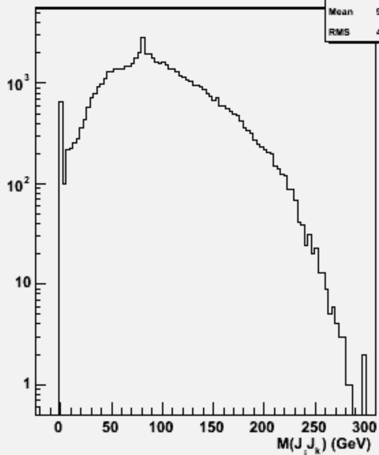
2jets mass(All comb)w103712 ae1_e1ude3n3_o
