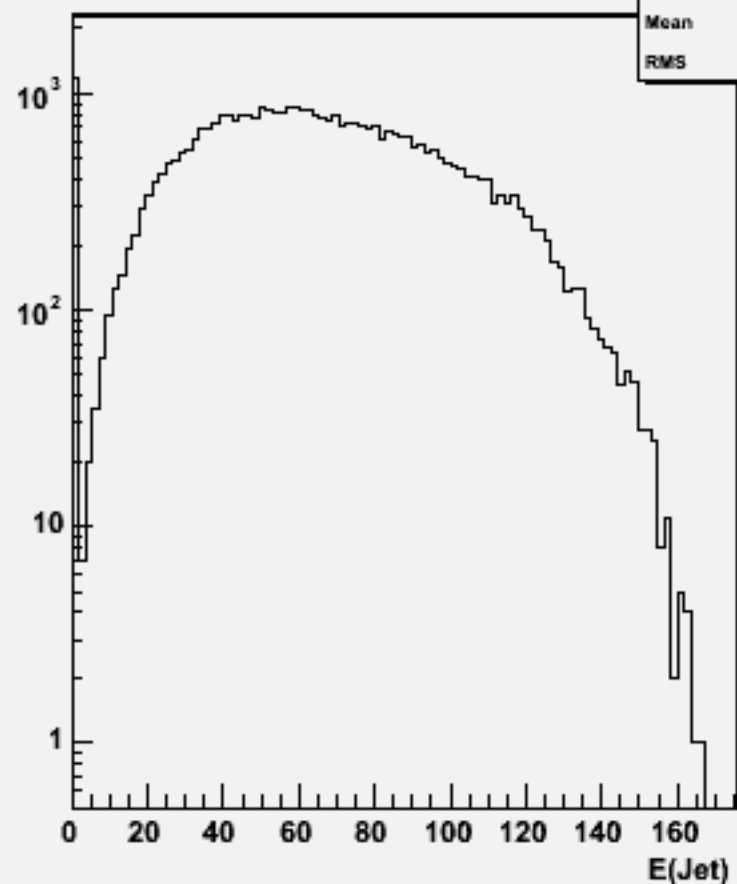
Jet energies(All jets)w103712 ae1_e1ude3n3_o
