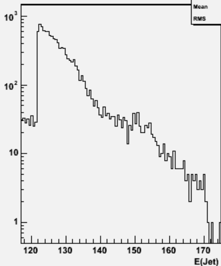
Jet energies(All jets)w103711 ae1_e1ude2n2_o
