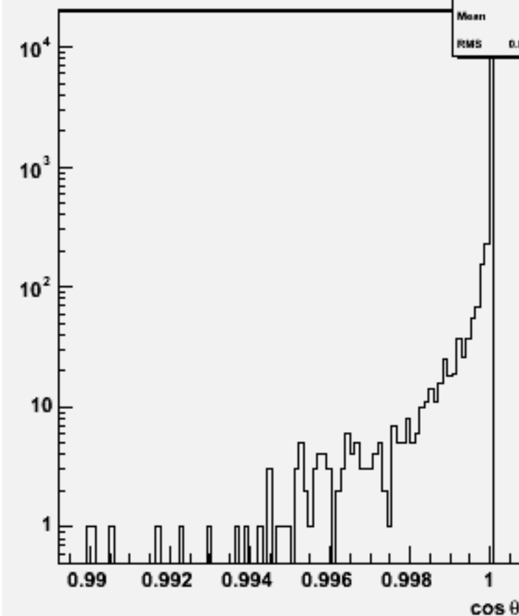
Jet cos \theta (All jets)w103711 ae1_e1ude2n2_o
