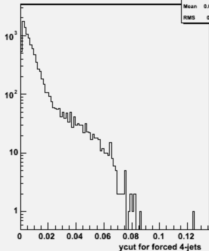
Ycut for 4-jets :w103711 ae1_e1ude2n2_o
