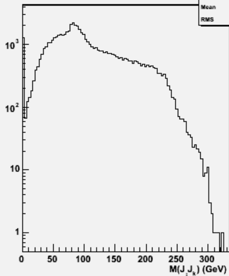
2jets mass(All comb)w103711 ae1_e1ude2n2_o
