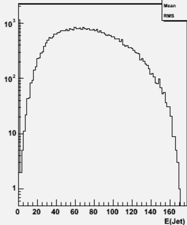
Jet energies(All jets)w103710 ae1_e1ude2n2_o
