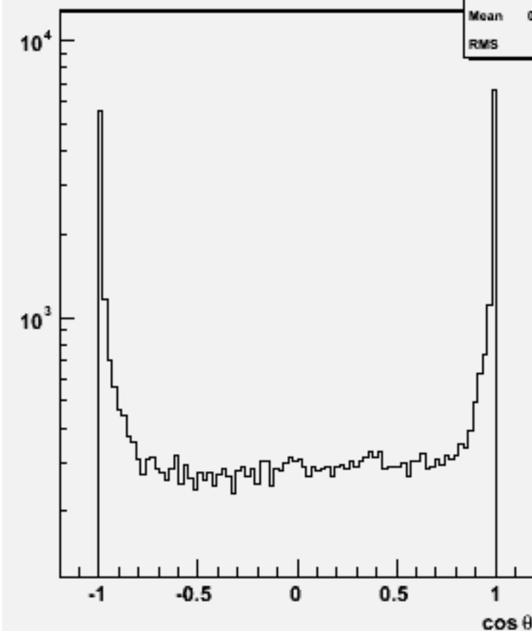
Jet cos \theta (All jets)w103710 ae1_e1ude2n2_o
