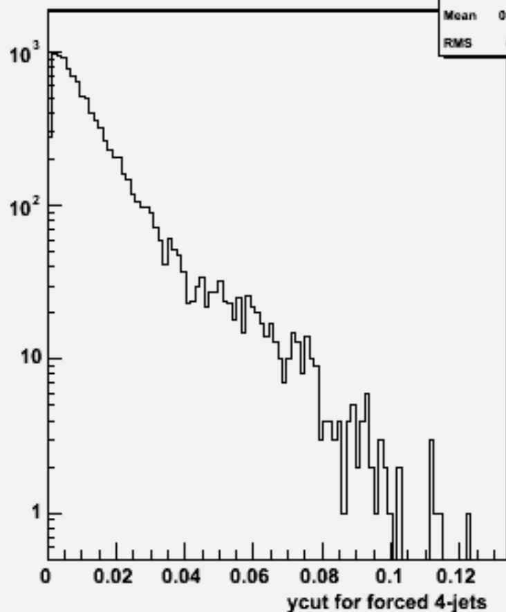
Ycut for 4-jets :w103710 ae1_e1ude2n2_o
