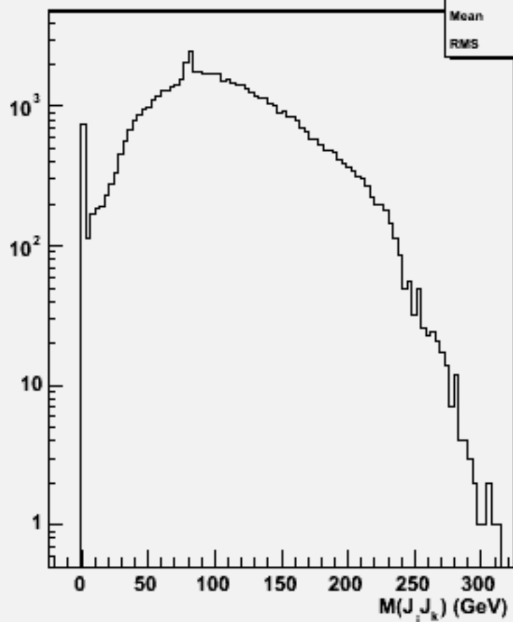
2jets mass(All comb)w103710 ae1_e1ude2n2_o
