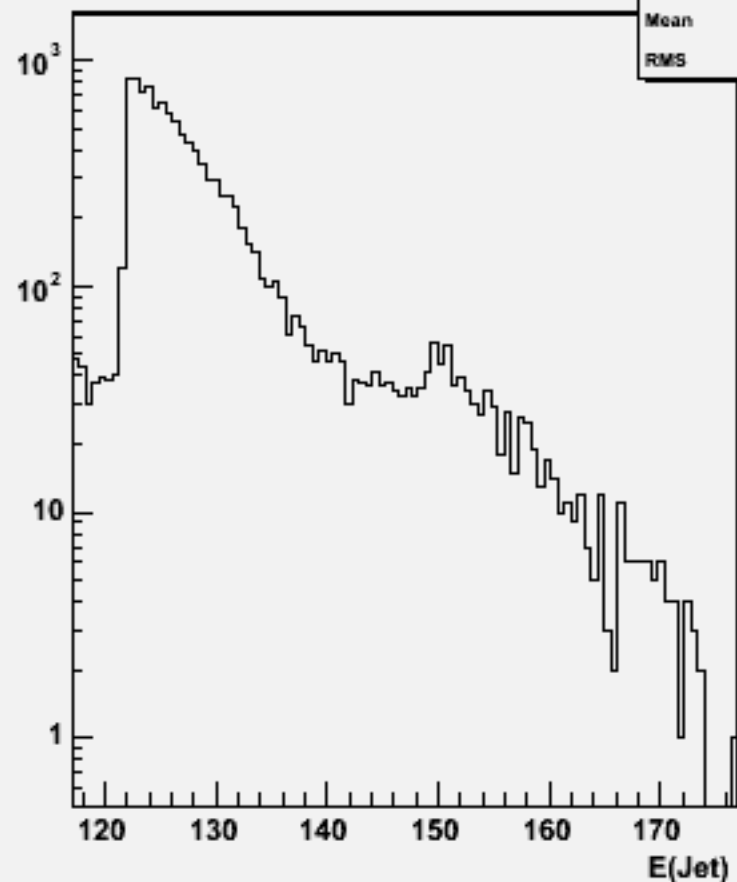
Jet energies(All jets)w103709 ae1_e1ude2n2_o
