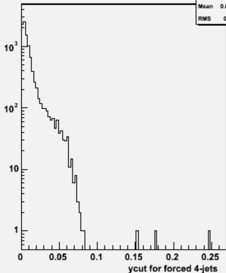
Ycut for 4-jets :w103709 ae1_e1ude2n2_o
