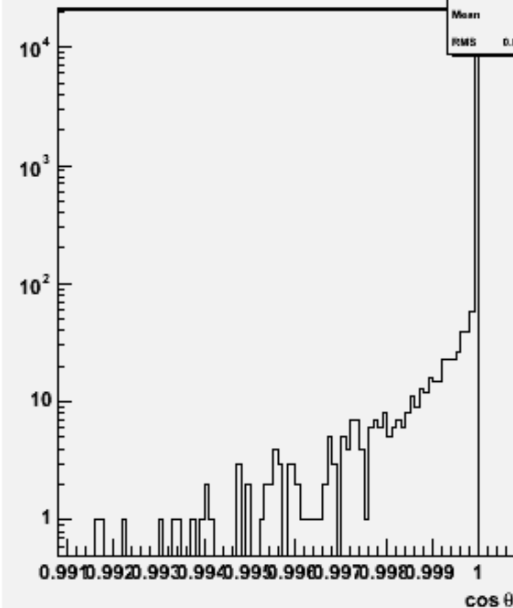
Jet cos \theta (All jets)w103709 ae1_e1ude2n2_o
