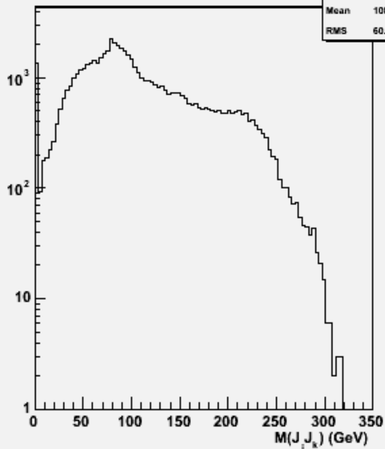
2jets mass(All comb)w103709 ae1_e1ude2n2_o
