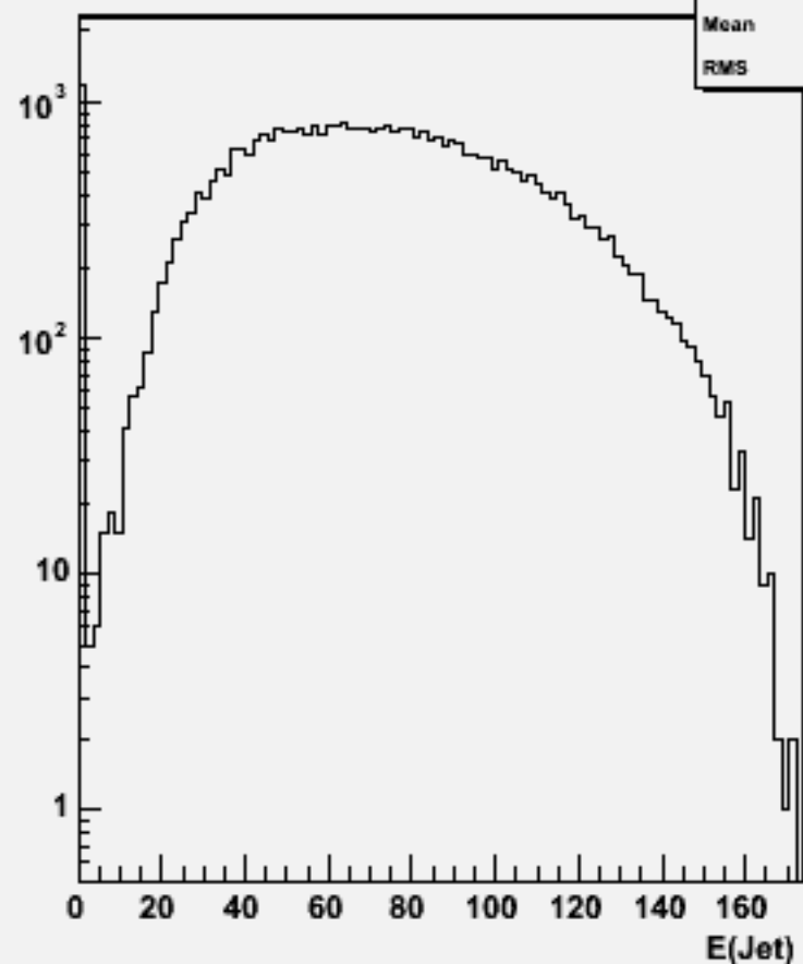
Jet energies(All jets)w103708 ae1_e1ude2n2_o
