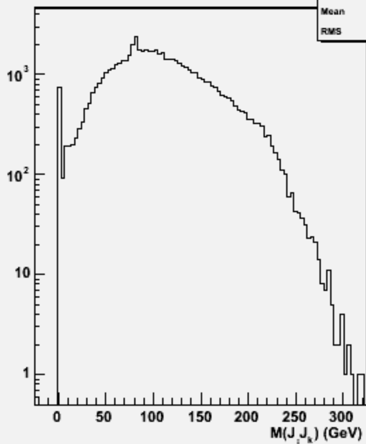
2jets mass(All comb)w103708 ae1_e1ude2n2_o
