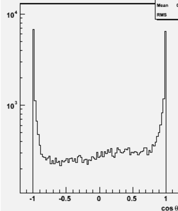
Jet cos \theta (All jets)w103708 ae1_e1ude2n2_o
