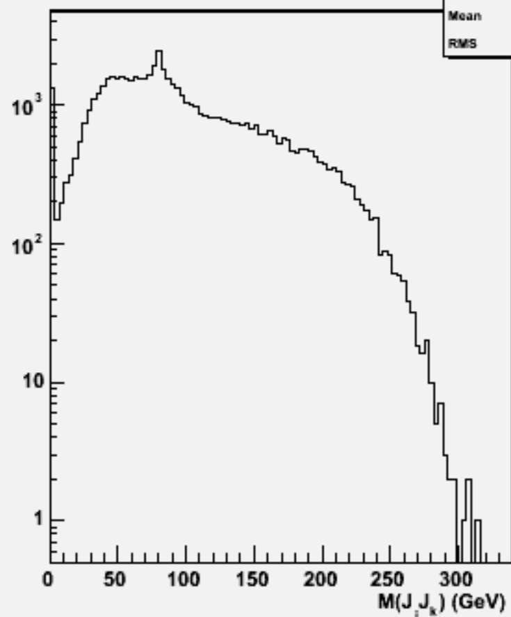
2jets mass(All comb)w103703 ae1_e1n3e3sc_o
