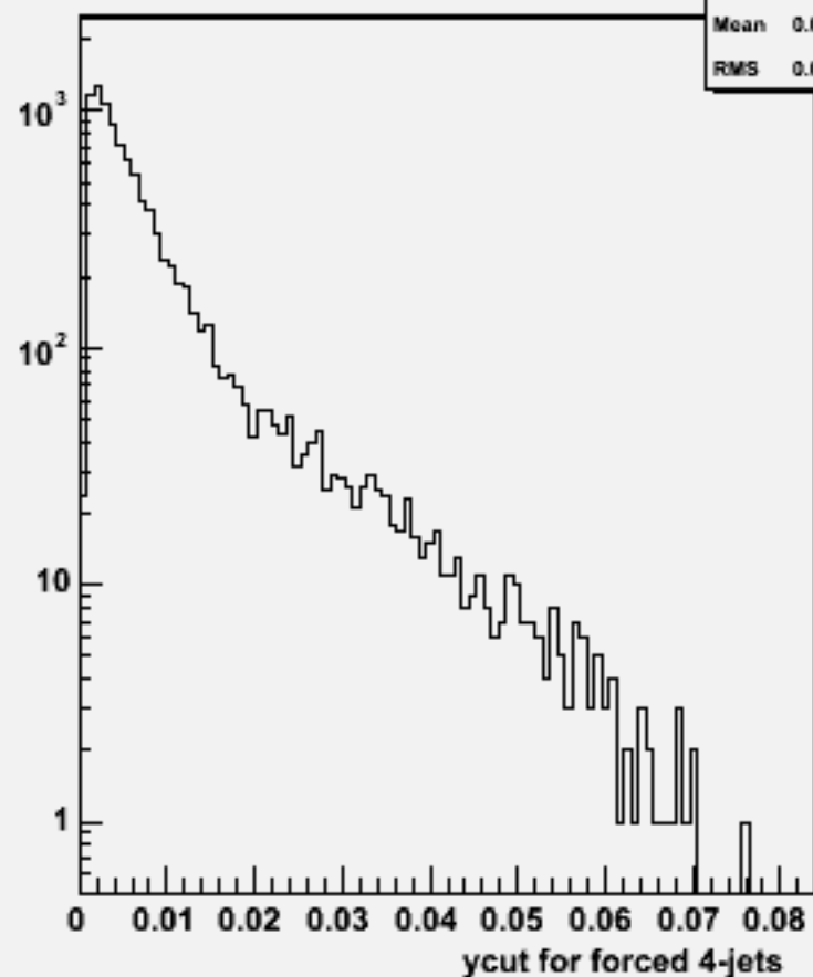
Ycut for 4-jets :w103703 ae1_e1n3e3sc_o
