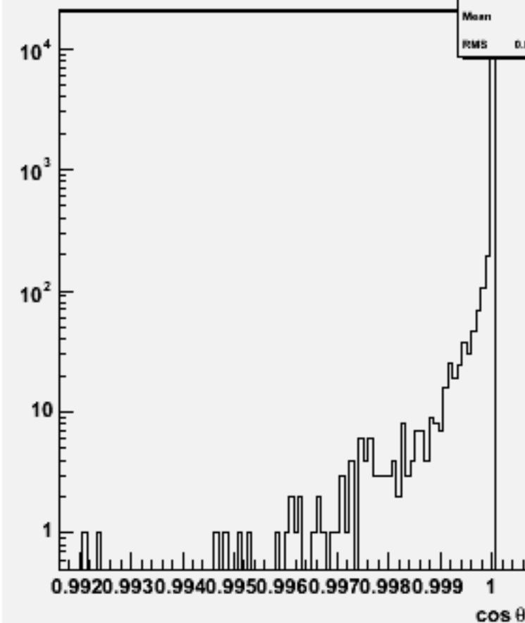
Jet cos \theta (All jets)w103703 ae1_e1n3e3sc_o
