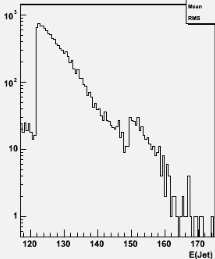
Jet energies(All jets)w103703 ae1_e1n3e3sc_o
