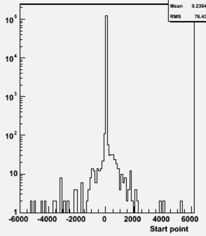
Start point Z : w103692 ae1_e1n3e3e3n3_o
