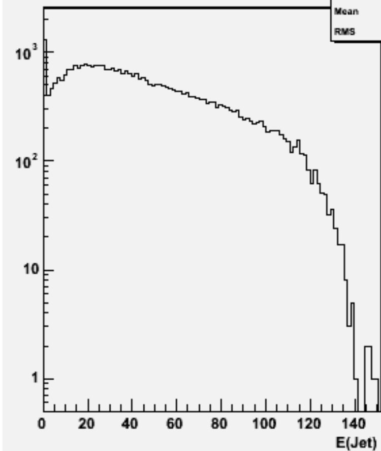
Jet energies(All jets)w103692 ae1_e1n3e3e3n3_o
