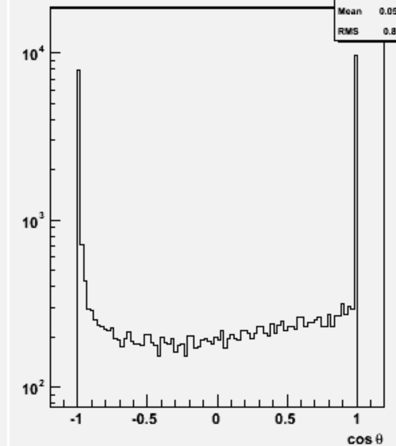
Jet cos \theta (All jets)w103692 ae1_e1n3e3e3n3_o
