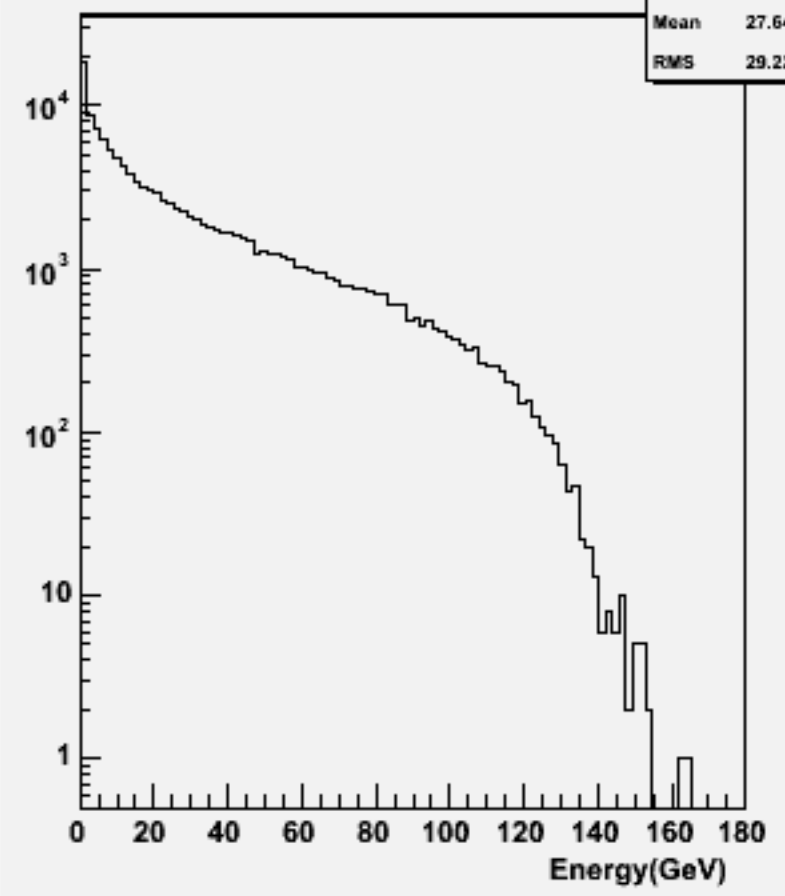
Start point R : w103692 ae1_e1n3e3e3n3_o
