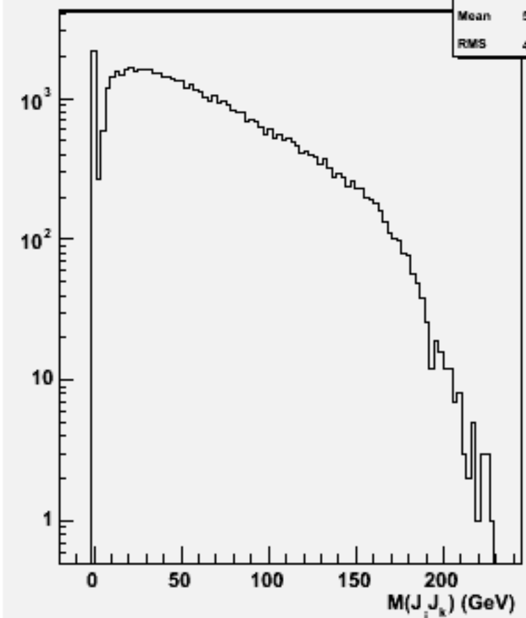
2jets mass(All comb)w103692 ae1_e1n3e3e3n3_o
