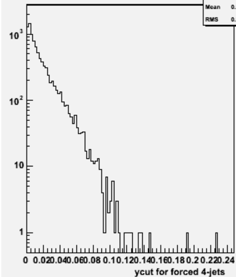
Ycut for 4-jets :w103692 ae1_e1n3e3e3n3_o
