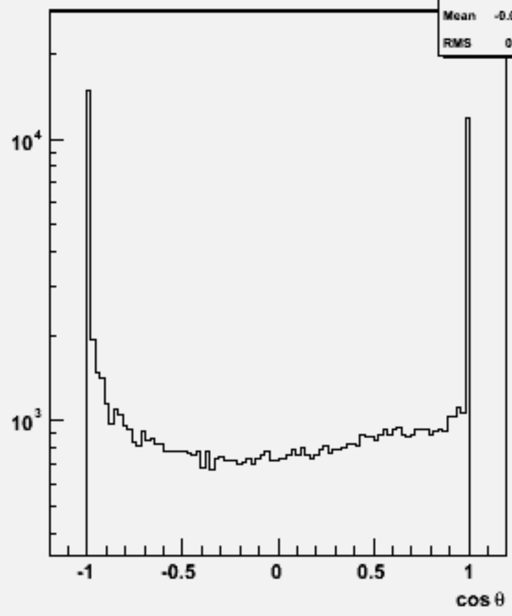
Particle cos \theta : w103686 ae1_e1n3e3e1n1_o
