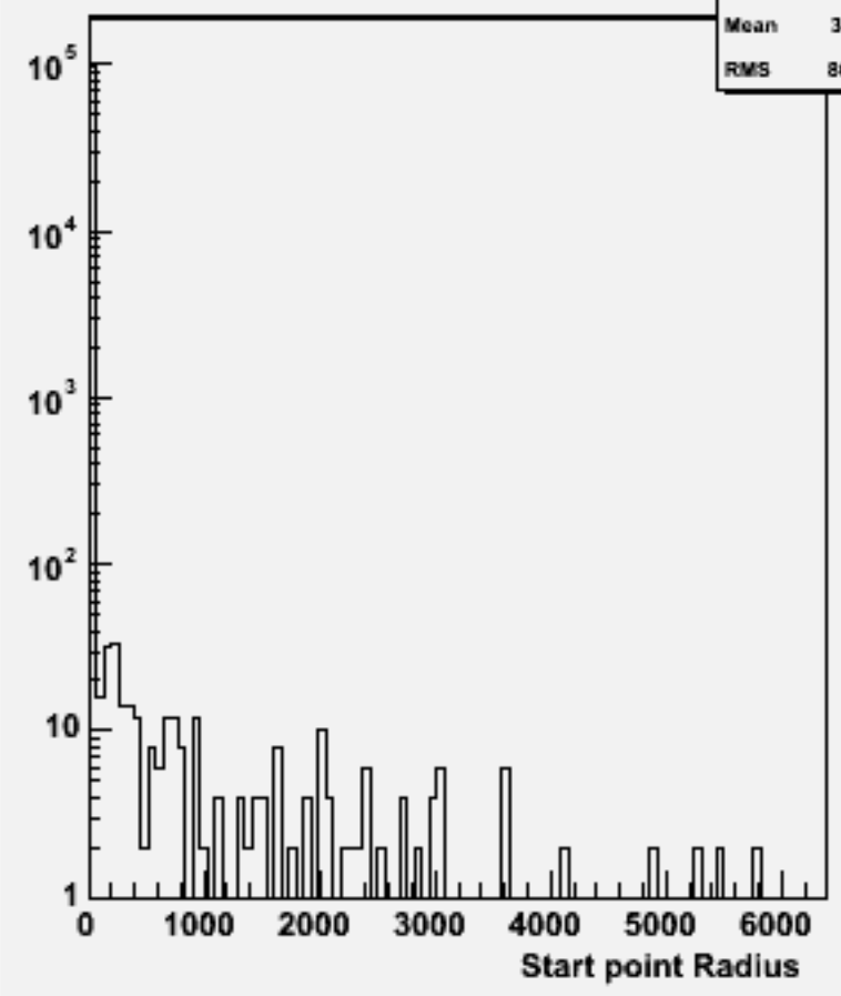
Start point R : w103686 ae1_e1n3e3e1n1_o
