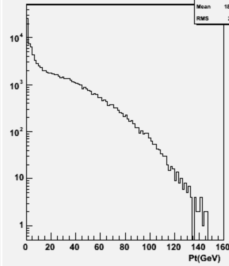
Start point Z : w103686 ae1_e1n3e3e1n1_o
