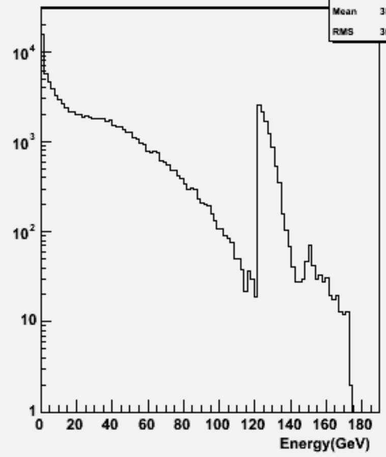
Start point R : w103685 ae1_e1n3e3e1n1_o
