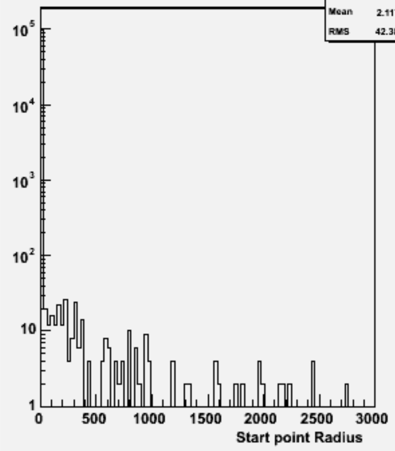
Start point R : w103685 ae1_e1n3e3e1n1_o
