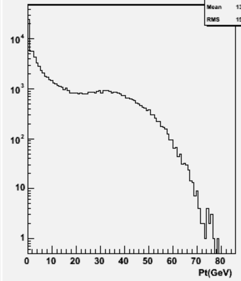
Start point Z : w103685 ae1_e1n3e3e1n1_o
