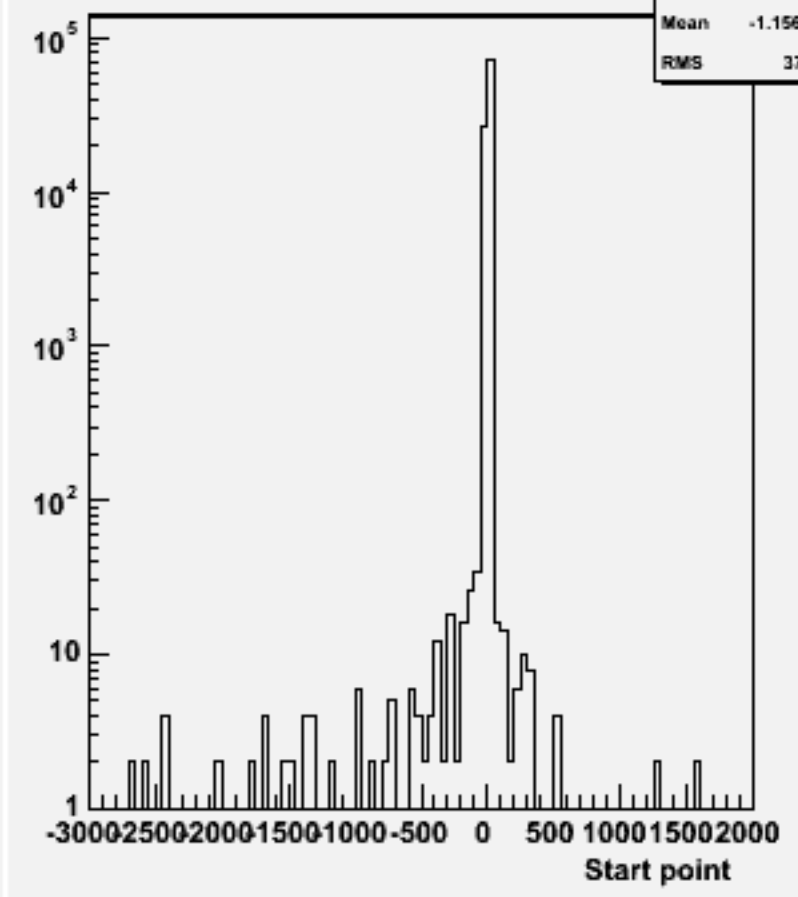
Start point Z : w103685 ae1_e1n3e3e1n1_o
