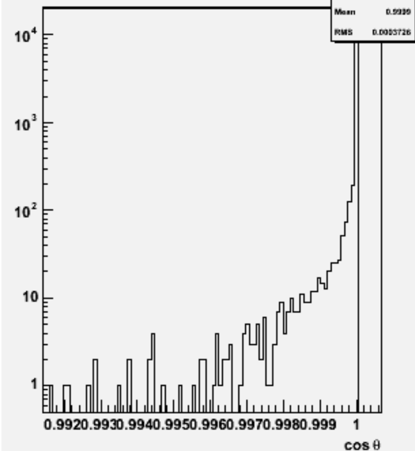
Jet cos theta (All jets)w103683 ae1_e1n2e2sc_o
