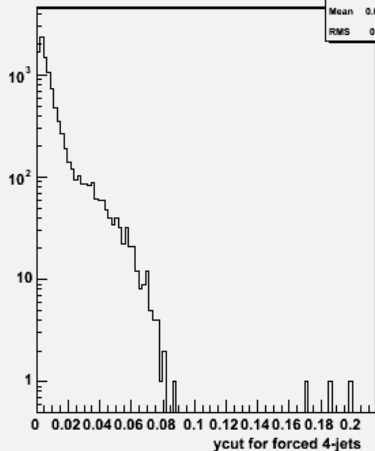
Ycut for 4-jets :w103683 ae1_e1n2e2sc_o
