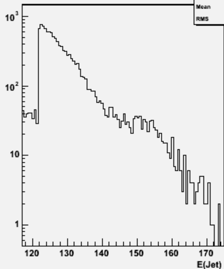
Jet energies(All jets)w103683 ae1_e1n2e2sc_o
