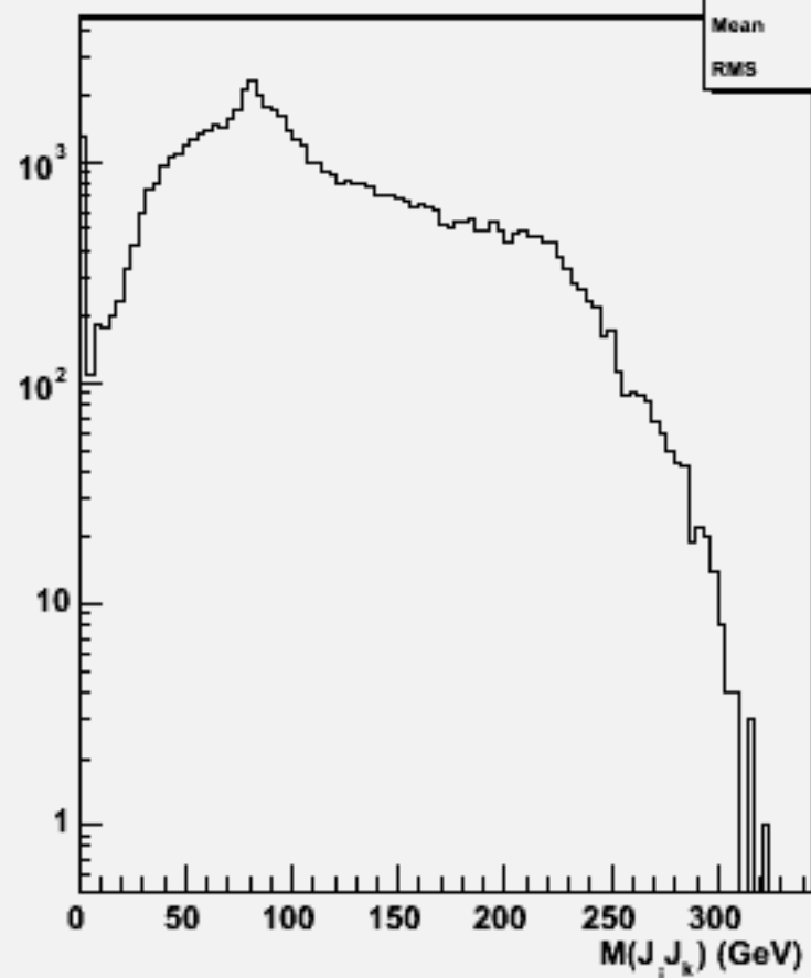
2jets mass(All comb)w103683 ae1_e1n2e2sc_o
