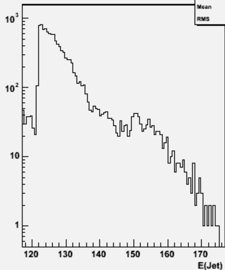
Jet energies(All jets)w103681 ae1_e1n2e2sc_o
