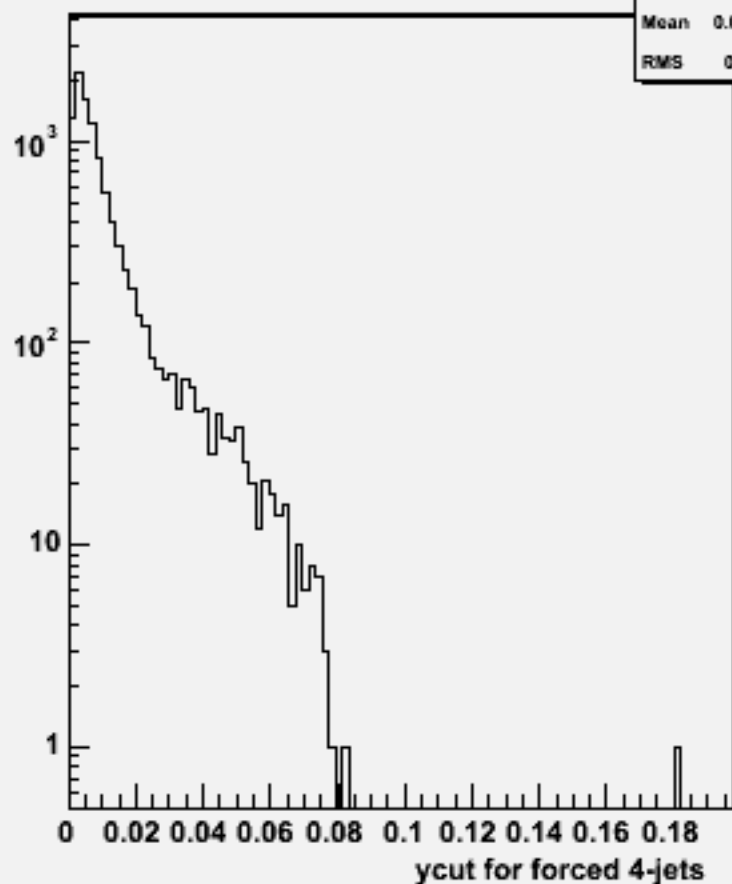
Ycut for 4-jets :w103681 ae1_e1n2e2sc_o
