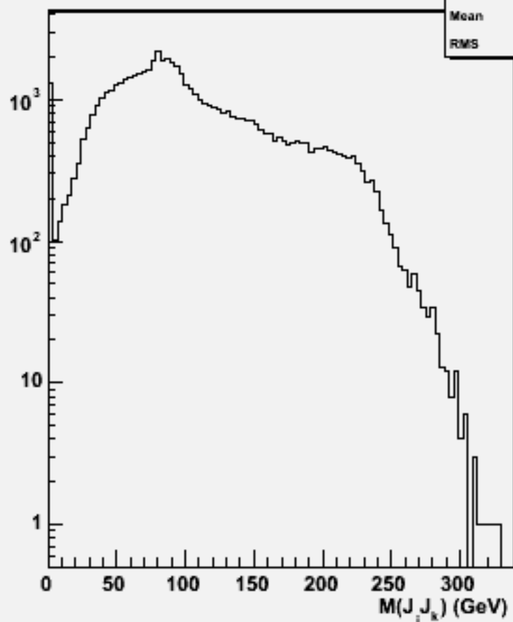
2jets mass(All comb)w103681 ae1_e1n2e2sc_o
