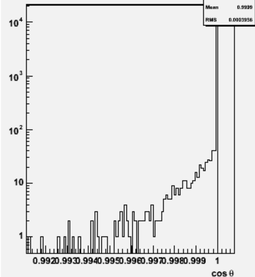
Jet cos theta (All jets)w103681 ae1_e1n2e2sc_o
